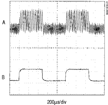
LINE-TRANSIENT RESPONSE
