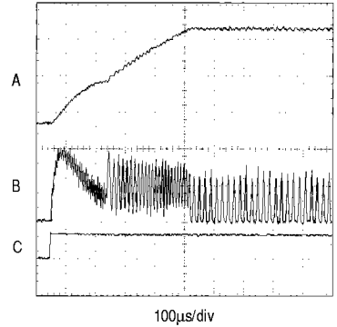
POWER-UP RESPONSE
