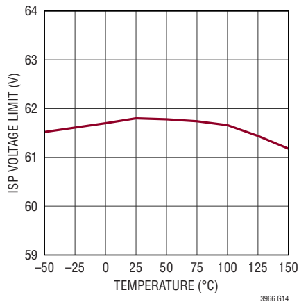
ISP Voltage Limit vs Temperature
