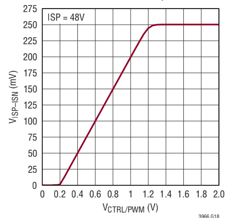
V_{ISP-ISN} vs ADIM V_{CTRL/PWM}
