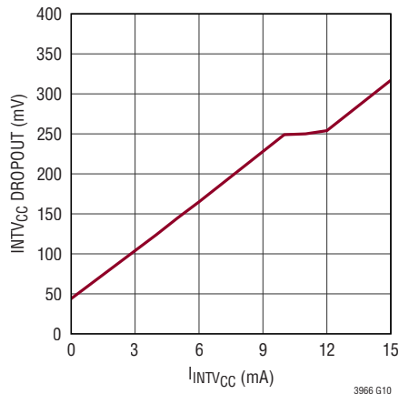
INTV CC Dropout vs Temperature Load
