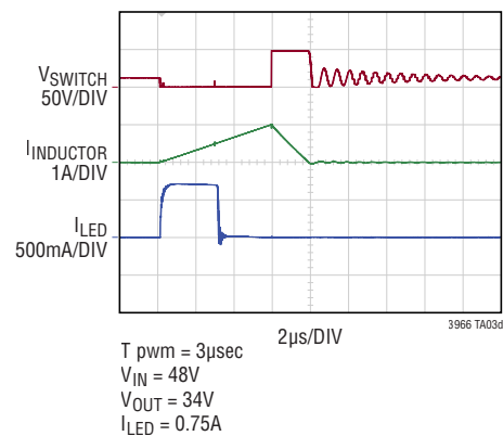
8192:1 Dimming
