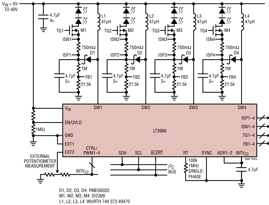
5V to 40V Buck-Boost Mode Driver for 4 Series 330mA LEDs
