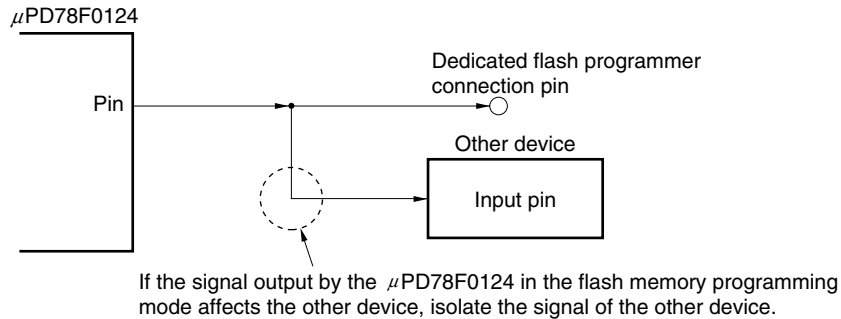
Figure 25-15. Malfunction of Other Device
