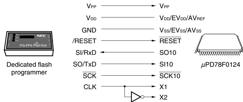
Figure 25-8. Communication with Dedicated Flash Programmer (CSI10)
