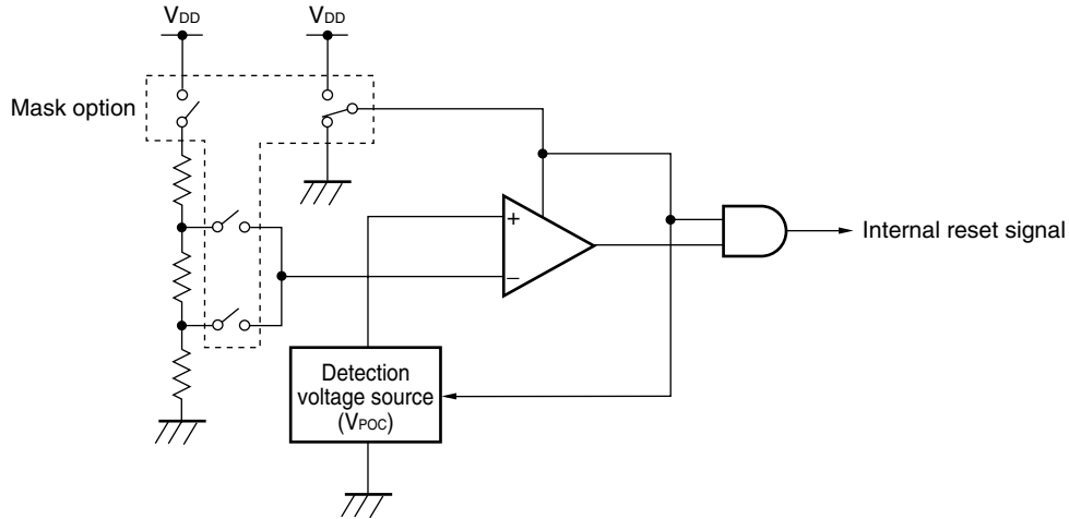
Figure 21-1. Block Diagram of Power-on-Clear Circuit
