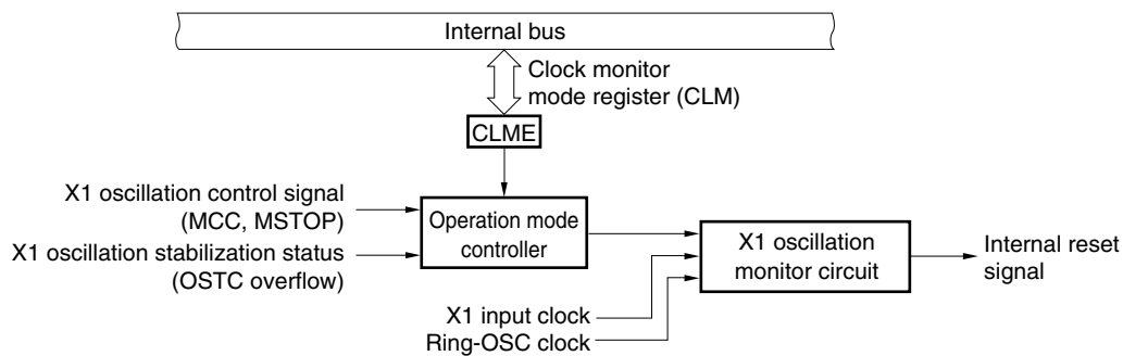
★ Figure 20-1. Block Diagram of Clock Monitor
