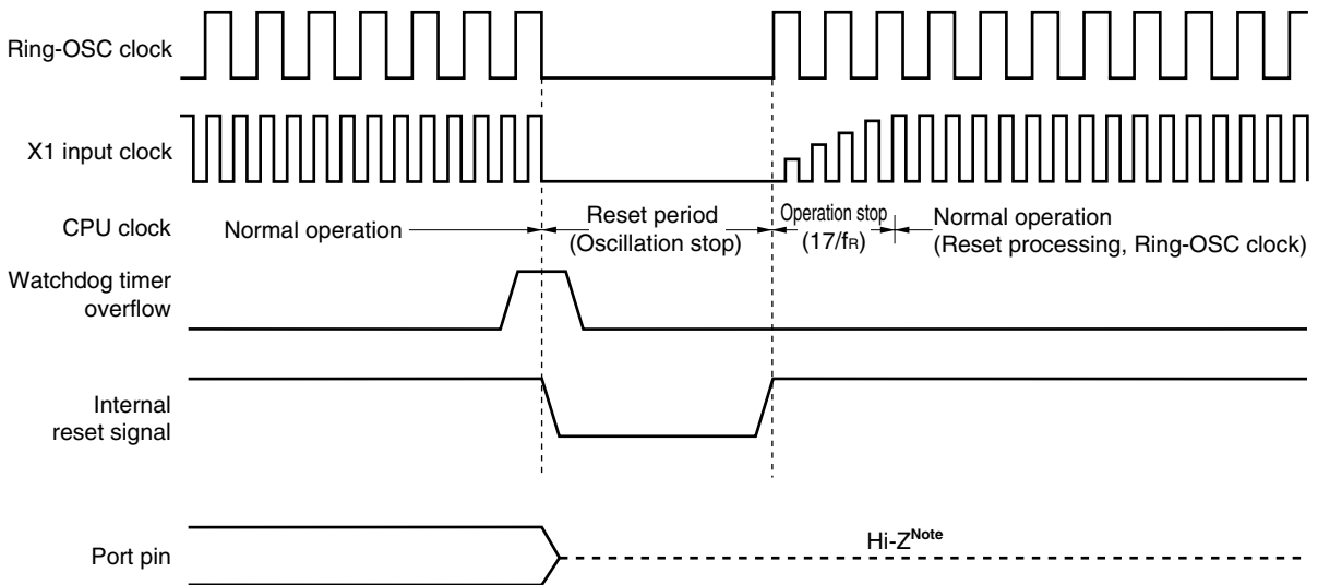
Figure 19-3. Timing of Reset Due to Watchdog Timer Overflow
