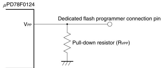
Figure 25-13. Example of Connection of V_{PP} Pin
