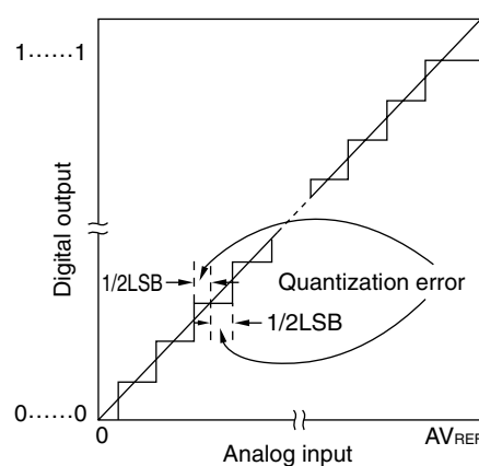
Figure 12-13. Quantization Error
