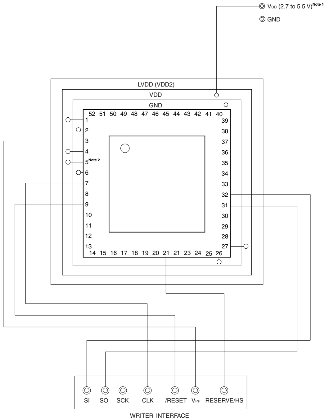
Figure 25-5. Example of Wiring Adapter for Flash Memory Writing in UART (UART0 + HS) Mode
