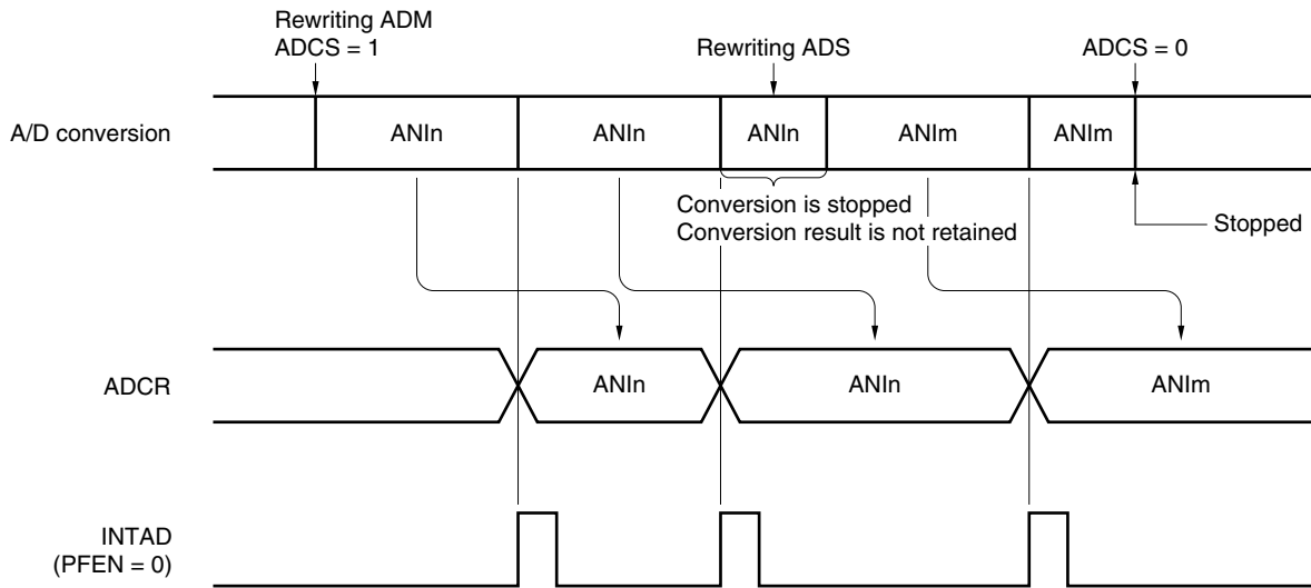
Figure 12-10. A/D Conversion Operation
