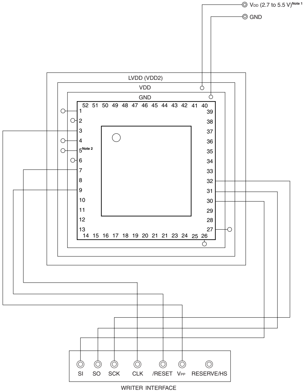
Figure 25-2. Example of Wiring Adapter for Flash Memory Writing in 3-Wire Serial I/O (CSI10) Mode
