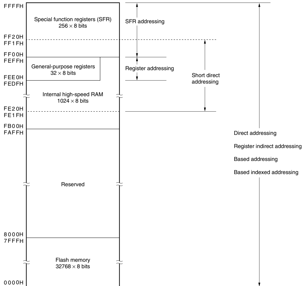
Figure 3-10. Correspondence Between Data Memory and Addressing ( \mu PD78F0124)
