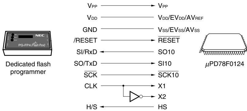
Figure 25-9. Communication with Dedicated Flash Programmer (CSI10 + HS)
