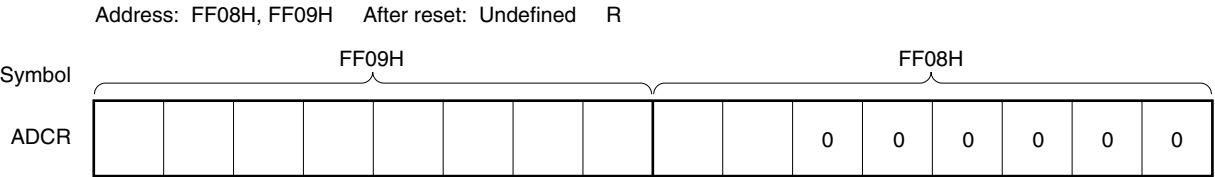
Figure 12-5. Format of A/D Conversion Result Register (ADCR)
