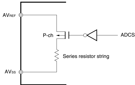
Figure 12-18. Circuit Configuration of Series Resistor String
