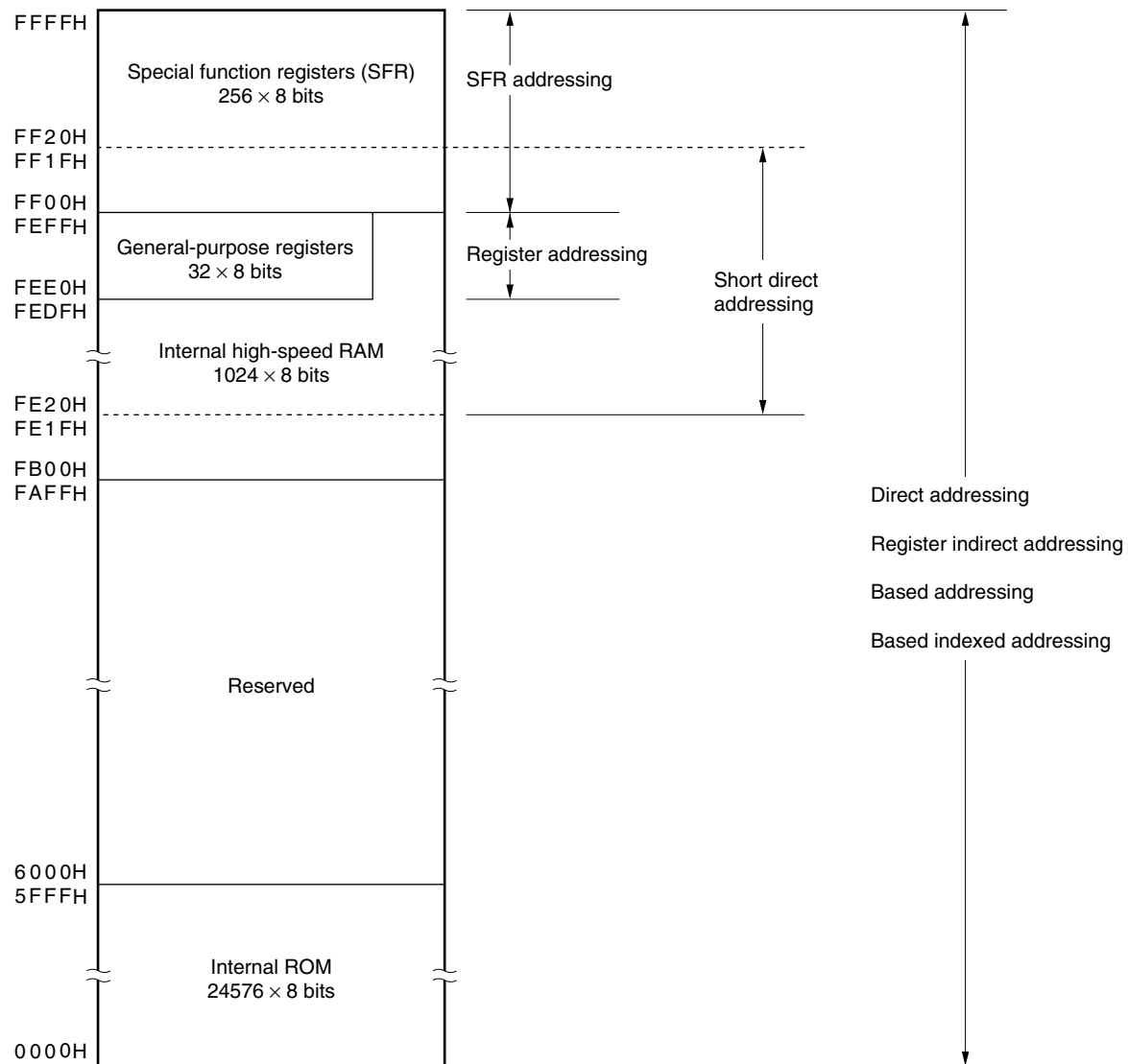
Figure 3-8. Correspondence Between Data Memory and Addressing ( \mu PD780123)
