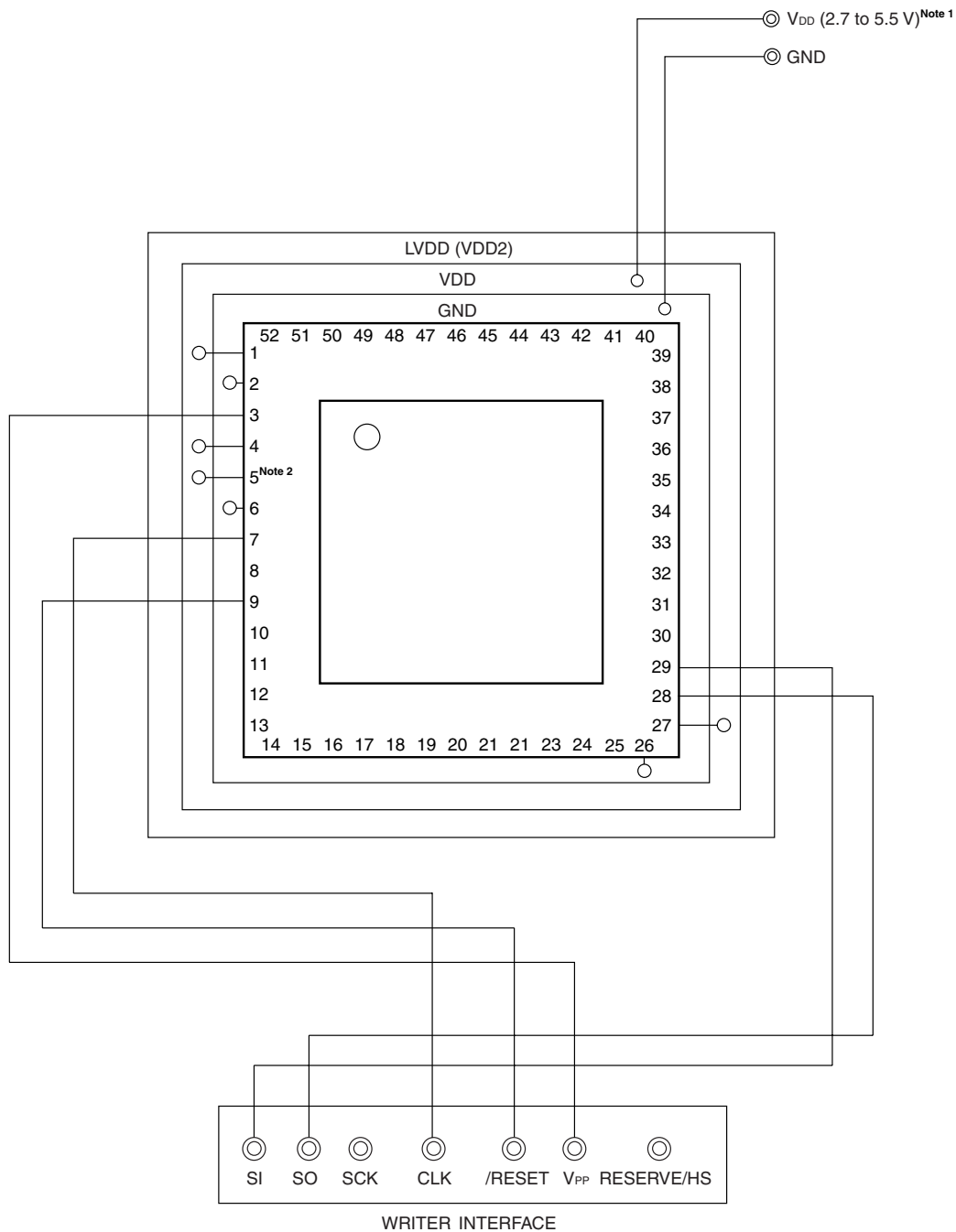
Figure 25-6. Example of Wiring Adapter for Flash Memory Writing in UART (UART6) Mode
