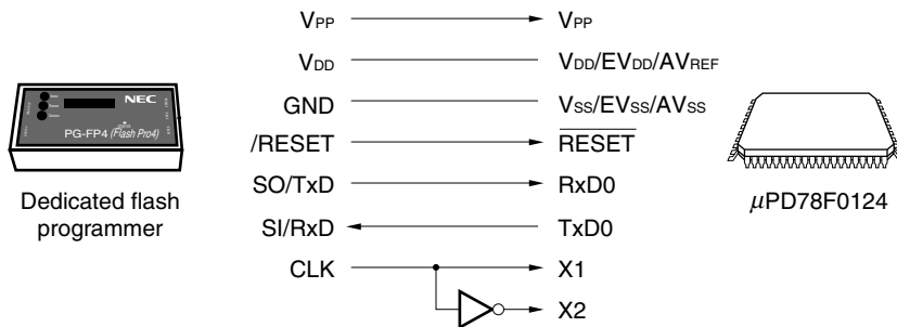
Figure 25-10. Communication with Dedicated Flash Programmer (UART0)
