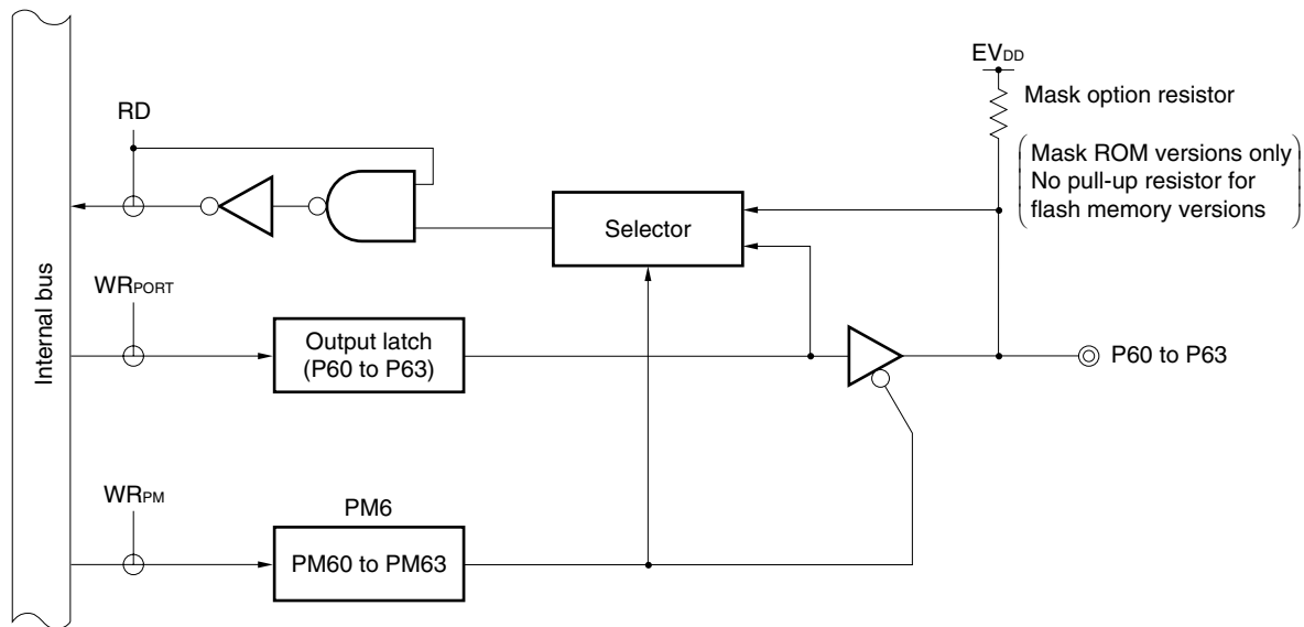
Figure 4-13. Block Diagram of P60 to P63
