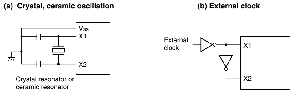
★ Figure 5-8. Examples of External Circuit of X1 Oscillator
