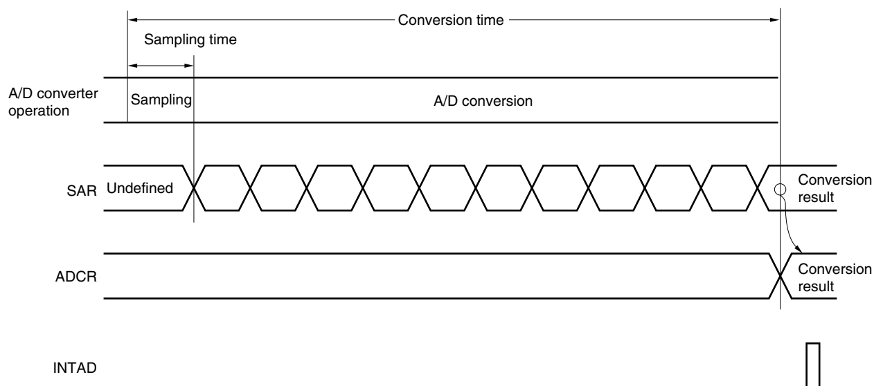
Figure 12-8. Basic Operation of A/D Converter
