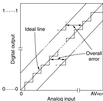
Figure 12-12. Overall Error
