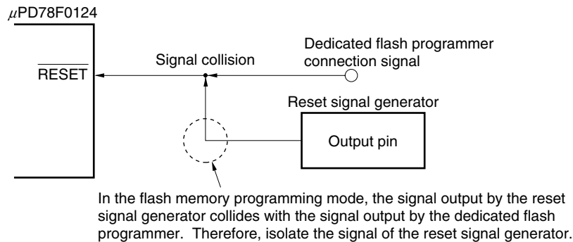
Figure 25-16. Signal Collision ( \overline{\text{RESET}} Pin)
