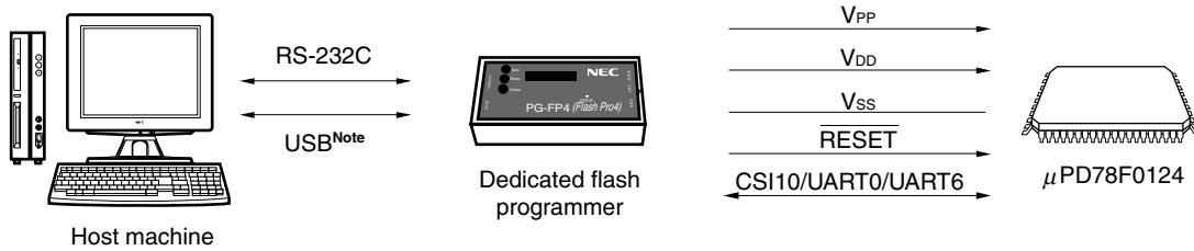
Figure 25-7. Environment for Writing Program to Flash Memory
