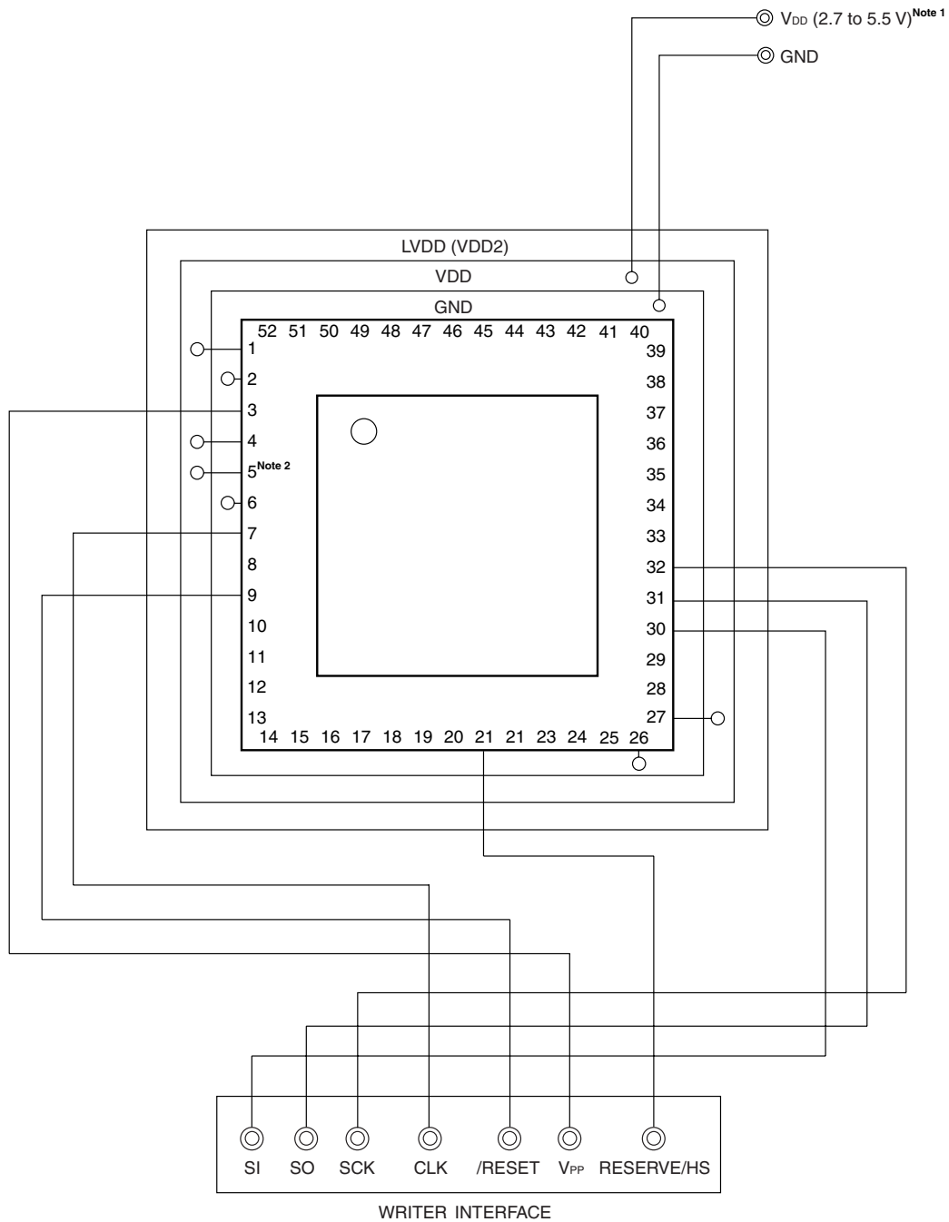
Figure 25-3. Example of Wiring Adapter for Flash Memory Writing in 3-Wire Serial I/O (CSI10 + HS) Mode
