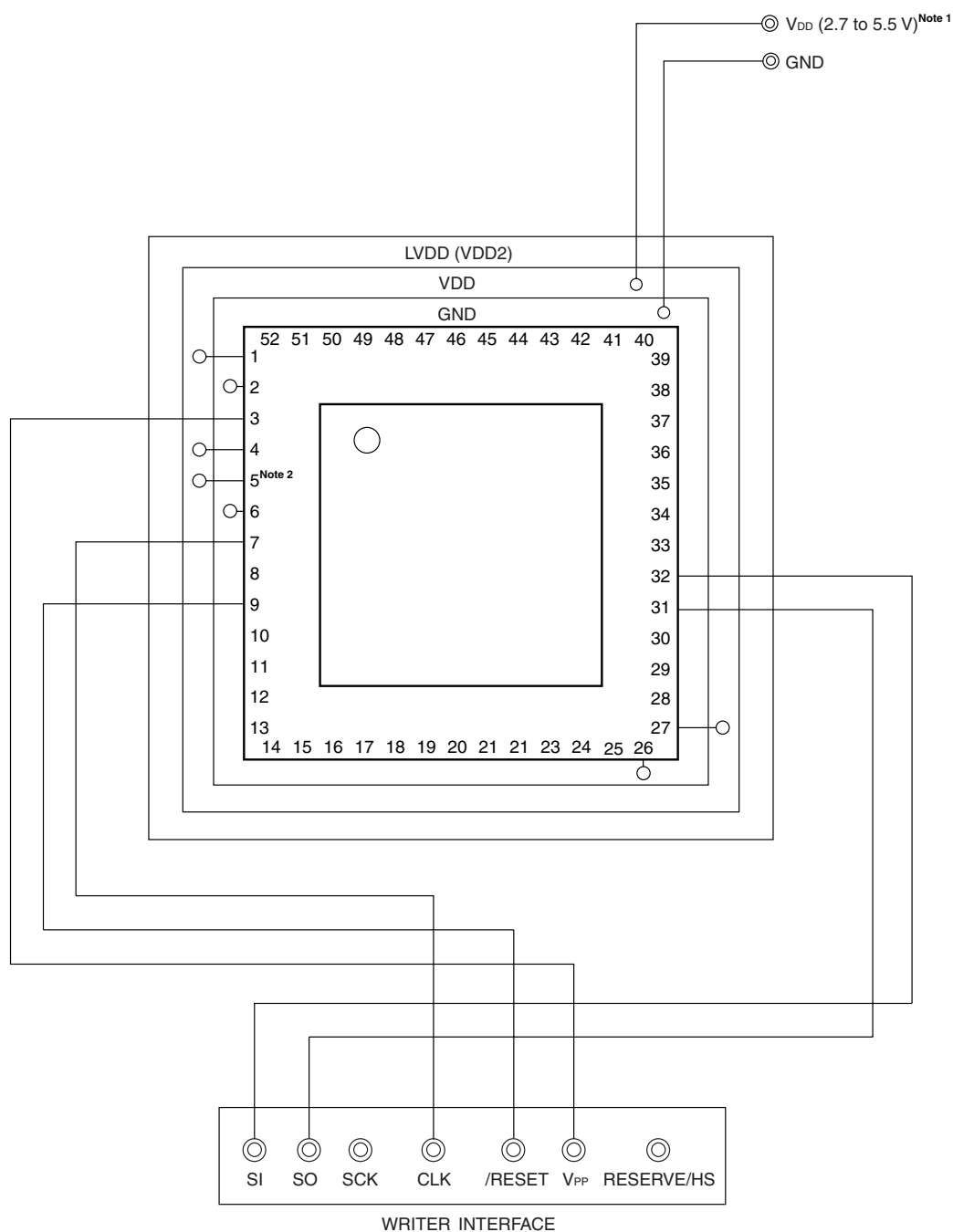
Figure 25-4. Example of Wiring Adapter for Flash Memory Writing in UART (UART0) Mode
