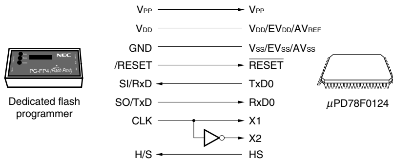
Figure 25-11. Communication with Dedicated Flash Programmer (UART0 + HS)
