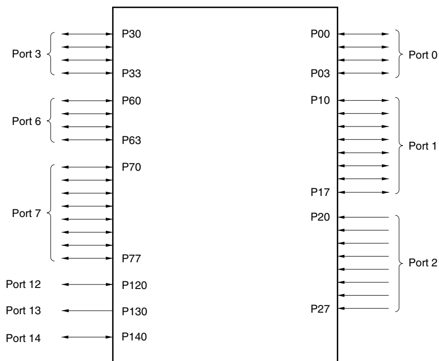
Figure 4-1. Port Types
