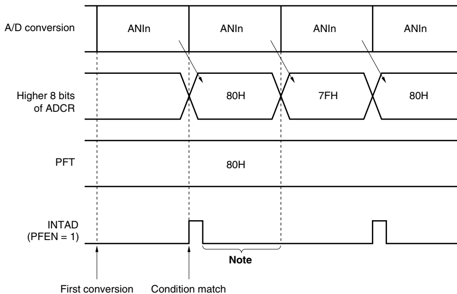
Figure 12-11. Power-Fail Detection (When PFEN = 1 and PFCM = 0)
