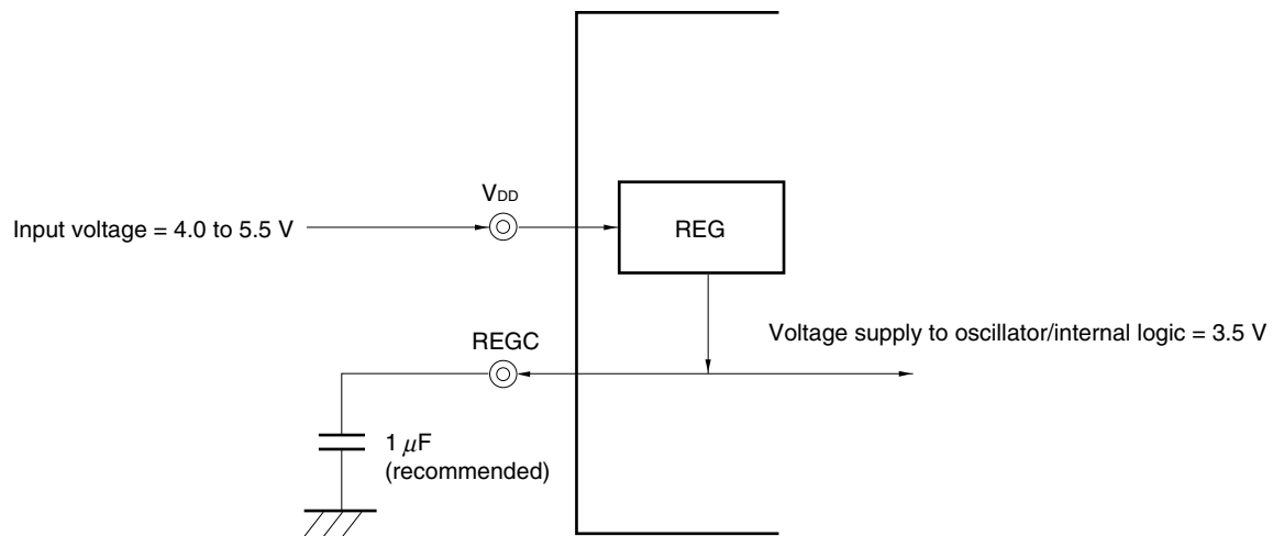
(b) When connecting REGC pin to V_{\text{SS}} via a capacitor
