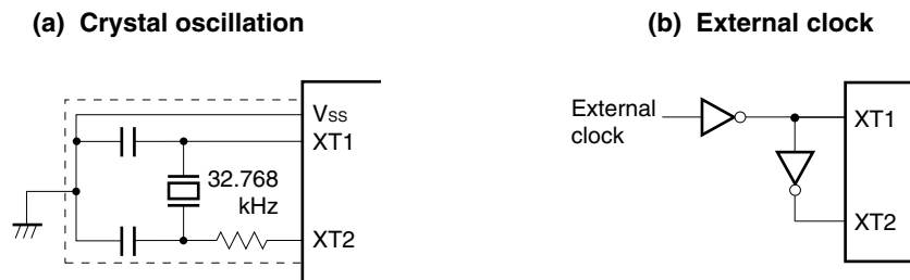
★ Figure 5-9. Examples of External Circuit of Subsystem Clock Oscillator
