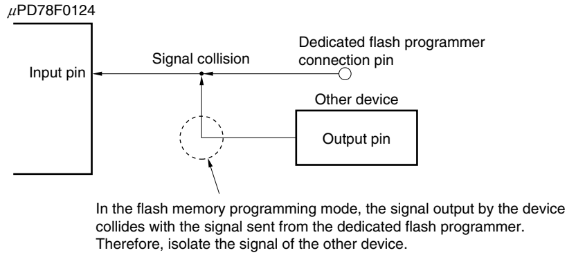
Figure 25-14. Signal Collision (Input Pin of Serial Interface)
