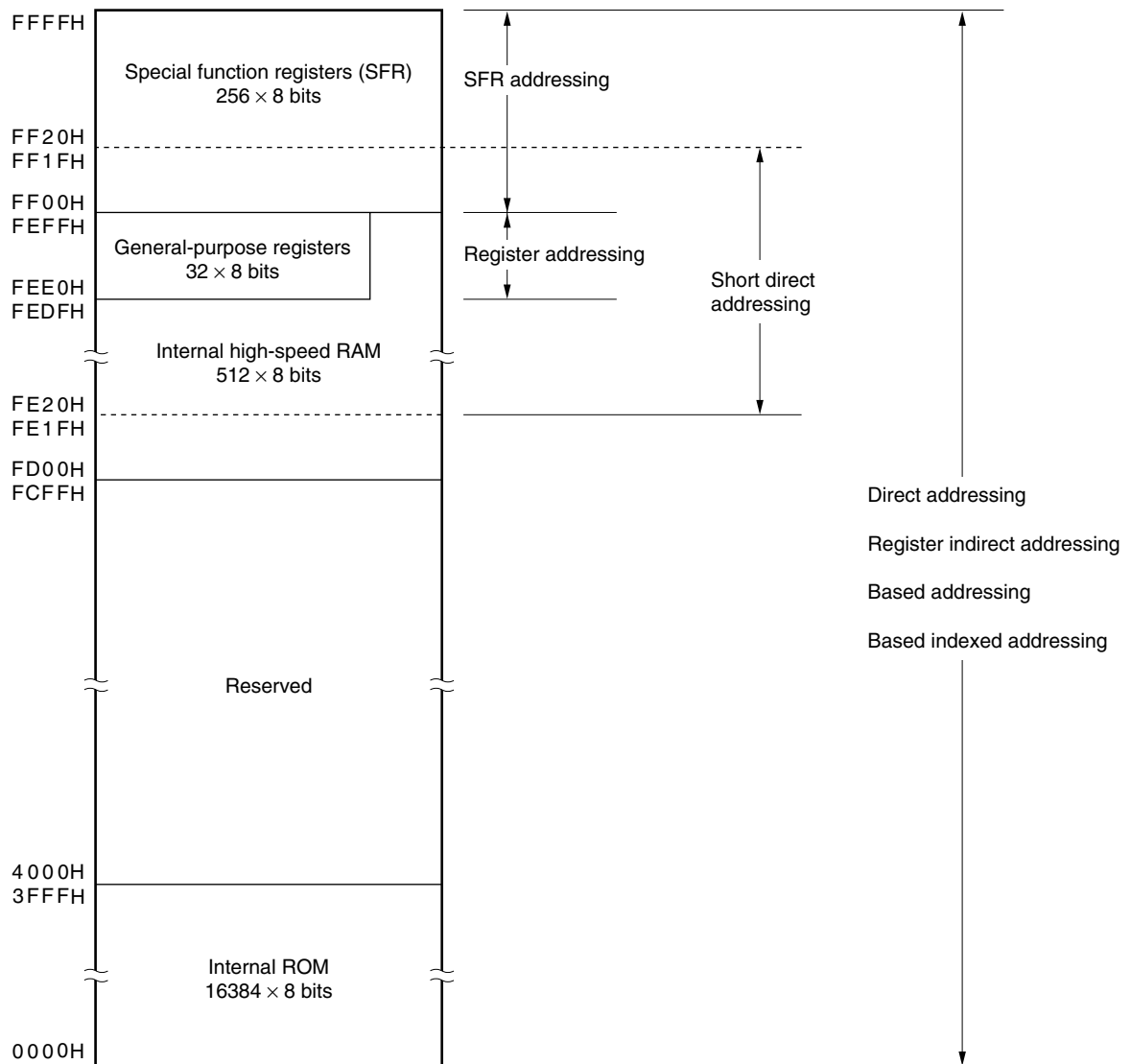
Figure 3-7. Correspondence Between Data Memory and Addressing ( \mu PD780122)
