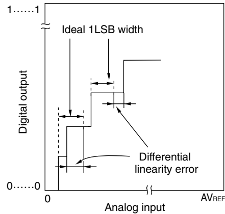
Figure 12-17. Differential Linearity Error
