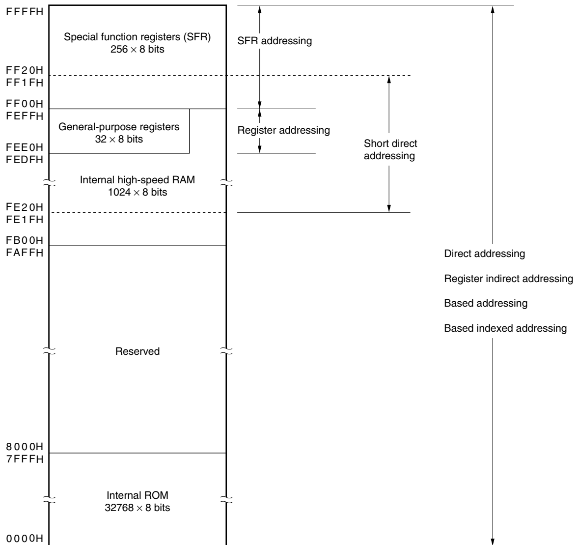
Figure 3-9. Correspondence Between Data Memory and Addressing ( \mu PD780124)
