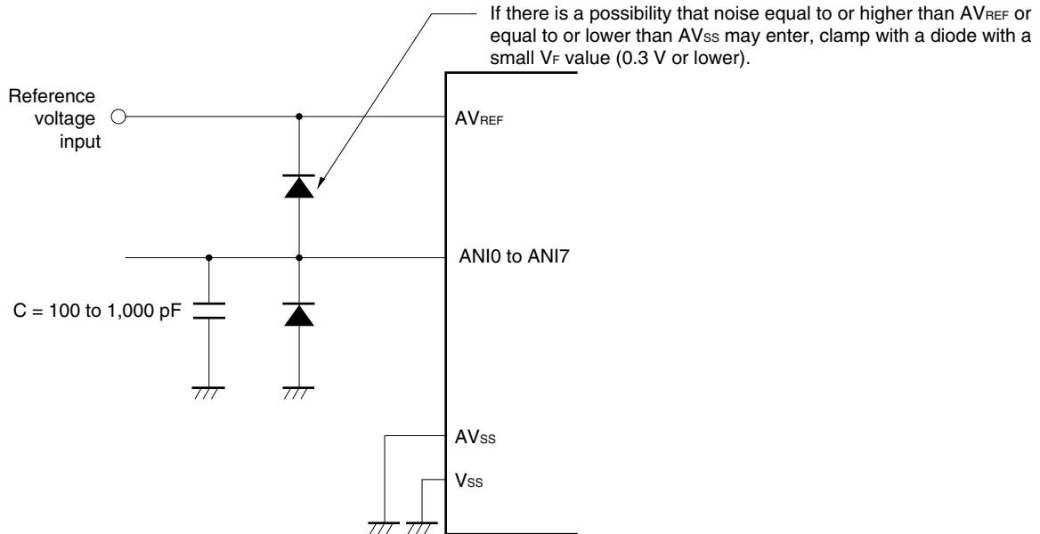
Figure 12-19. Analog Input Pin Connection
