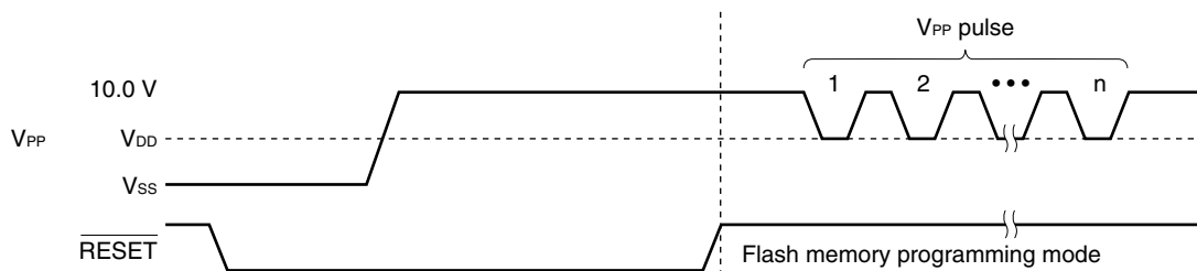
Figure 25-18. Flash Memory Programming Mode
