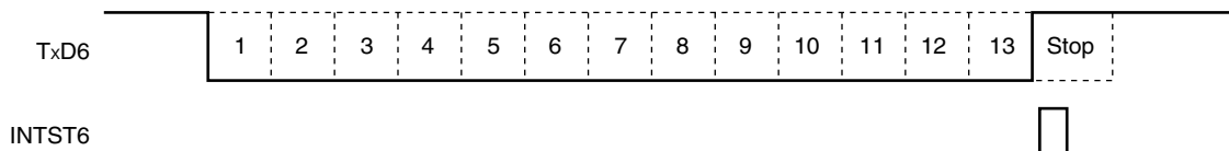
Figure 14-23. SBF Transmission
