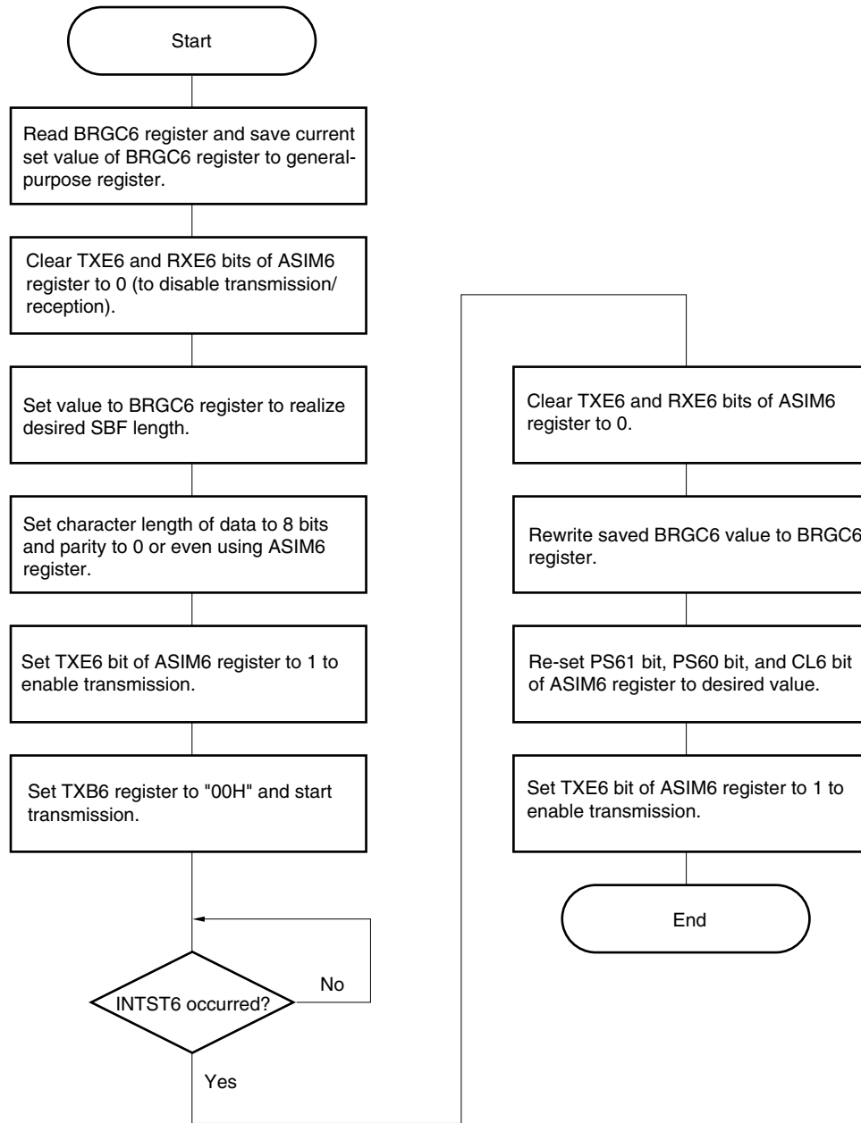
Figure 14-23. SBF Transmission
