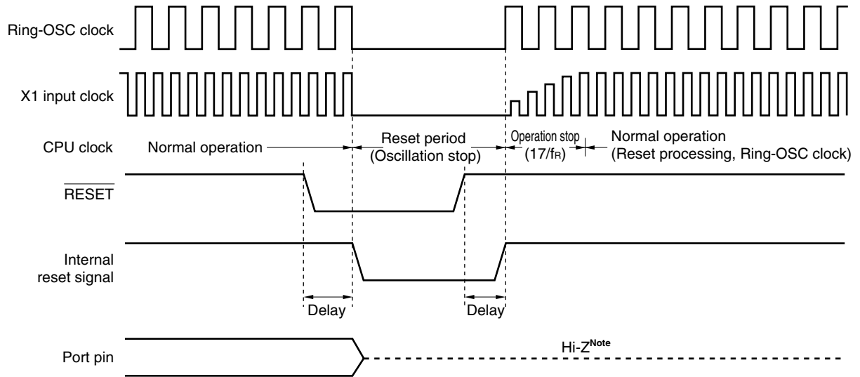
Figure 19-2. Timing of Reset by \overline{\text{RESET}} Input
