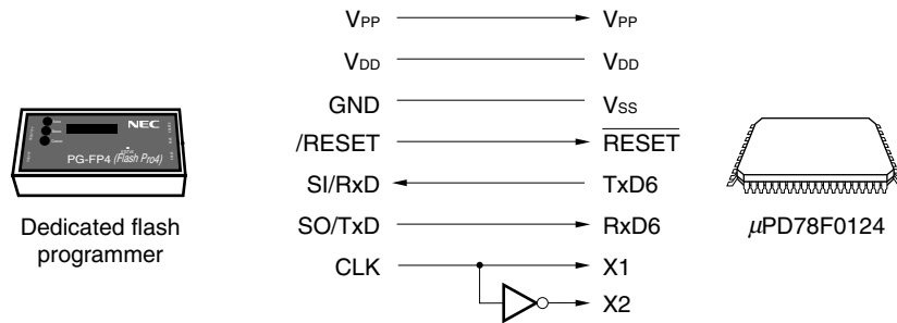
Figure 25-12. Communication with Dedicated Flash Programmer (UART6)
