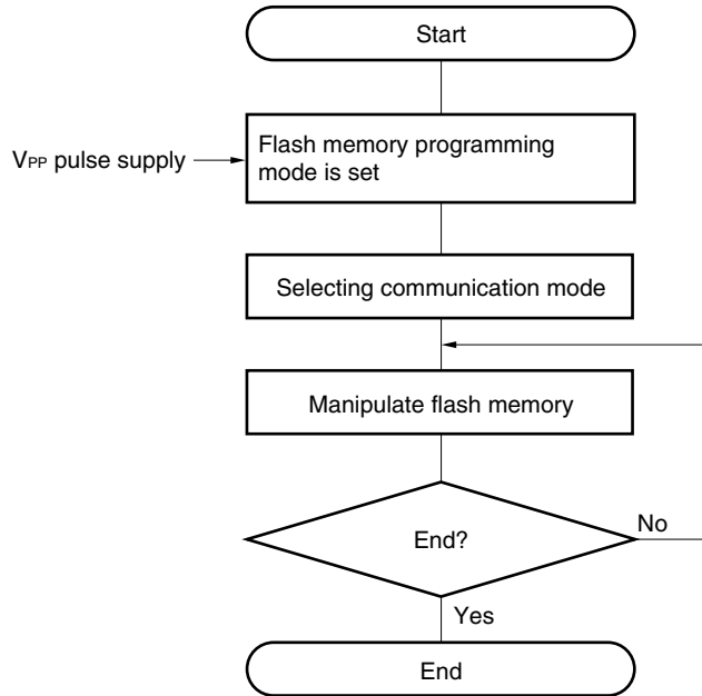
Figure 25-17. Flash Memory Manipulation Procedure
