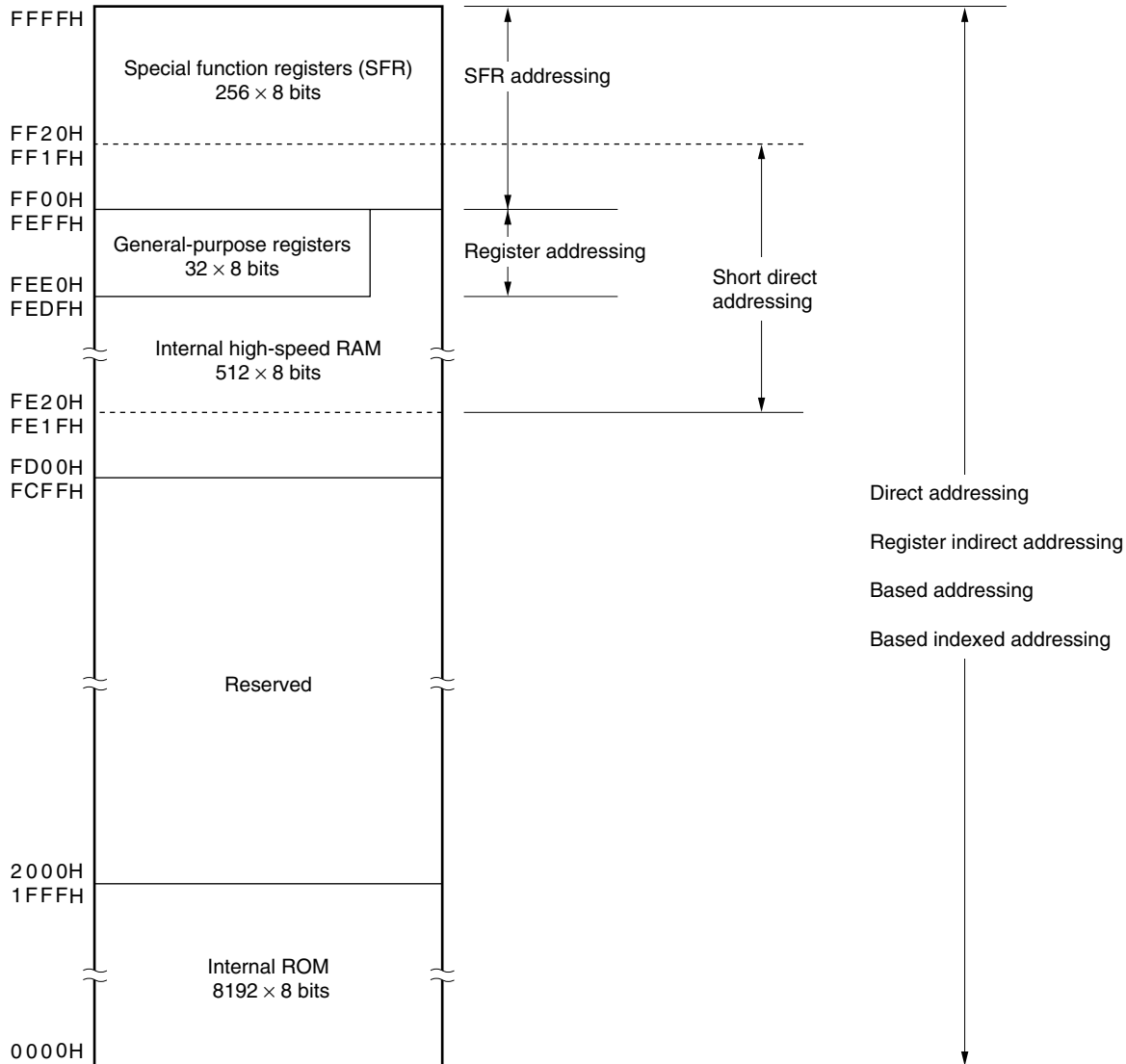
Figure 3-6. Correspondence Between Data Memory and Addressing ( \mu PD780121)
