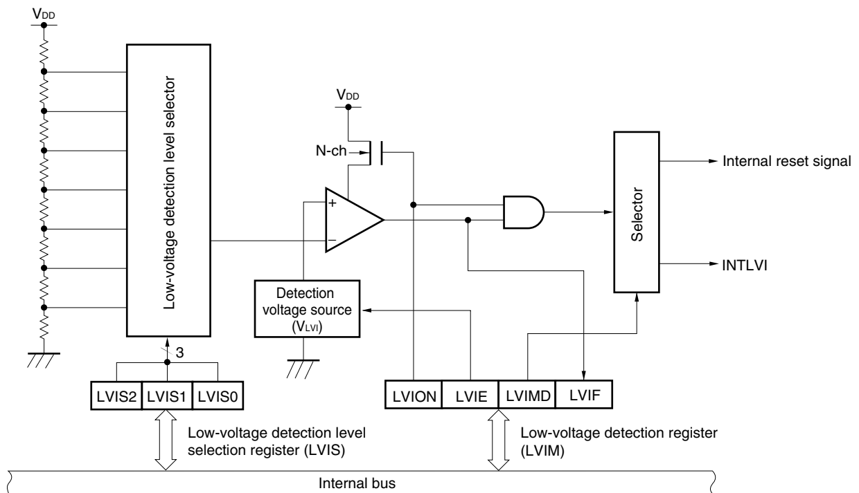
★ Figure 22-1. Block Diagram of Low-Voltage Detector
