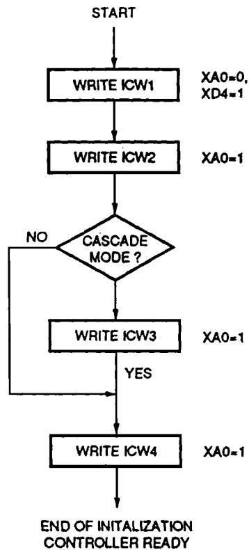
Figure 8. Initialization Sequence
