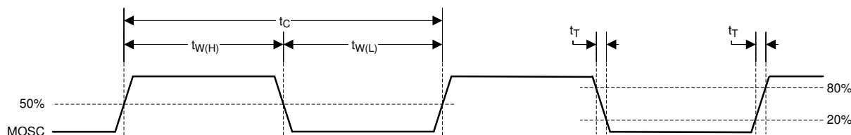
Figure 6-5. System Oscillators
