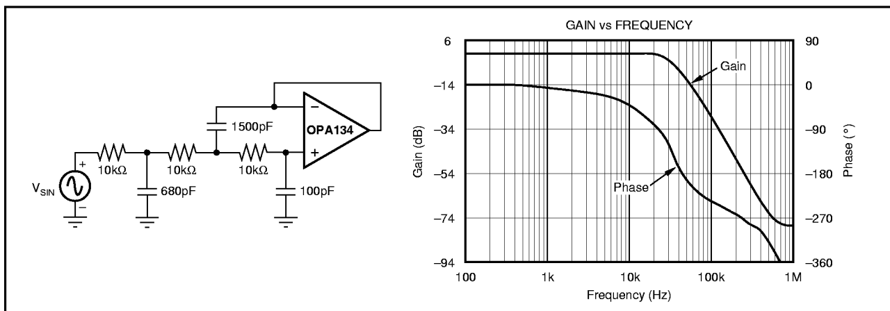
FIGURE 9. 3rd-Order LPF.
