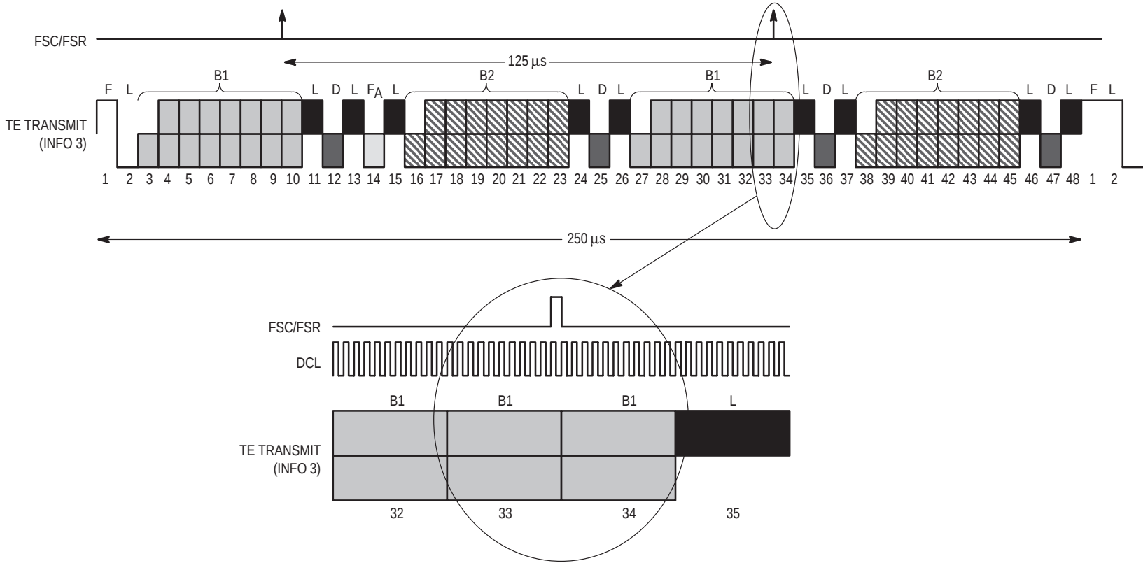
Figure 4-3. Phase Relationship of TE Transmit Signal
