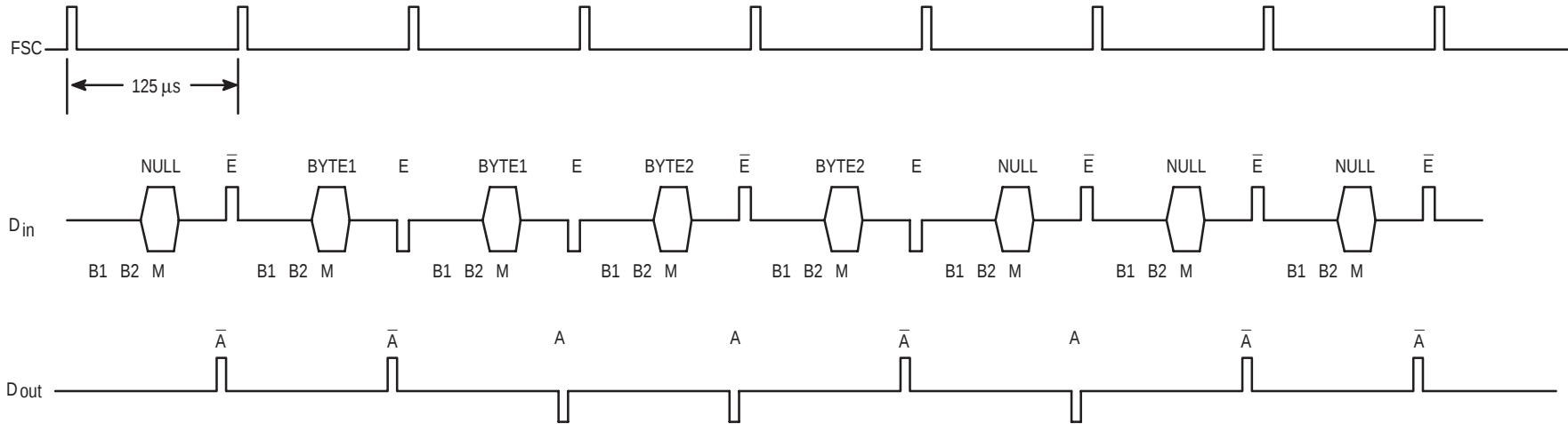
Figure 6-3. Monitor Channel Access Protocol
