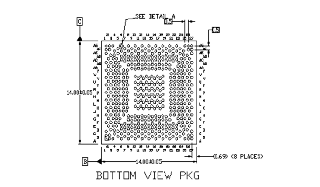
Figure 7-5. PCH (Bottom View)
