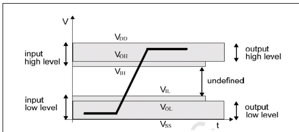
Figure 4-2. MMC Bus Signal Levels
