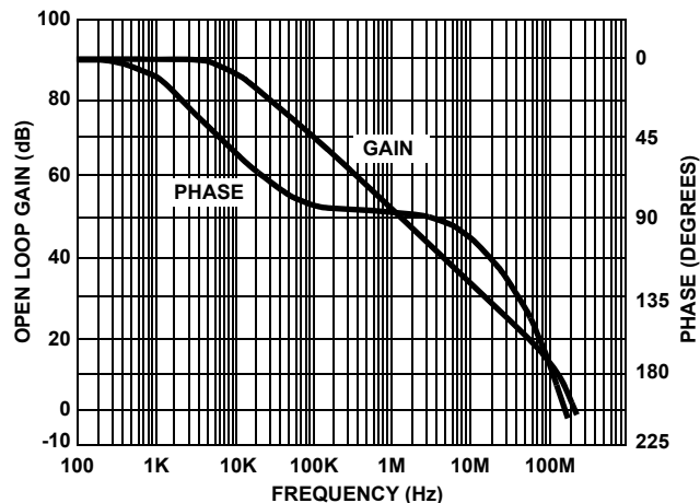
FIGURE 16. OPEN LOOP GAIN/PHASE vs FREQUENCY
