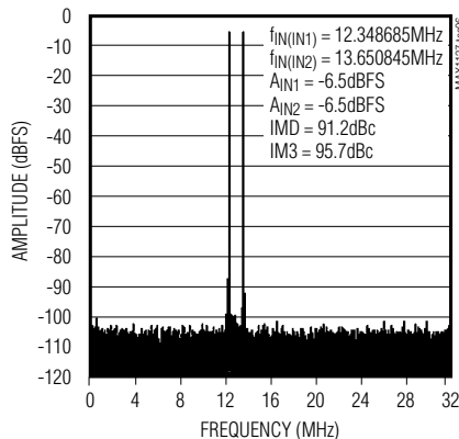
TWO-TONE INTERMODULATION DISTORTION (32,768-POINT DATA RECORD)
