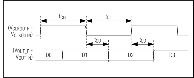
Figure 5. Serialized Output Detailed Timing Diagram
