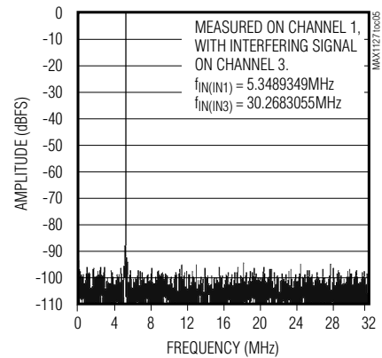
CROSSTALK (4096-POINT DATA RECORD)
