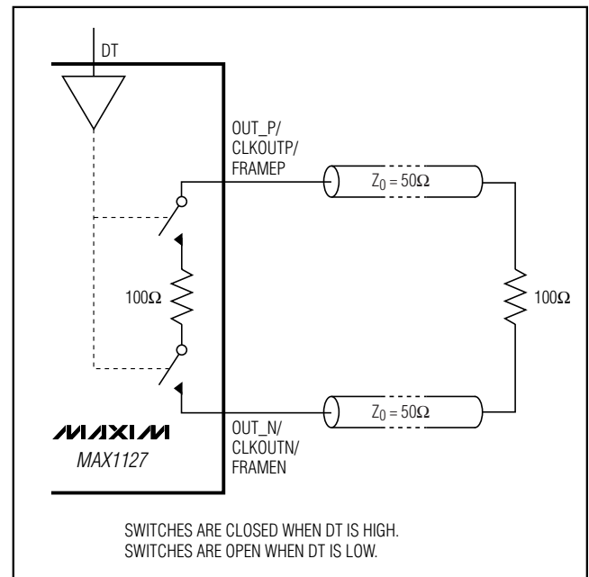
Figure 8. Double Termination
