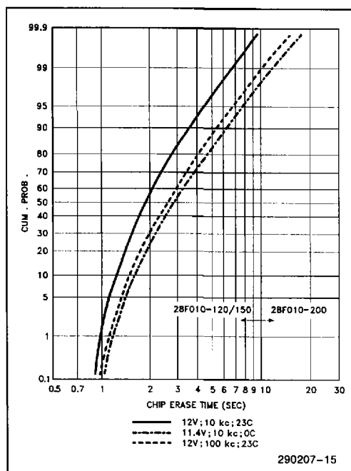
Figure 9. Typical Erase Capability
