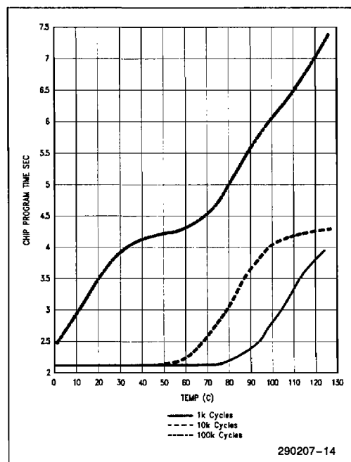
Figure 8. Typical Program Time at 12V
