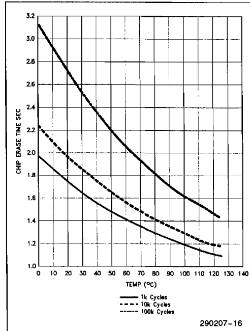
Figure 10. Typical Erase Time at 12V
