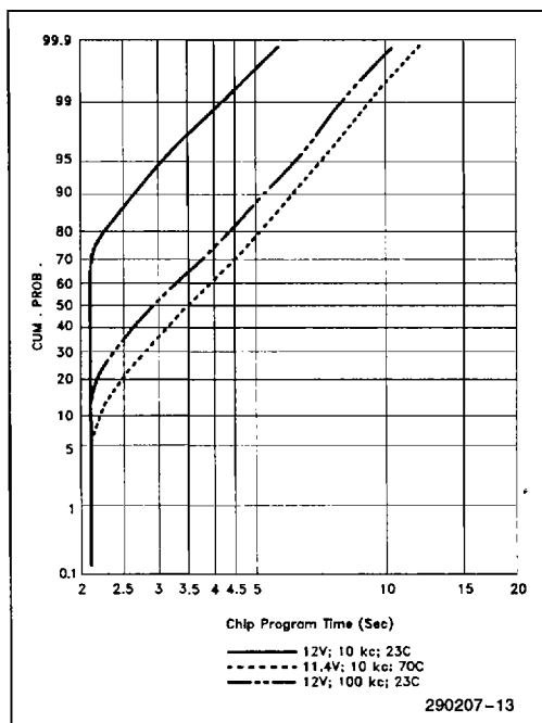
Figure 7. Typical Programming Capability
