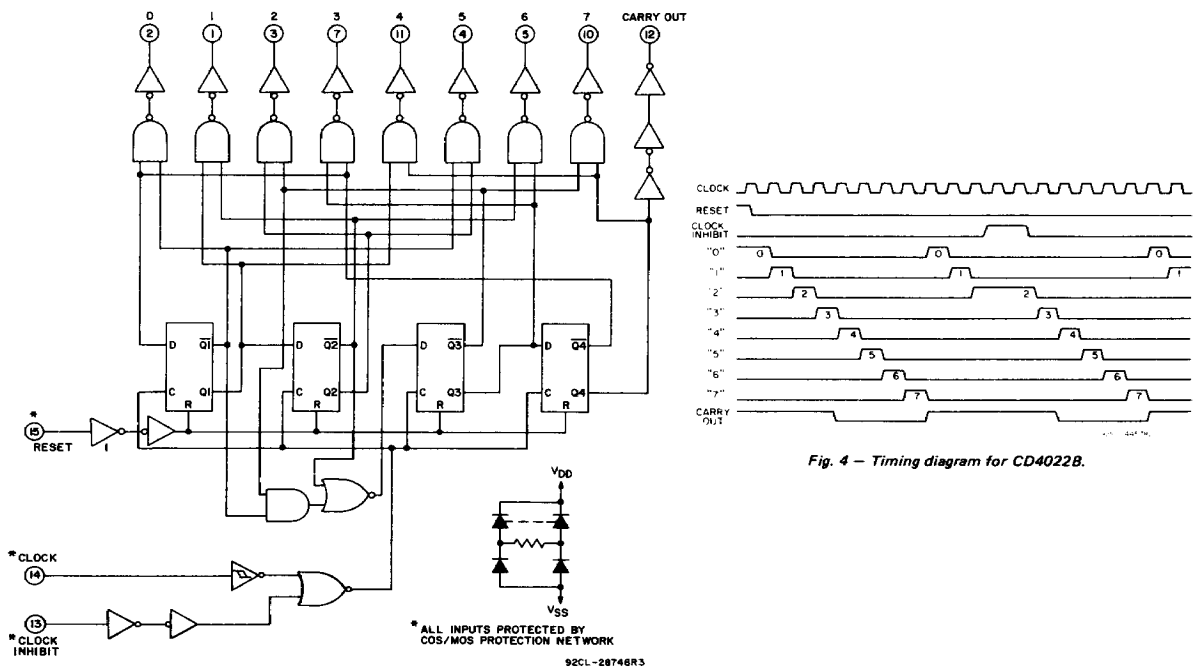
Fig. 3 - Logic diagram for CD4022B.
