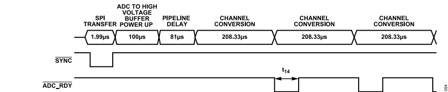
Figure 48. Single Measurement, Continuous Conversions Timing Diagram
