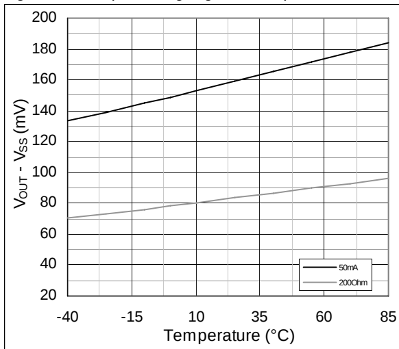
Figure 13. Output Swing High vs. Temp.; V_{DD} = 5.5V
