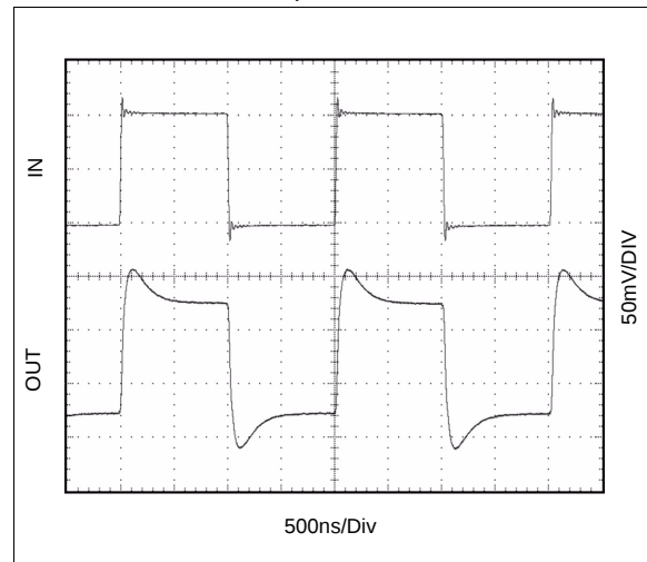
Figure 18. Transient Response; V_{IN} = 100\text{mV} , C_{LOAD} = 100\text{pF}
