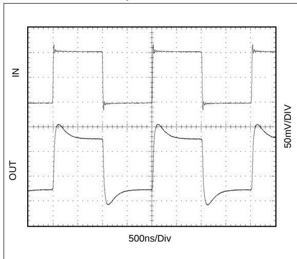
Figure 17. Transient Response; V_{IN} = 100\text{mV} , C_{LOAD} = 10\text{pF}
