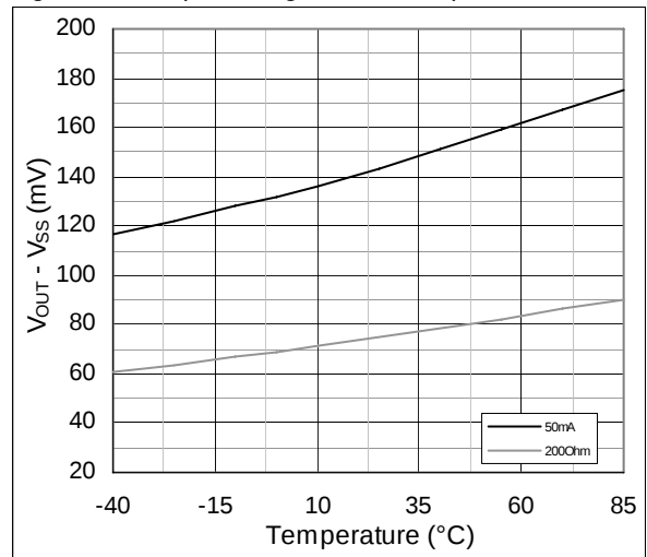
Figure 14. Output Swing Low vs. Temp.; V_{DD} = 5.5V
