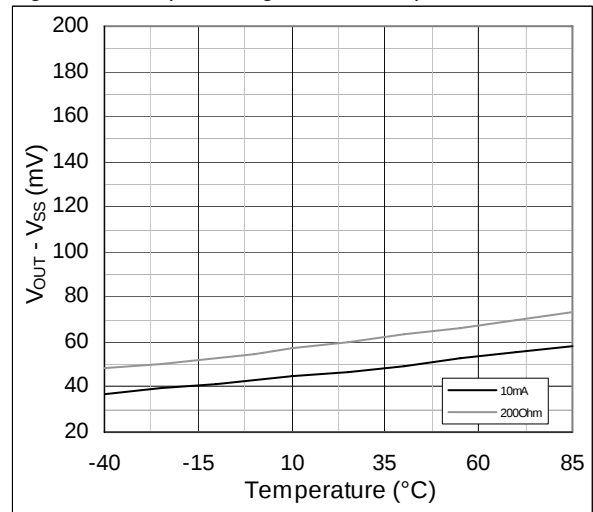
Figure 12. Output Swing Low vs. Temp.; V_{DD} = 2.7V
