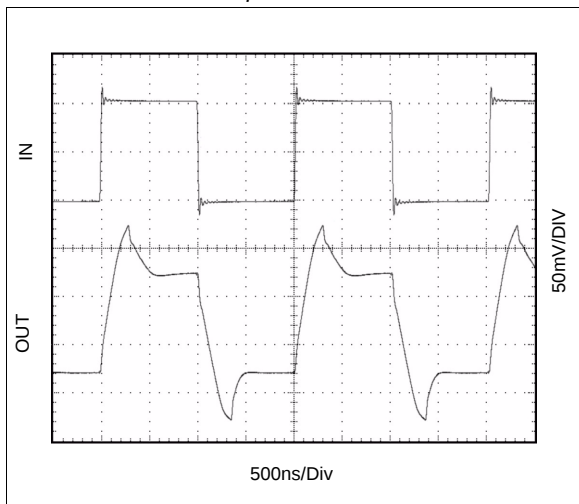
Figure 19. Transient Response; V_{IN} = 1\text{V} , C_{LOAD} = 10\text{pF}
