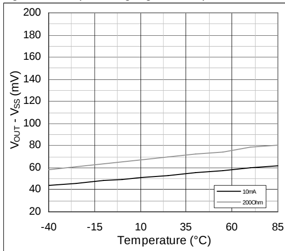
Figure 11. Output Swing High vs. Temp.; V_{DD} = 2.7V
