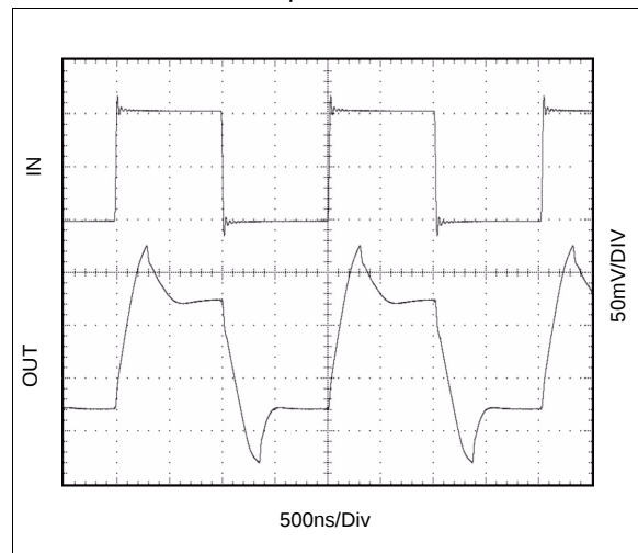
Figure 20. Transient Response; V_{IN} = 1\text{V} , C_{LOAD} = 100\text{pF}
