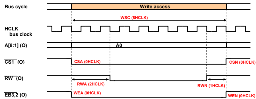
Fig. 5-3 iMX21 bus cycle waveform
