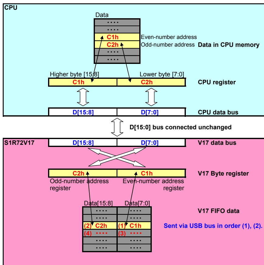
Fig. 3-3 Access to FIFO registers (big-endian CPU)
