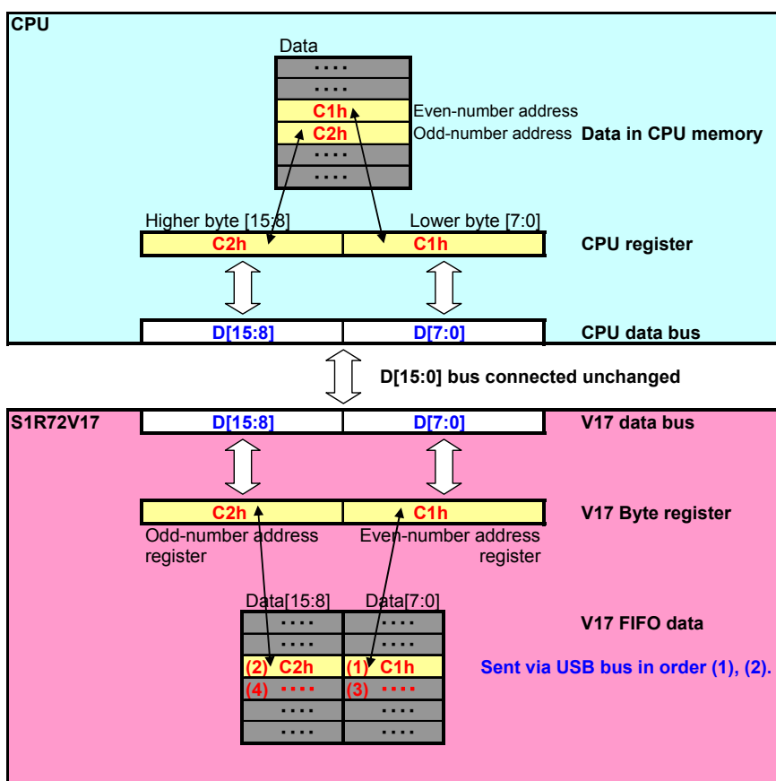
Fig. 3-6 Access to FIFO registers (little-endian CPU)
