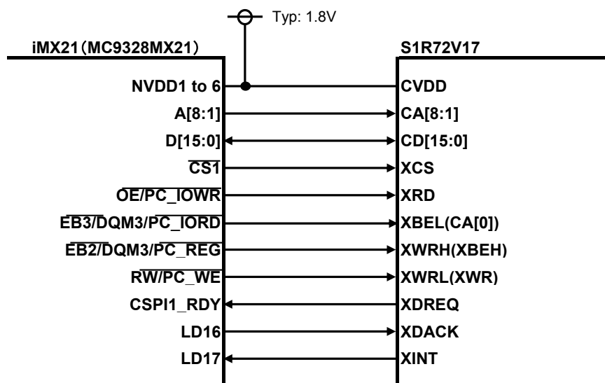
Fig. 5-1 Connection example with iMX21
