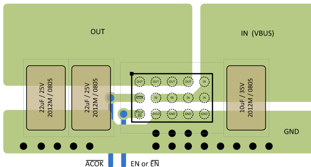
Figure 8. Recommended PCB Layout
