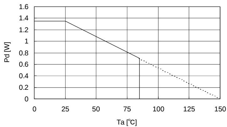
Fig.71 Thermal Derating Curve
