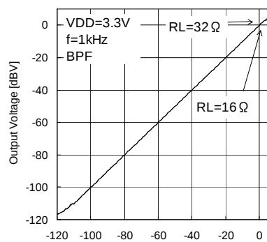
Fig.41 Output Voltage vs. Input Voltage (VDD=3.3V)
