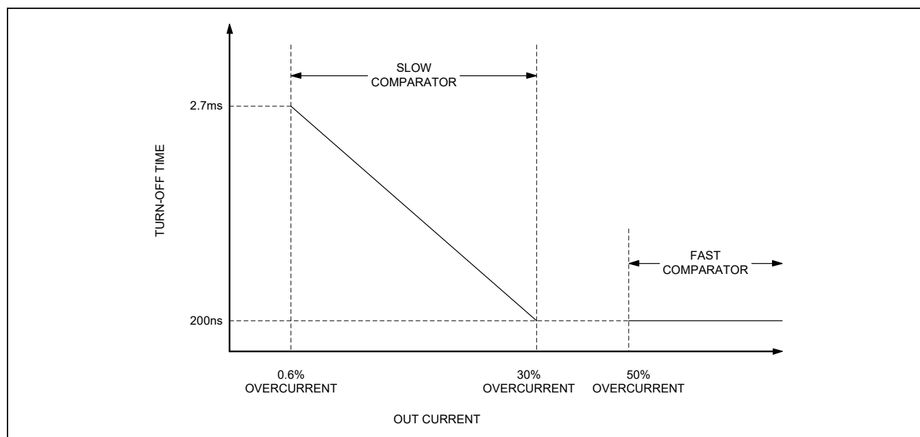
Figure 3. VariableSpeed/BiLevel Response
