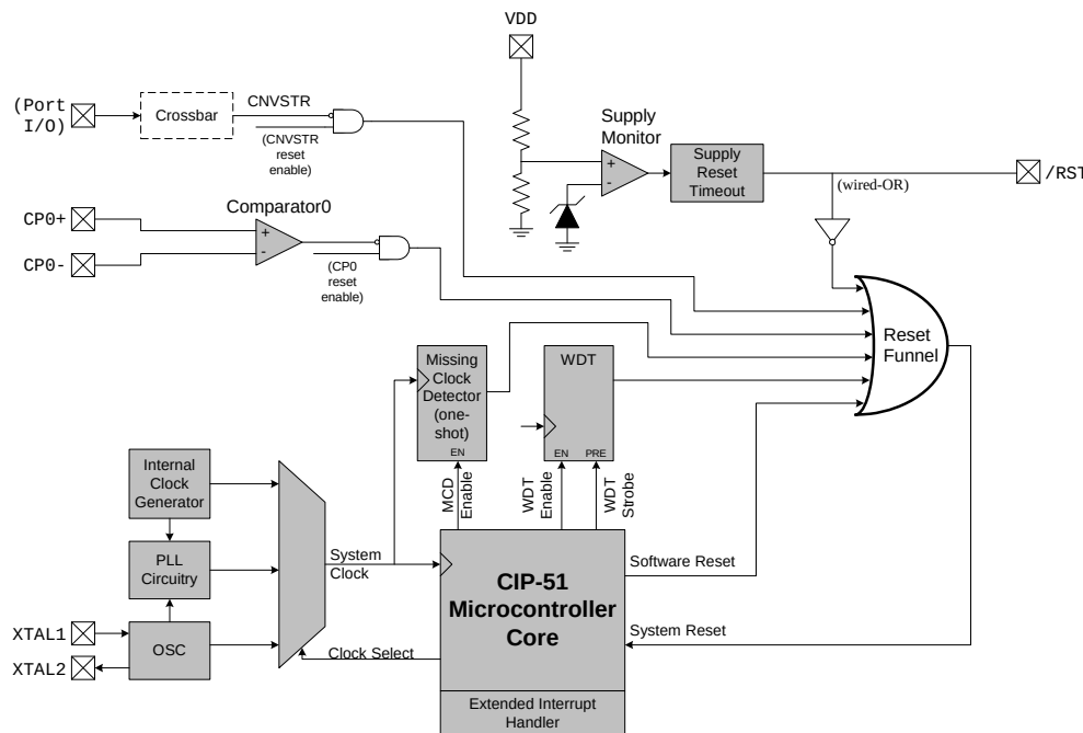
Figure 13.1. Reset Sources
