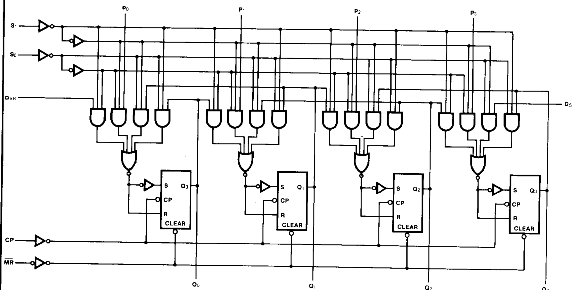
LOGIC DIAGRAM
