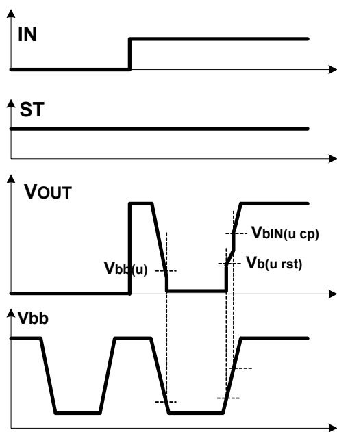
Figure 5a. Undervoltage
