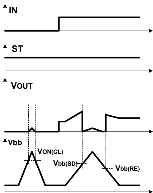
Figure 6. Overvoltage
