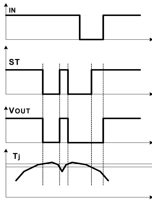
Figure 7. Over temperature
