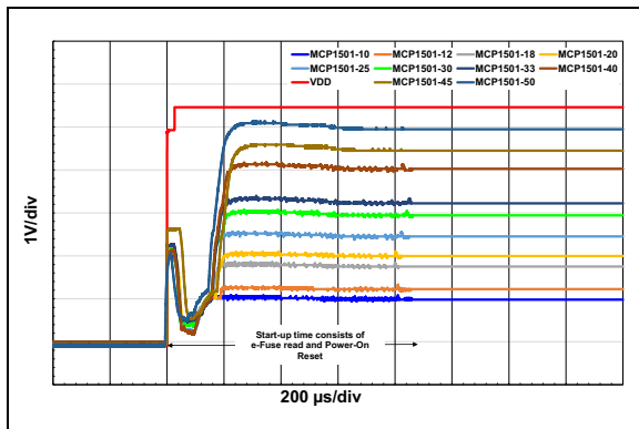
FIGURE 3-20: Fast Ramp Start-Up at 25°C for All Options.
