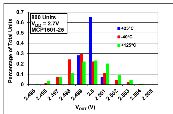
FIGURE 3-18: MCP1501 Output Voltage Histogram, V_{DD} = 2.7V .
