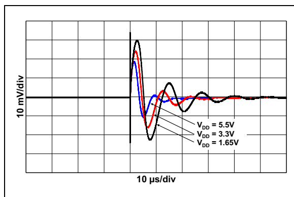
FIGURE 3-32: MCP1501-10 Transient Response vs. V_{DD} , C_L = 4.7nF .
