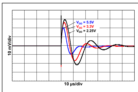
FIGURE 3-33: MCP1501-20 Transient Response vs. V_{DD} , C_L = 4.7 nF .
