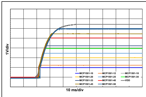
FIGURE 3-21: Slow Ramp Start-Up at 25°C for All Options.
