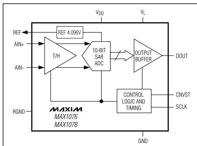
Figure 3. Functional Diagram
