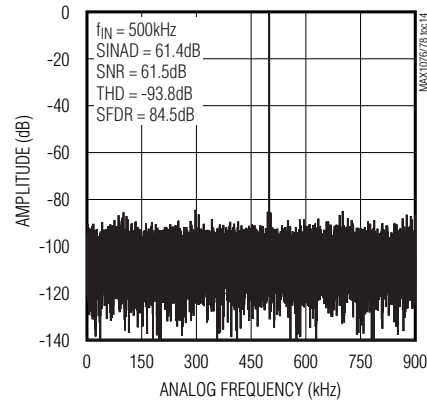
FFT PLOT (MAX1078)
