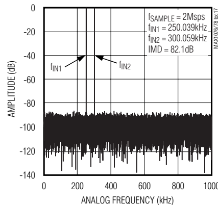
TWO-TONE IMD PLOT (MAX1078)
