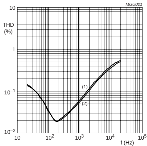
a. V_{CC} = 9 \text{ V} ; R_L = 16 \Omega ; P_o = 0.1 \text{ W} .
