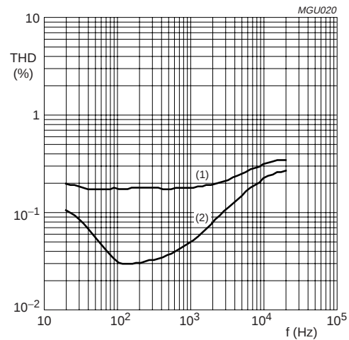
b. V_{CC} = 9 \text{ V} ; R_L = 16 \Omega ; P_o = 0.5 \text{ W} .
