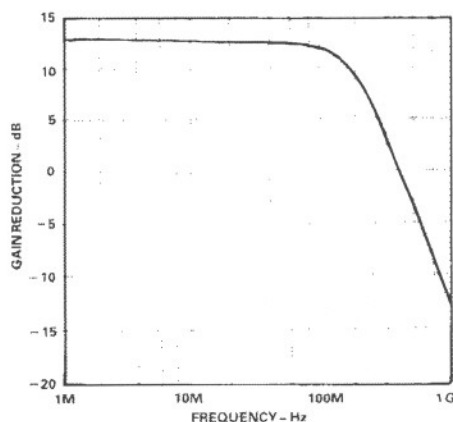
Figure 10. X4 Buffer Frequency Response (100 \Omega in Series with 1 \mu F Load)
