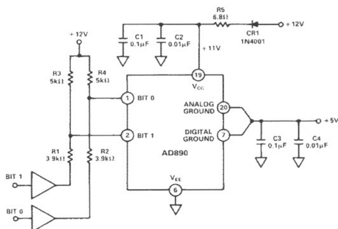
Figure 12. AD890 Connection for +5V, +12V Operation
