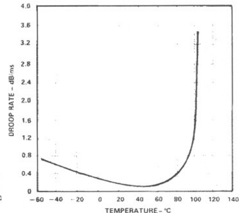
Figure 9. Hold-Mode Droop Rate vs. Temperature
