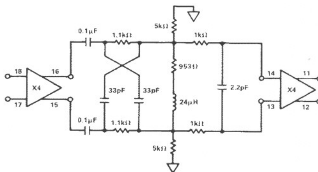
Figure 14. RLC Equalizer
