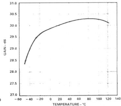
Figure 3. VGA Gain vs. Temperature
