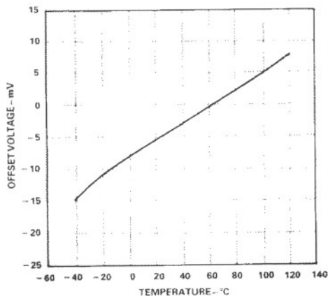
Figure 2. Rectifier Offset vs. Temperature
