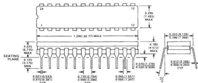
24-Pin Cerdip Package
