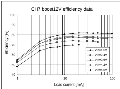
Fig.12 CH7 12V boost efficiency-Io
