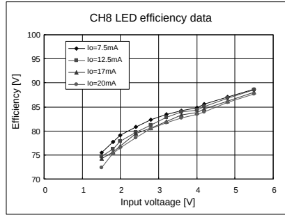
Fig.13 CH8 LED boost efficiency-Io
