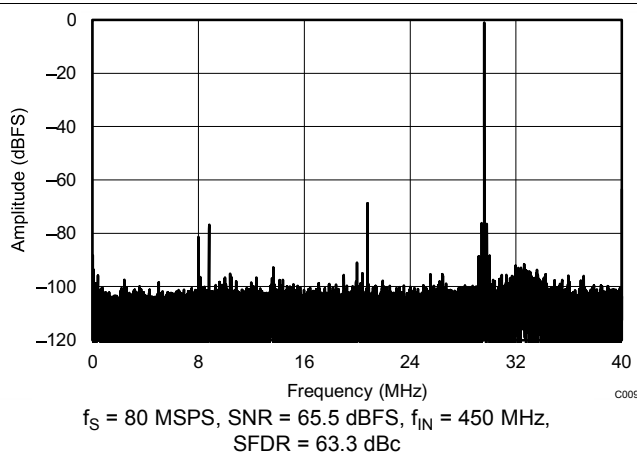
Figure 75. FFT for 450-MHz Input Signal (Dither On)
