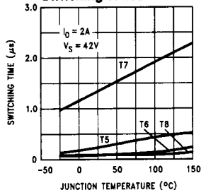
Sink Current Switching Times
