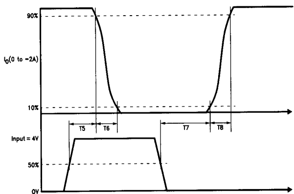
FIGURE 3(b). Sink Current Switching Time Definitions
