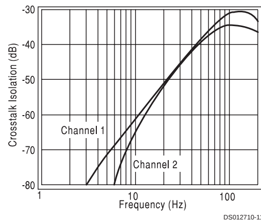
Channel-to-Channel Crosstalk
