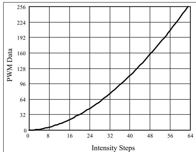
Figure 28 Gamma Correction (64 Steps)
