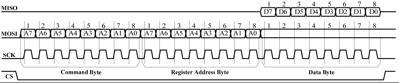
Figure 9 SPI Reading from IS31FL3747 (Typical)
