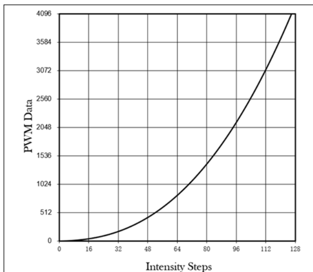
Figure 29 Gamma Correction (128 Steps)
