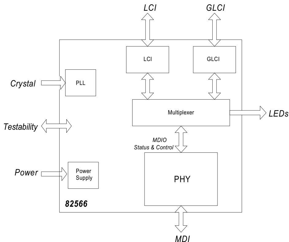
Figure 1. 82566 Block Diagram
