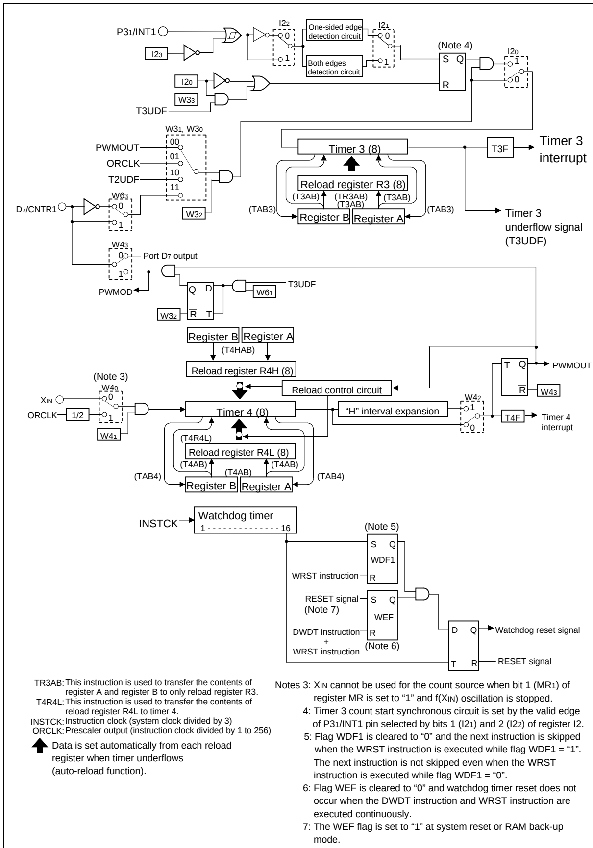
Fig. 26 Timer structure (2)
