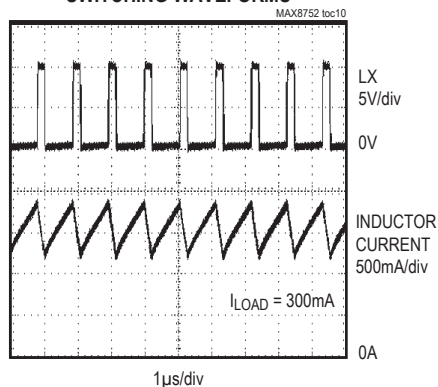
SWITCHING WAVEFORMS
