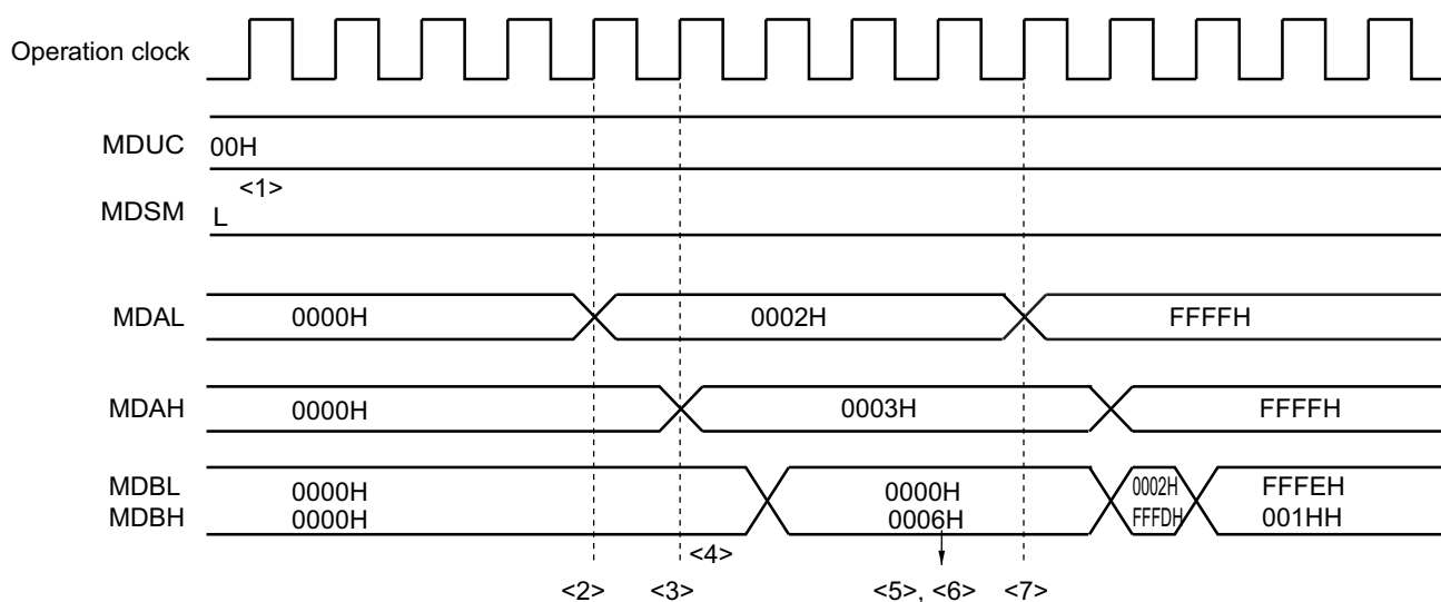
Figure 19-6. Timing Diagram of Multiplication (Unsigned) Operation ( 2 \times 3 = 6 )
