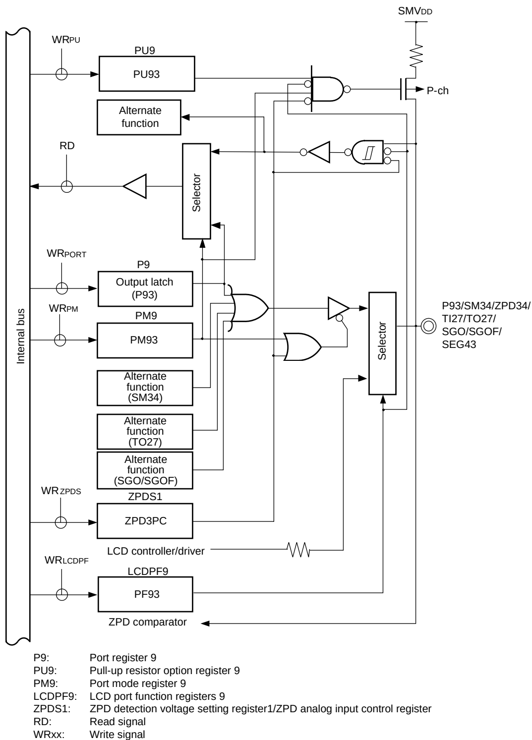
Figure 4-40. Block Diagram of P93
