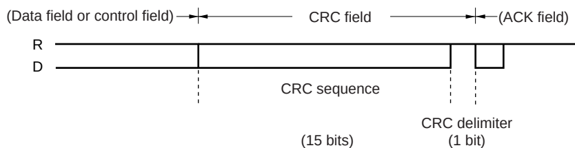
Figure 14-10. CRC Field
