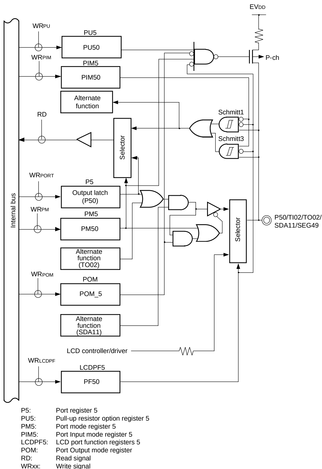
Figure 4-21. Block Diagram of P50
