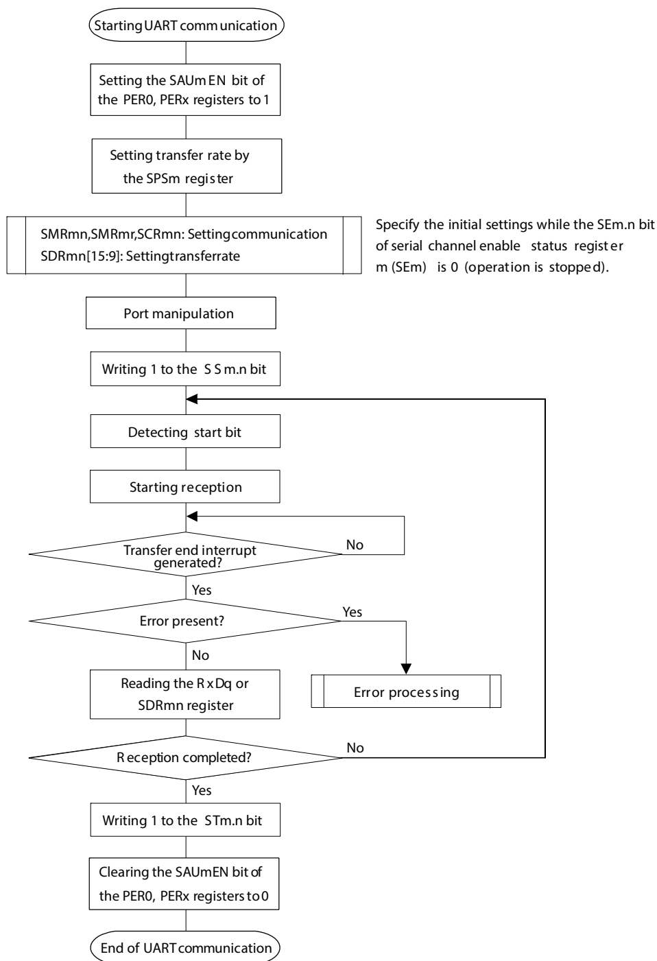
Figure 12-86. Flowchart of UART Reception
