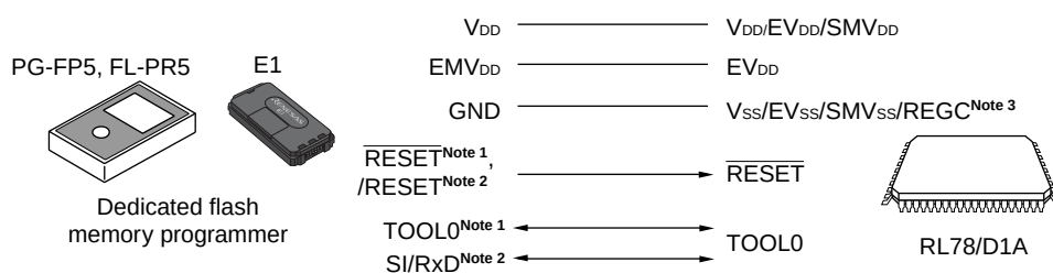
Figure 29-2. Communication with Dedicated Flash Memory Programmer
