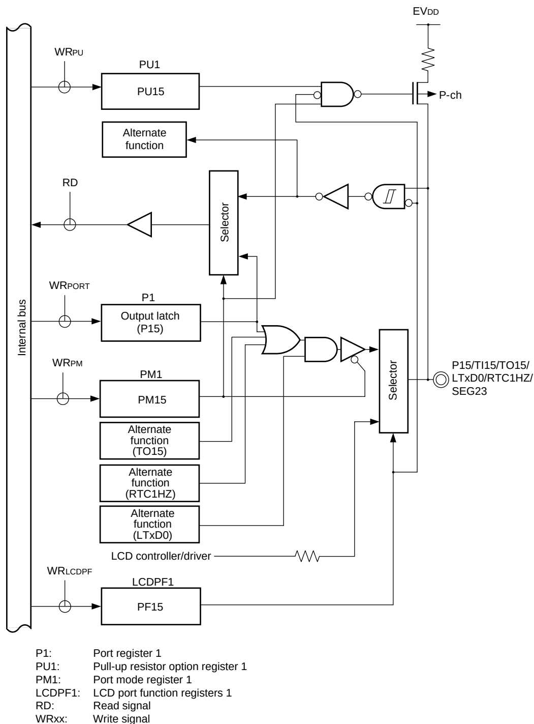
Figure 4-11. Block Diagram of P15
