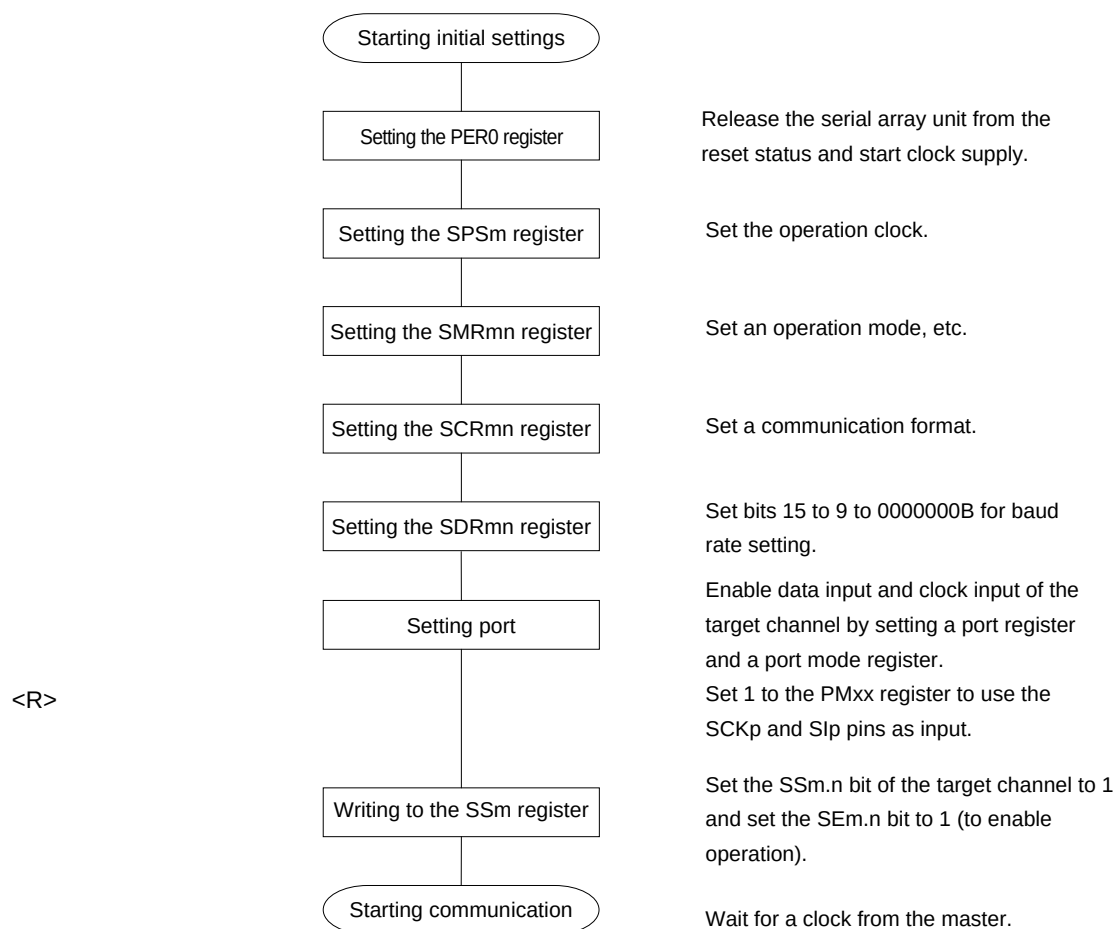
Figure 12-59. Initial Setting Procedure for Slave Reception
