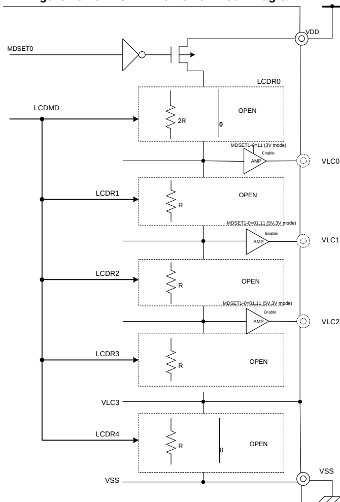
Figure 16-26. LCD Drive Power Block Diagram
