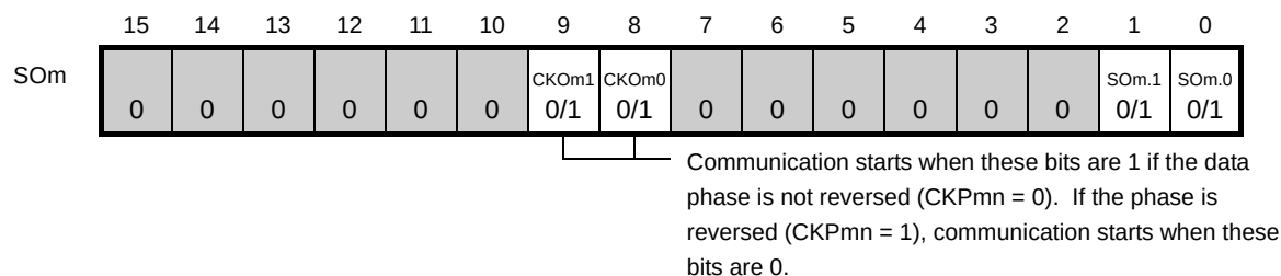
Figure 12-26. Example of Contents of Registers for Master Transmission of 3-Wire Serial I/O (CSI00, CSI01, CSI10) (1/2)
