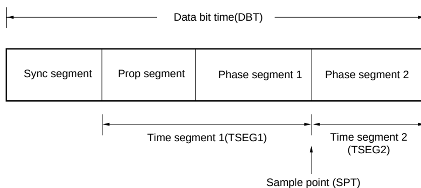
Figure 14-18. Segment Setting
