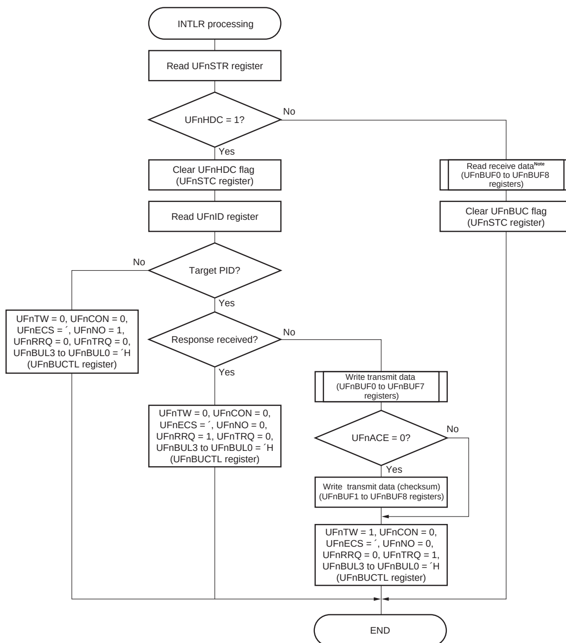
Figure 13-52. Basic Processing Flow Example of LIN Communication Automatic Baud Rate Mode (2/2)
