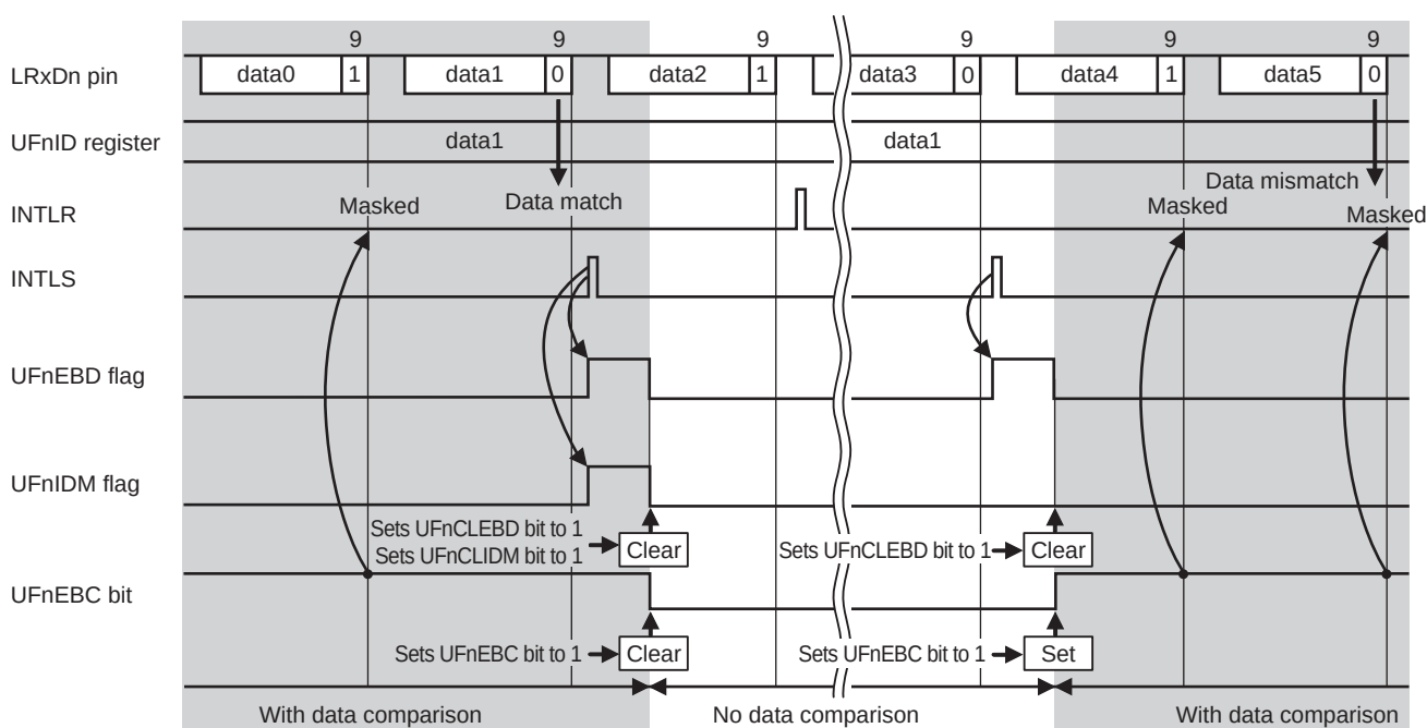
Figure 13-69. Expansion Bit Mode Reception (with Data Comparison) Example (LSB First, UFnEBL = 0 )
