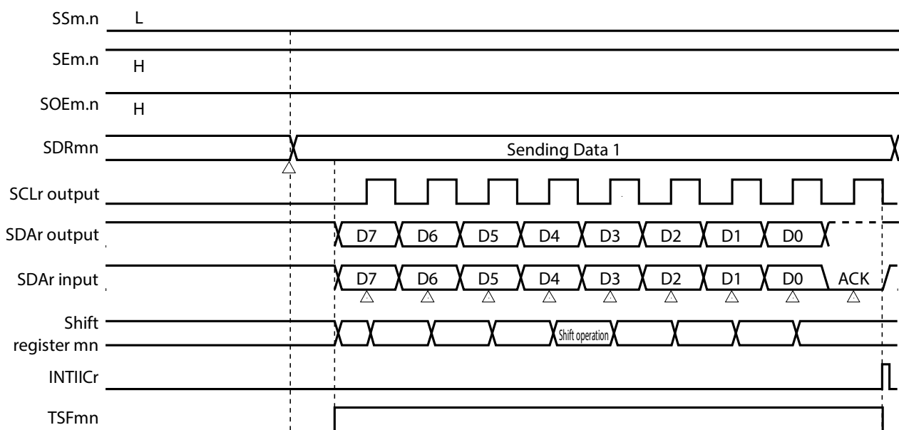
Figure 12-95. Timing Chart of Data Transmission
