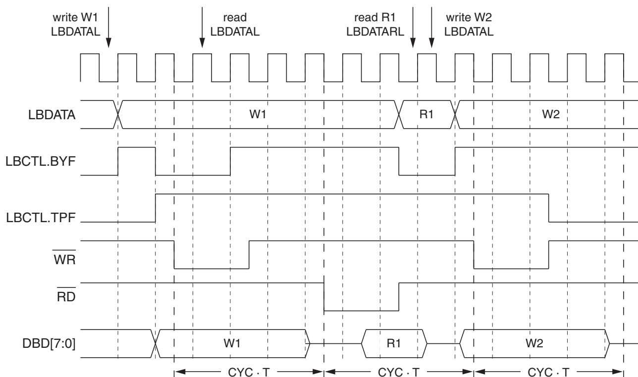
Figure 17-14. Timing (mod80: LBCTL.IMD = 0): 8-bit write-read-write, LBWST = 4, LBCYC = 7, LBCTL.TCIS = 0
