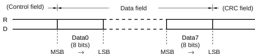
Figure 14-9. Data Field
