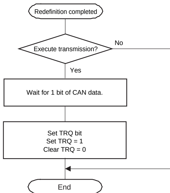
Figure 14-53. Setting Transmission Request (TRQ) to Transmit Message Buffer After Redefining
