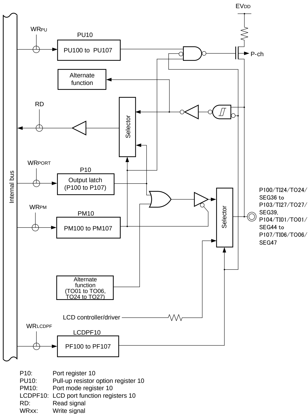
Figure 4-42. Block Diagram of P100 to P107
