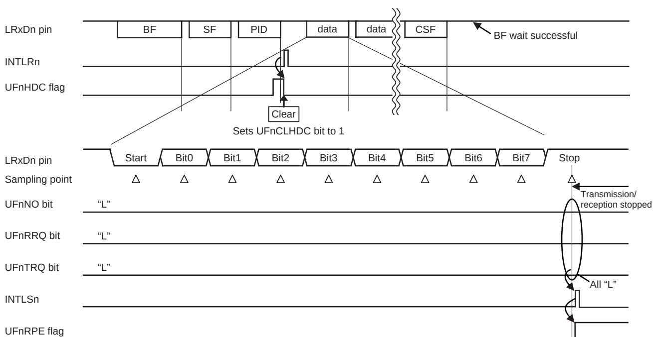
Figure 13-61. Response Preparation Error Occurrence Example
