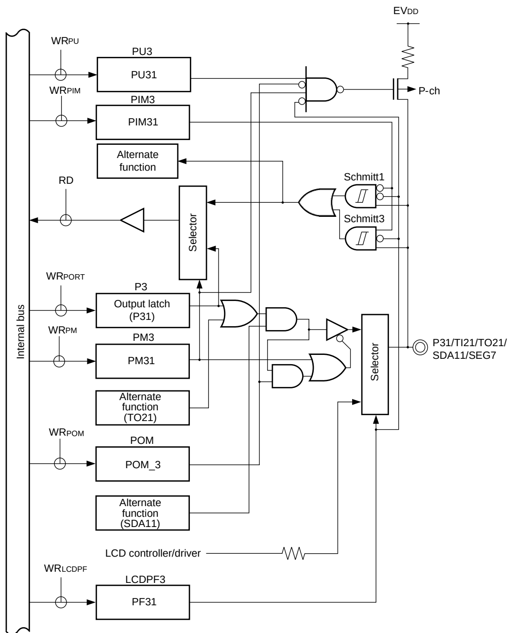
Figure 4-14. Block Diagram of P31
