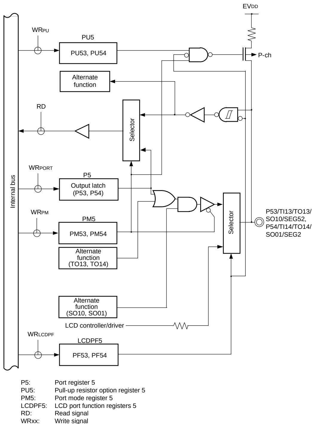
Figure 4-24. Block Diagram of P53, P54
