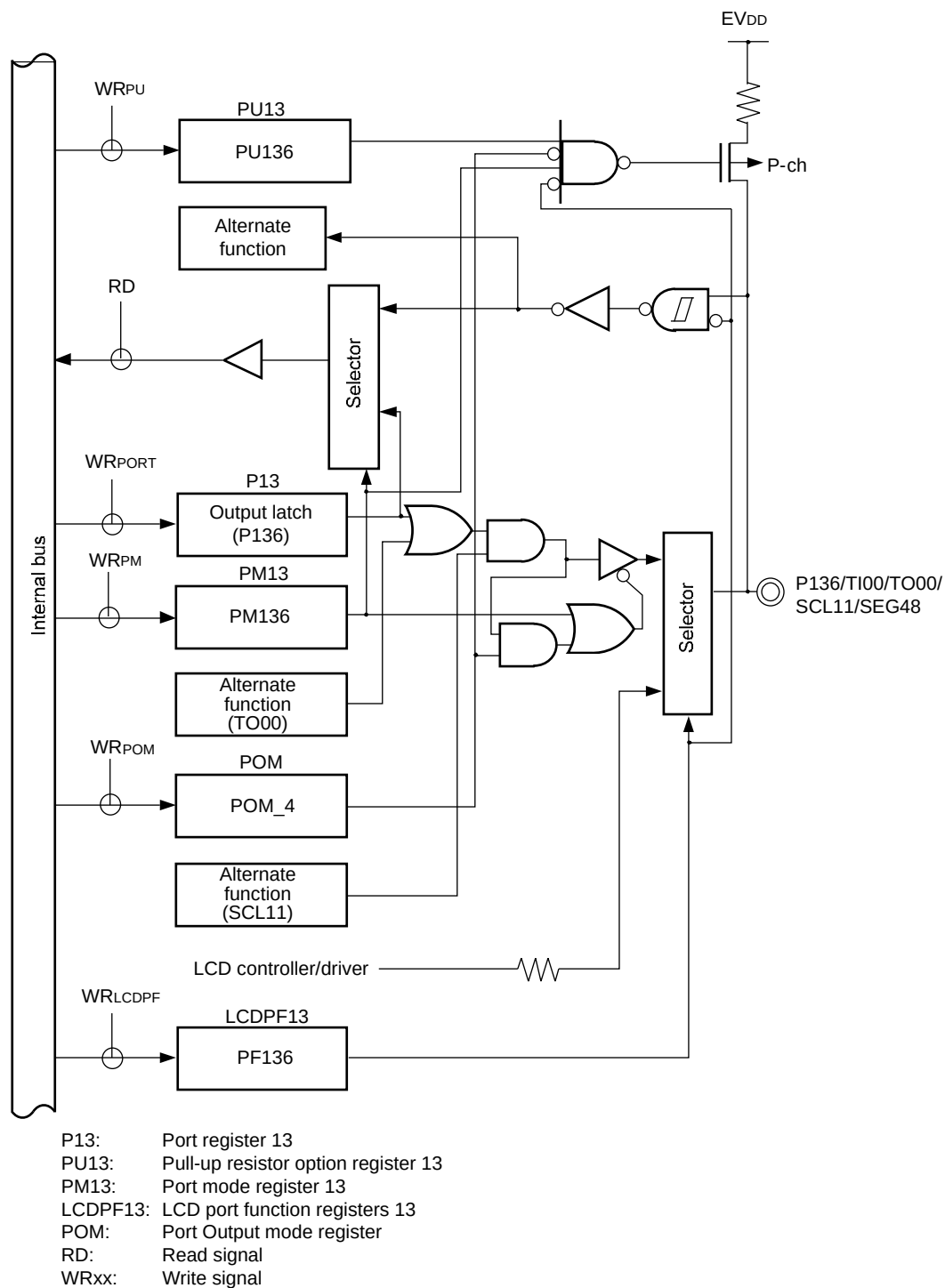
Figure 4-54. Block Diagram of P136
