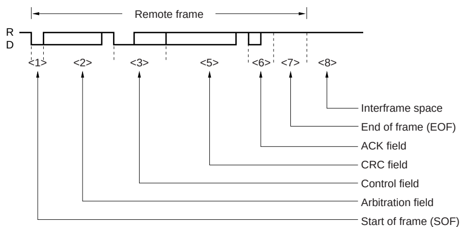
Figure 14-4. Remote Frame
