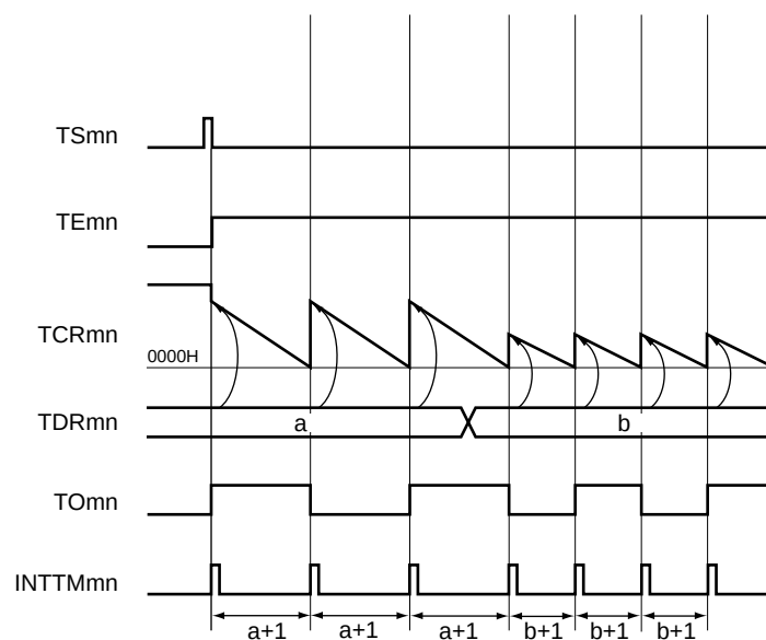
Figure 6-52. Example of Basic Timing of Operation as Interval Timer/Square Wave Output (MDmn0 = 1)
