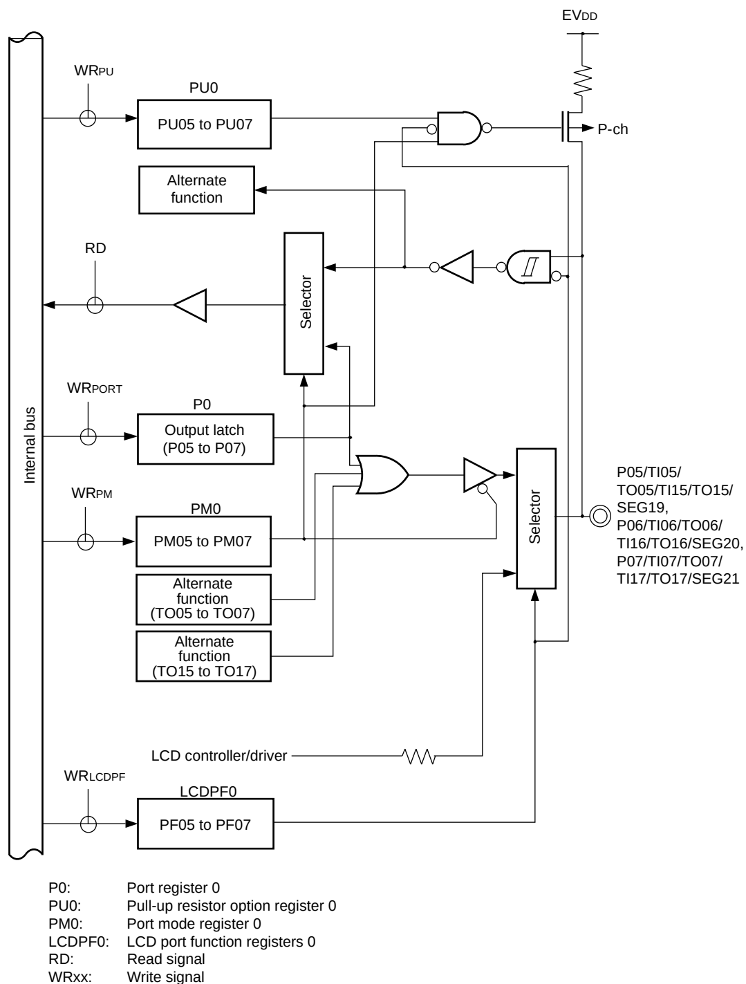
Figure 4-6. Block Diagram of P05 to P07
