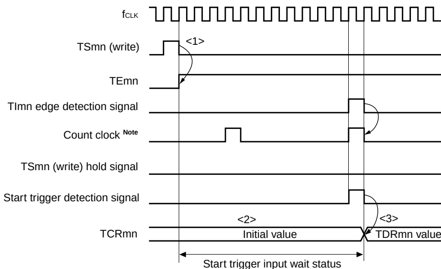
Figure 6-18. Start Timing (In One-count Mode)
