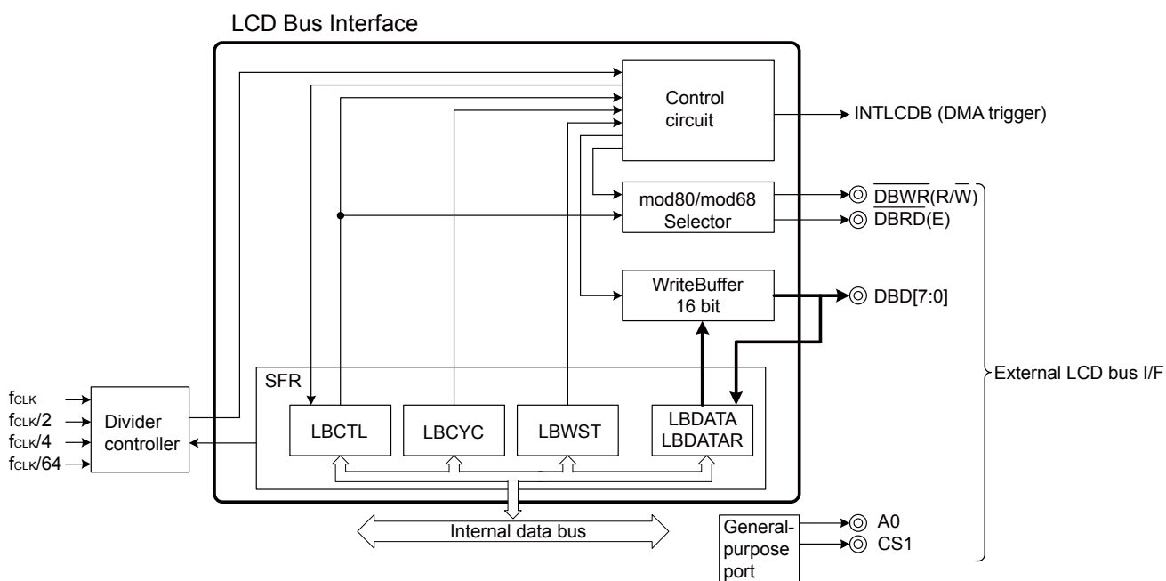
Figure 17-1. Block Diagram of LCD Bus Interface
