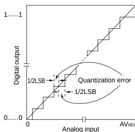
Figure 11-39. Quantization Error
