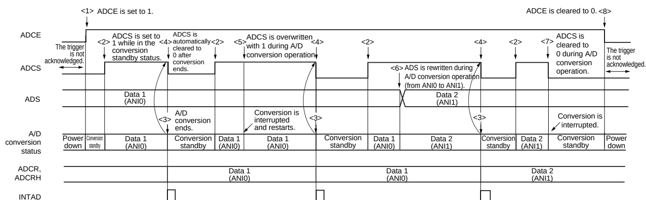
Figure 11-20. Example of Software Trigger Mode (Select Mode, One-Shot Conversion Mode) Operation Timing
