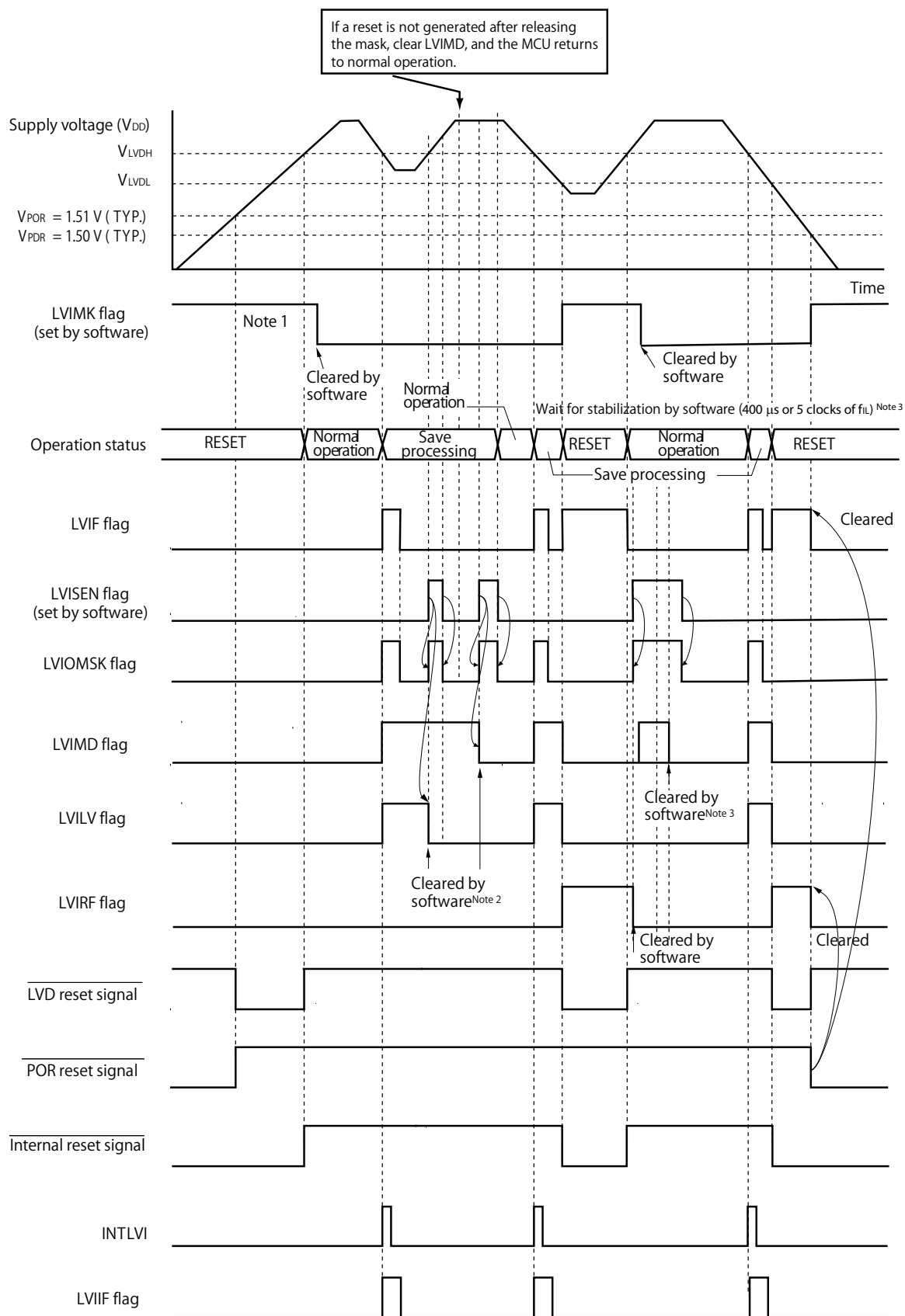
Figure 25-6. Timing of Voltage Detector Reset Signal and Interrupt Signal Generation (Option Byte LVIMDS1, LVIMDS0 = 1, 0) (1/2)
