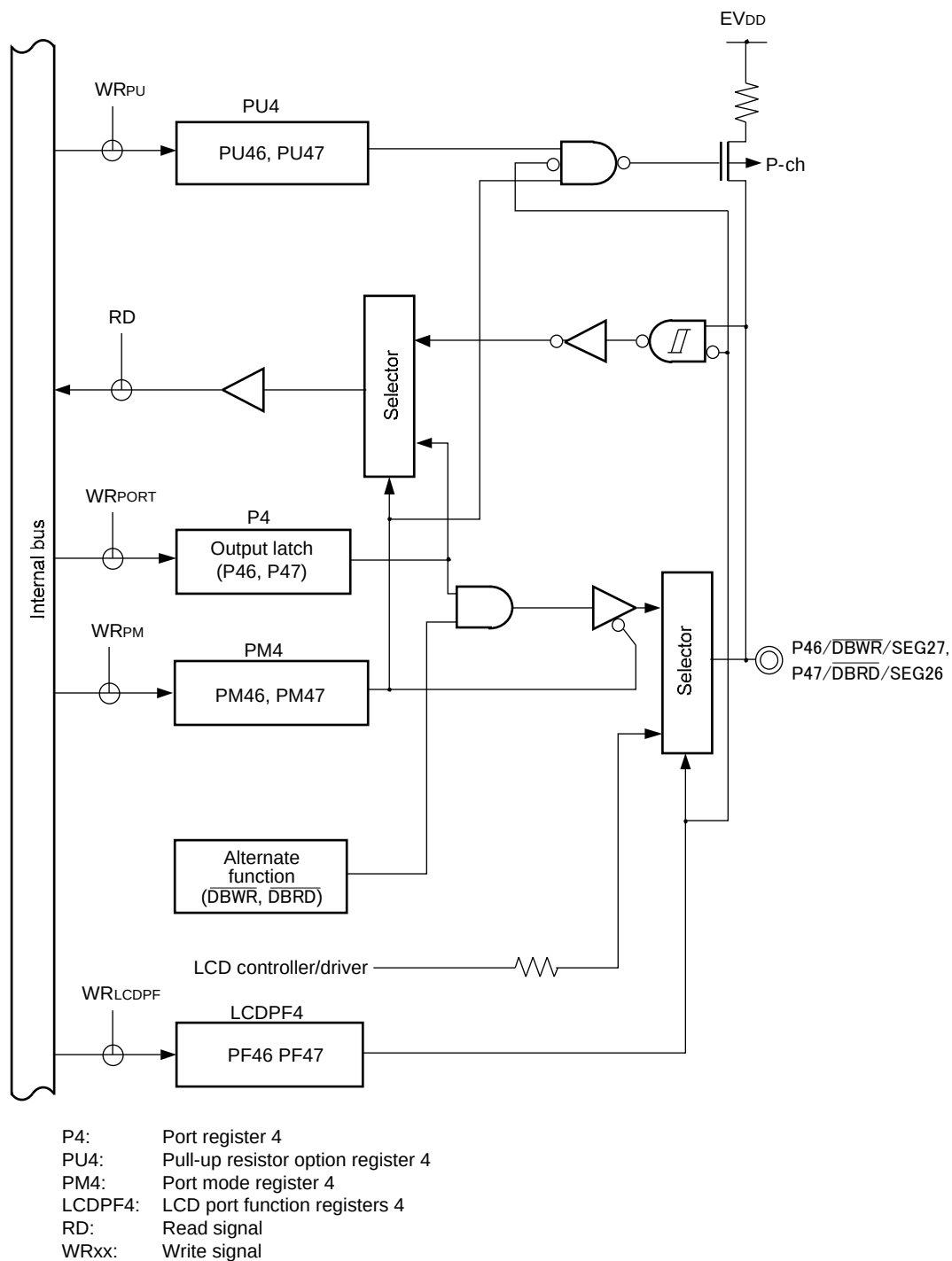
Figure 4-20. Block Diagram of P46, P47
