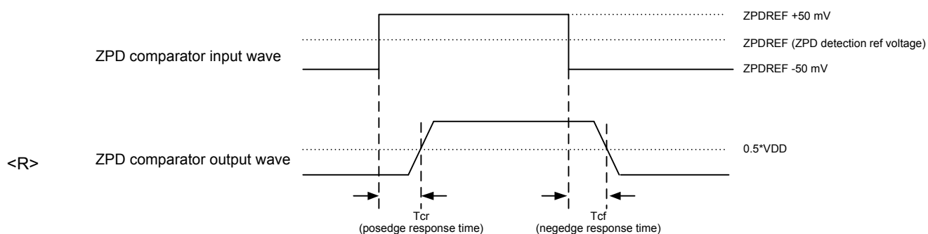
Figure 34-15. ZPD timing
