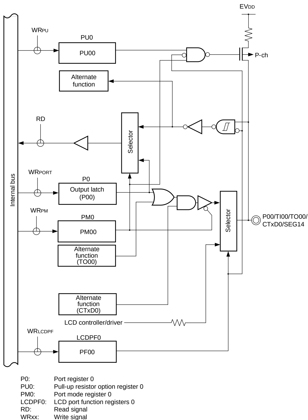
Figure 4-1. Block Diagram of P00
