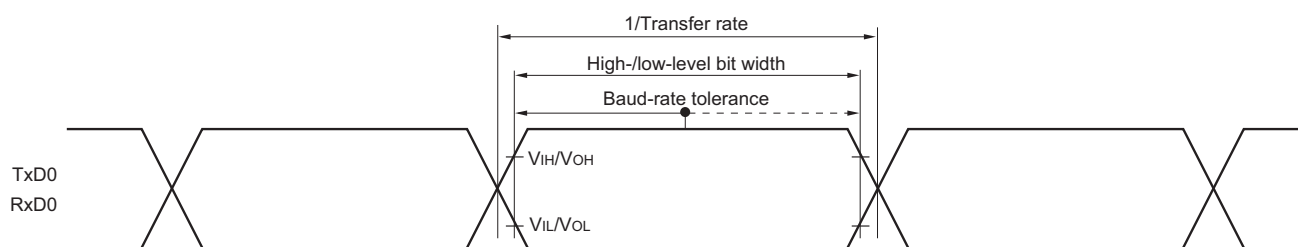
Figure 34-10. UART mode bit width (reference)
