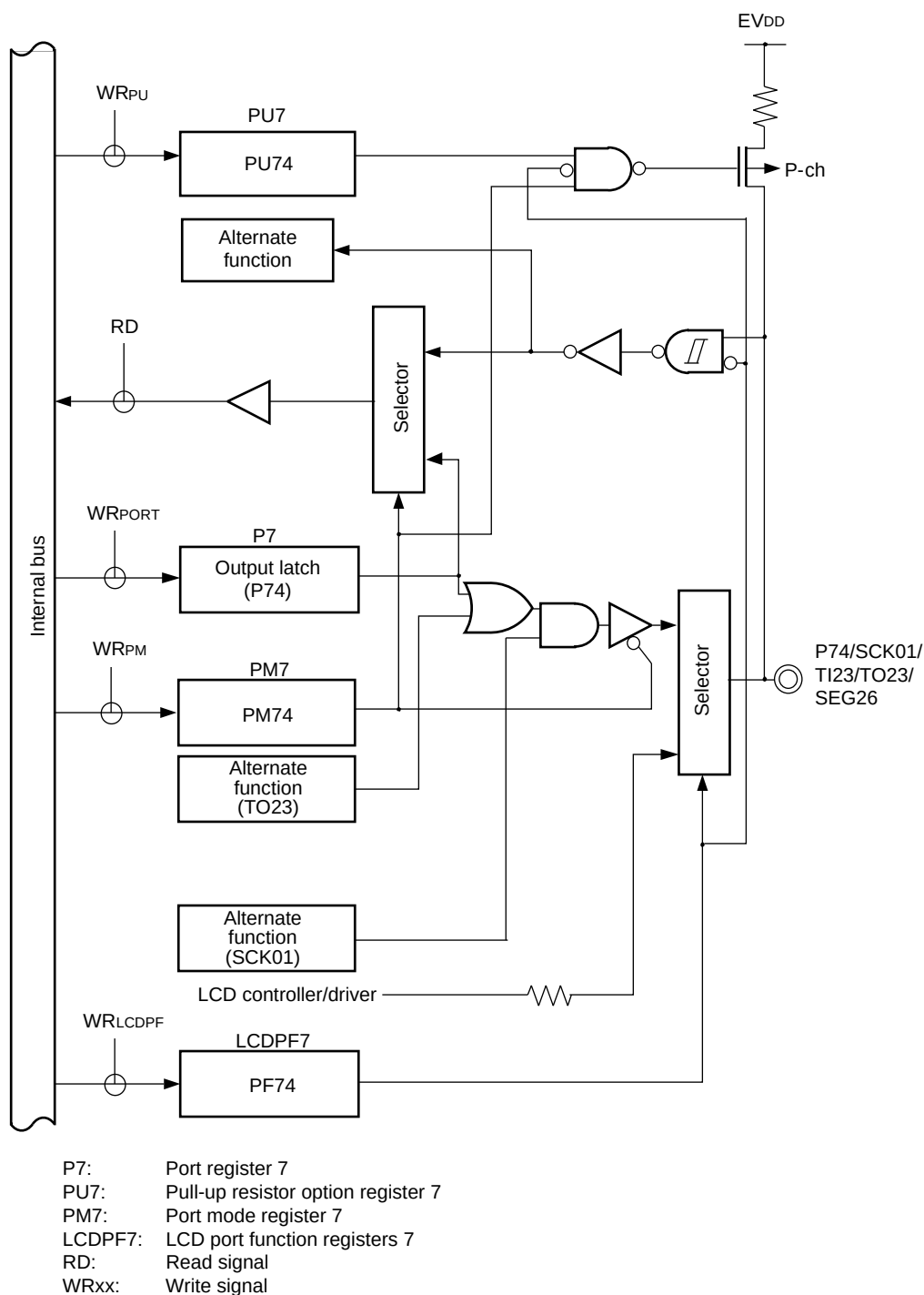
Figure 4-34. Block Diagram of P74
