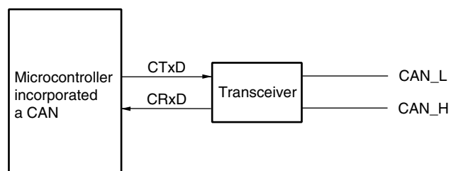
Figure 14-22. Connection to CAN Bus
