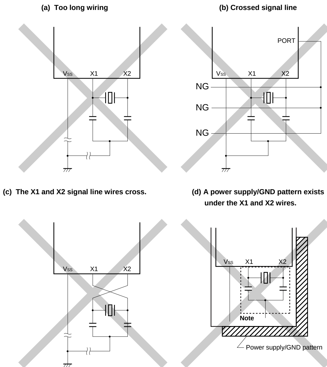
Figure 5-17. Examples of Incorrect Resonator Connection (1/2)
