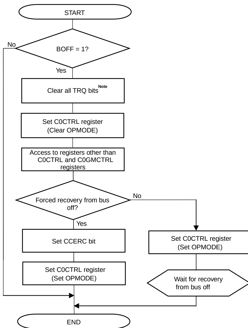
Figure 14-82. Bus-Off Recovery (Expect Normal Operation Mode with ABT)
