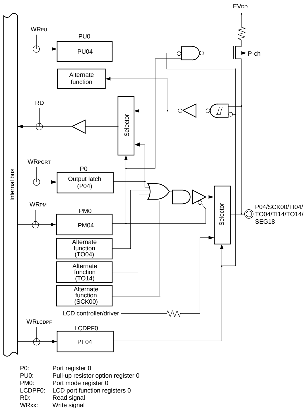
Figure 4-5. Block Diagram of P04
