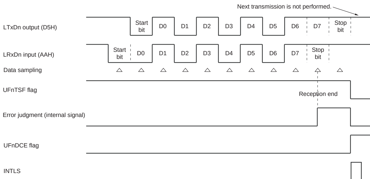
Figure 13-39. Timing Example of Consistency Error Occurrence due to Early End of Reception Processing
