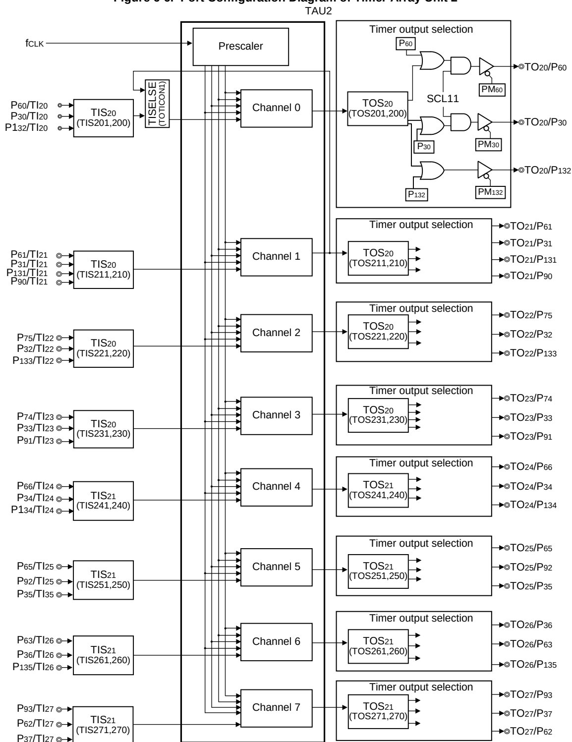
Figure 6-6. Port Configuration Diagram of Timer Array Unit 2
