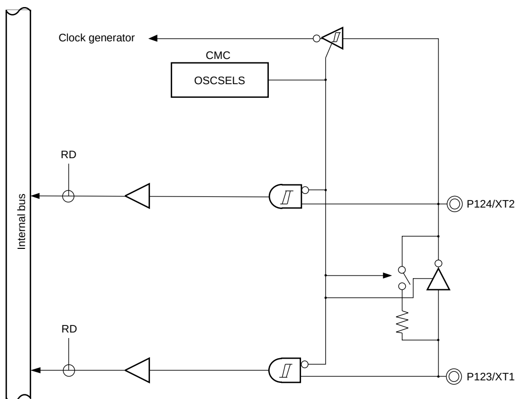
Figure 4-46. Block Diagram of P123, P124
