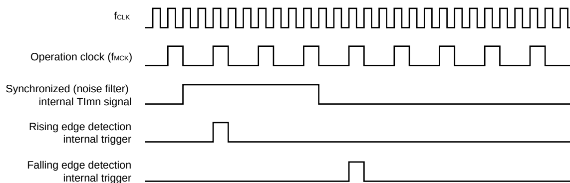
Figure 6-50. Edge Detection Basic Operation Timing
