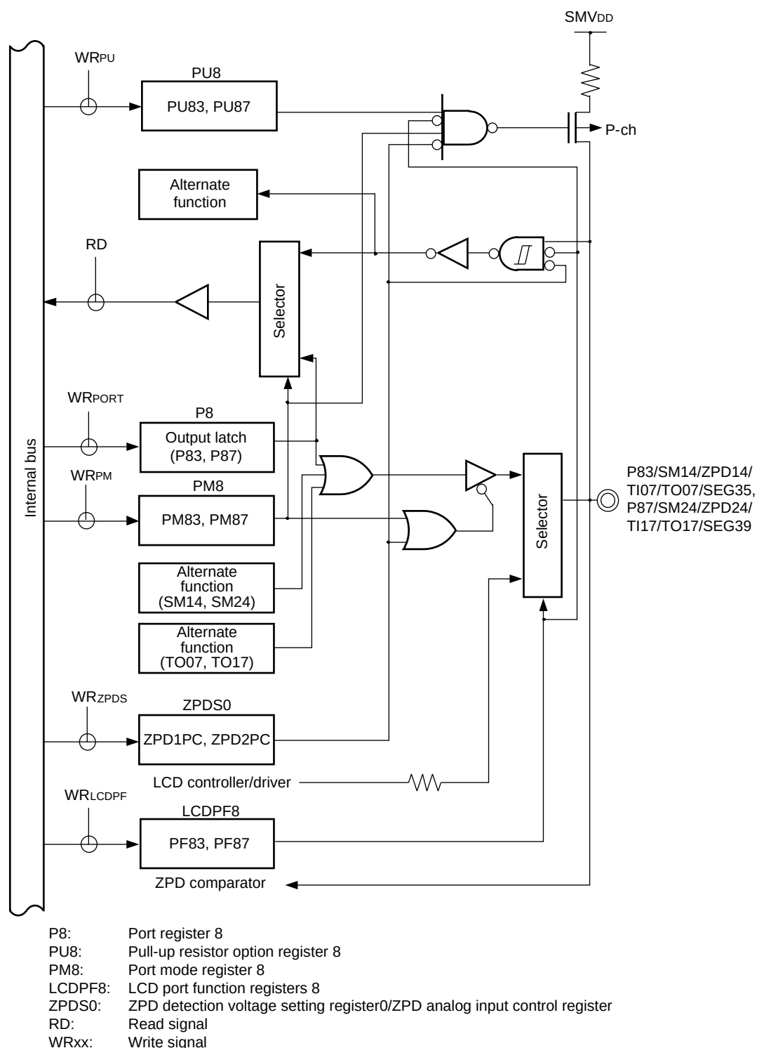
Figure 4-37. Block Diagram of P83, P87
