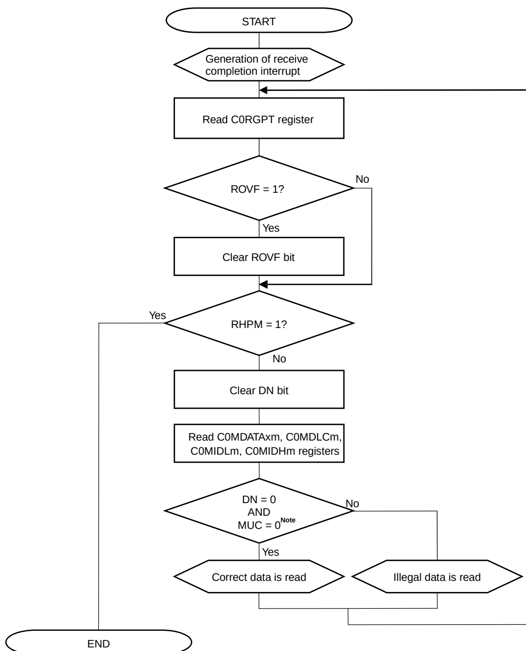
Figure 14-78. Reception via Interrupt (Using C0RGPT Register)
