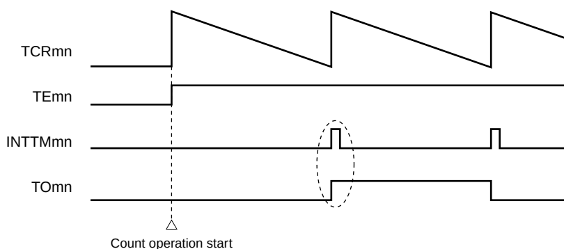
Figure 6-49. When MDmn0 Is Set to 0
