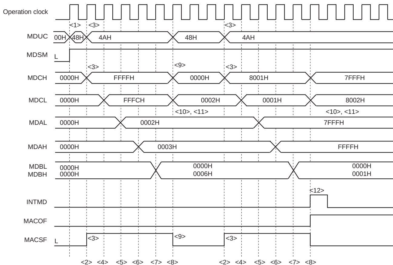
Figure 19-9. Timing Diagram of Multiply-Accumulation (signed) Operation (2 \times 3 + (-4) = 2 \rightarrow 32767 \times (-1) + (-2147483647) = -2147450882 \text{ (overflow occurs.)})
