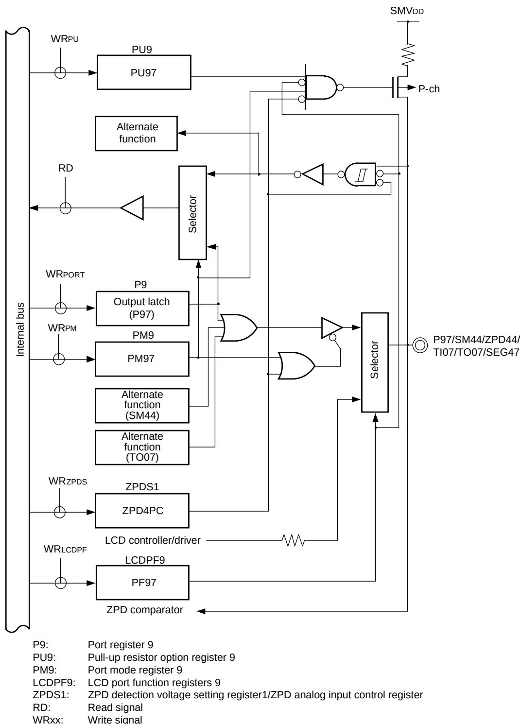
Figure 4-41. Block Diagram of P97
