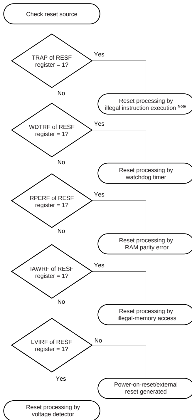
Figure 25-9. Checking reset source
