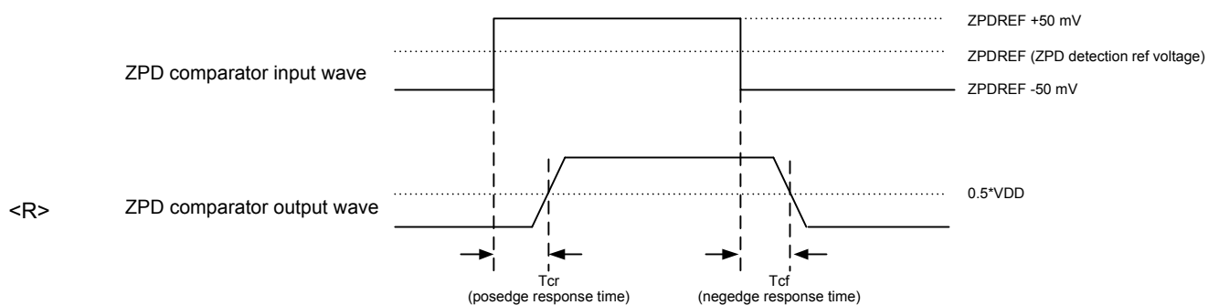
Figure 33-15. ZPD timing
