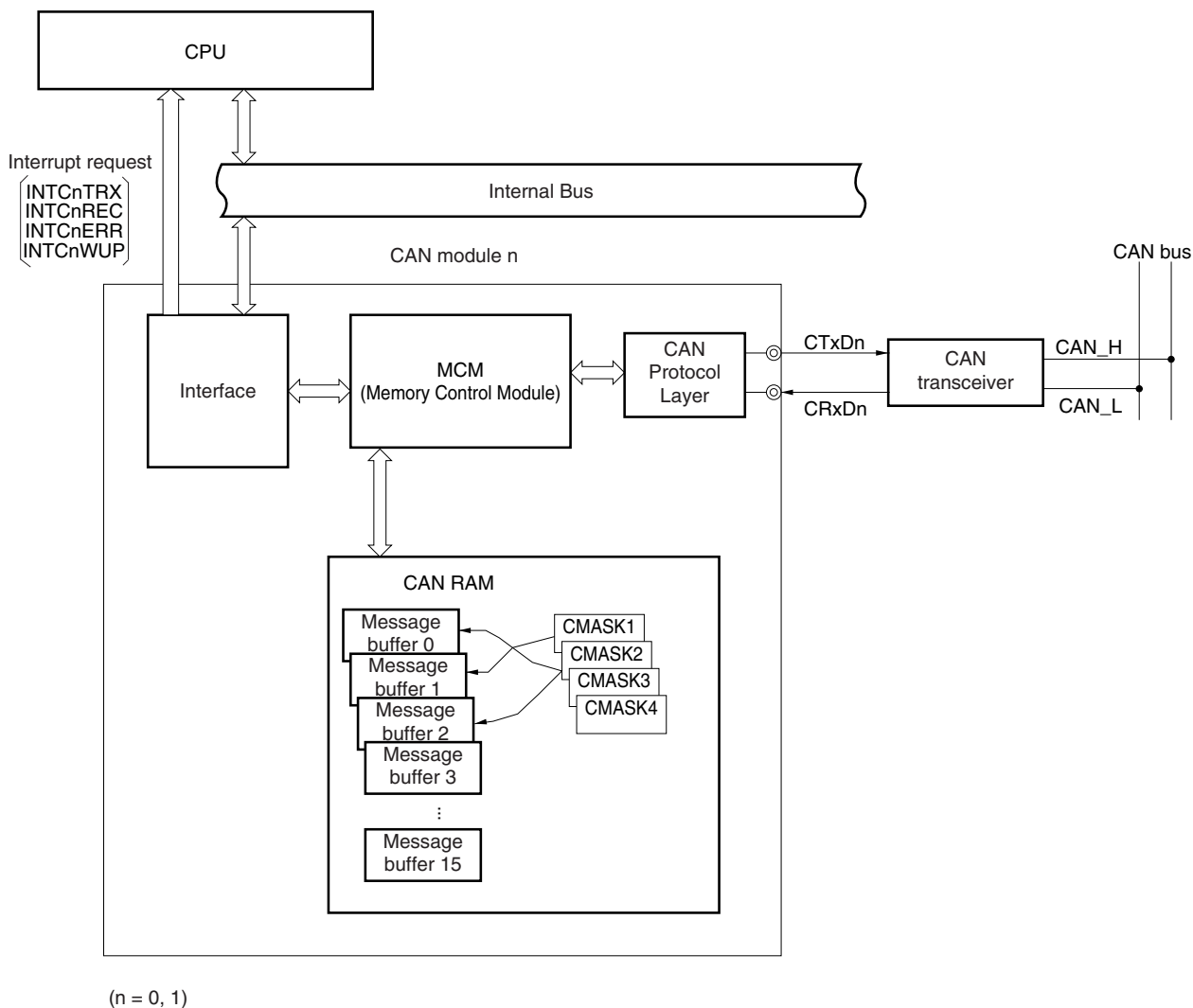
Figure 14-1. Block Diagram of CAN Module n
