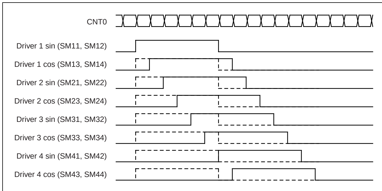
Figure 15-12. Output Timing of Signals SM11 to SM44
