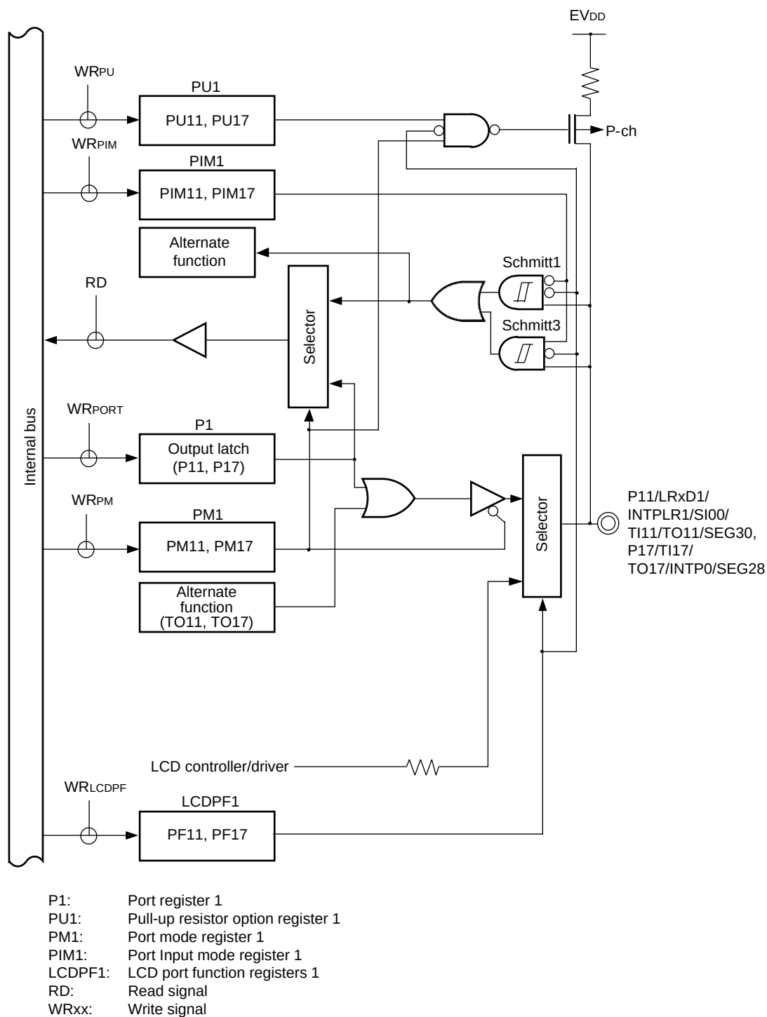
Figure 4-8. Block Diagram of P11, P17
