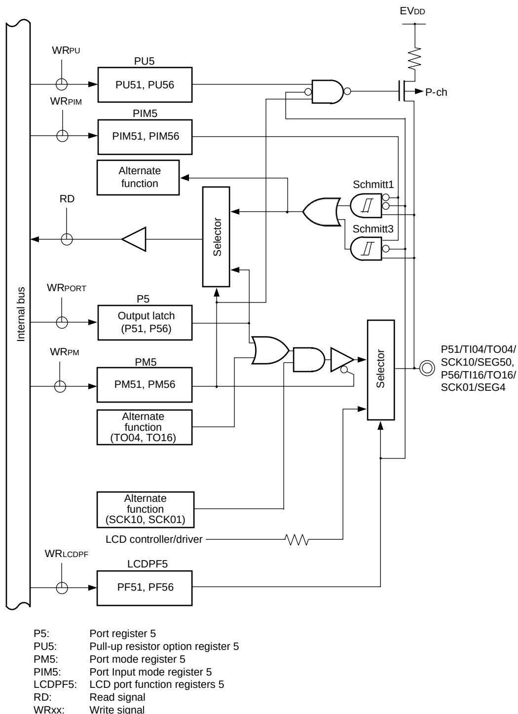
Figure 4-22. Block Diagram of P51, P56
