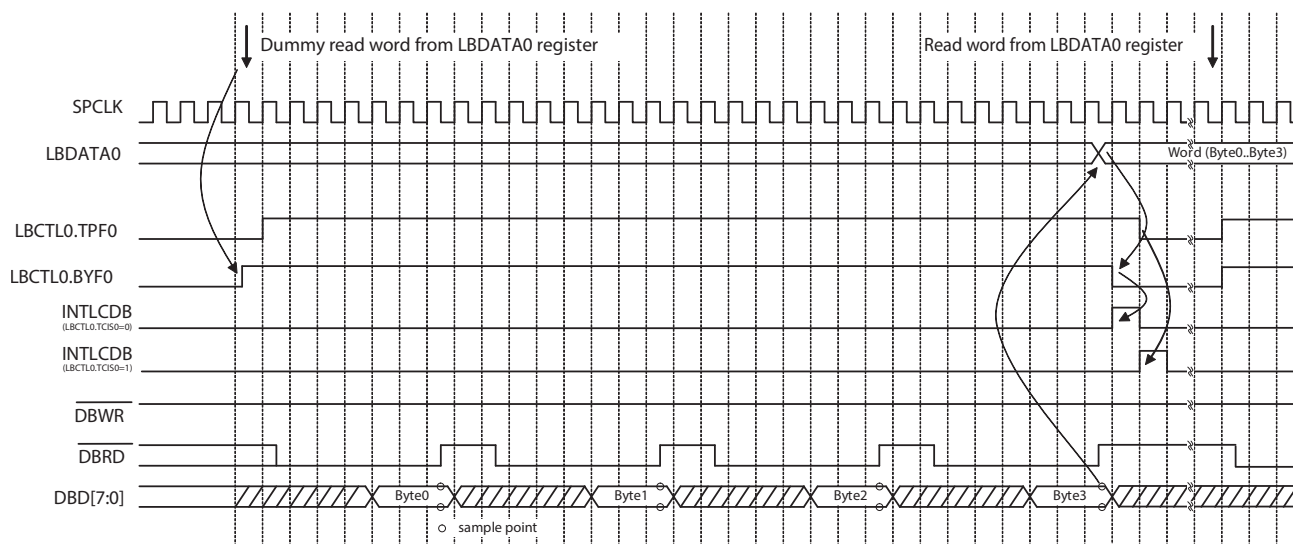
Figure 17-12. Timing (mod80: LBCTL.IMD = 0): read word, LBWST = 5, LBCYC = 8, LBCTL.TCIS = 0 and 1
