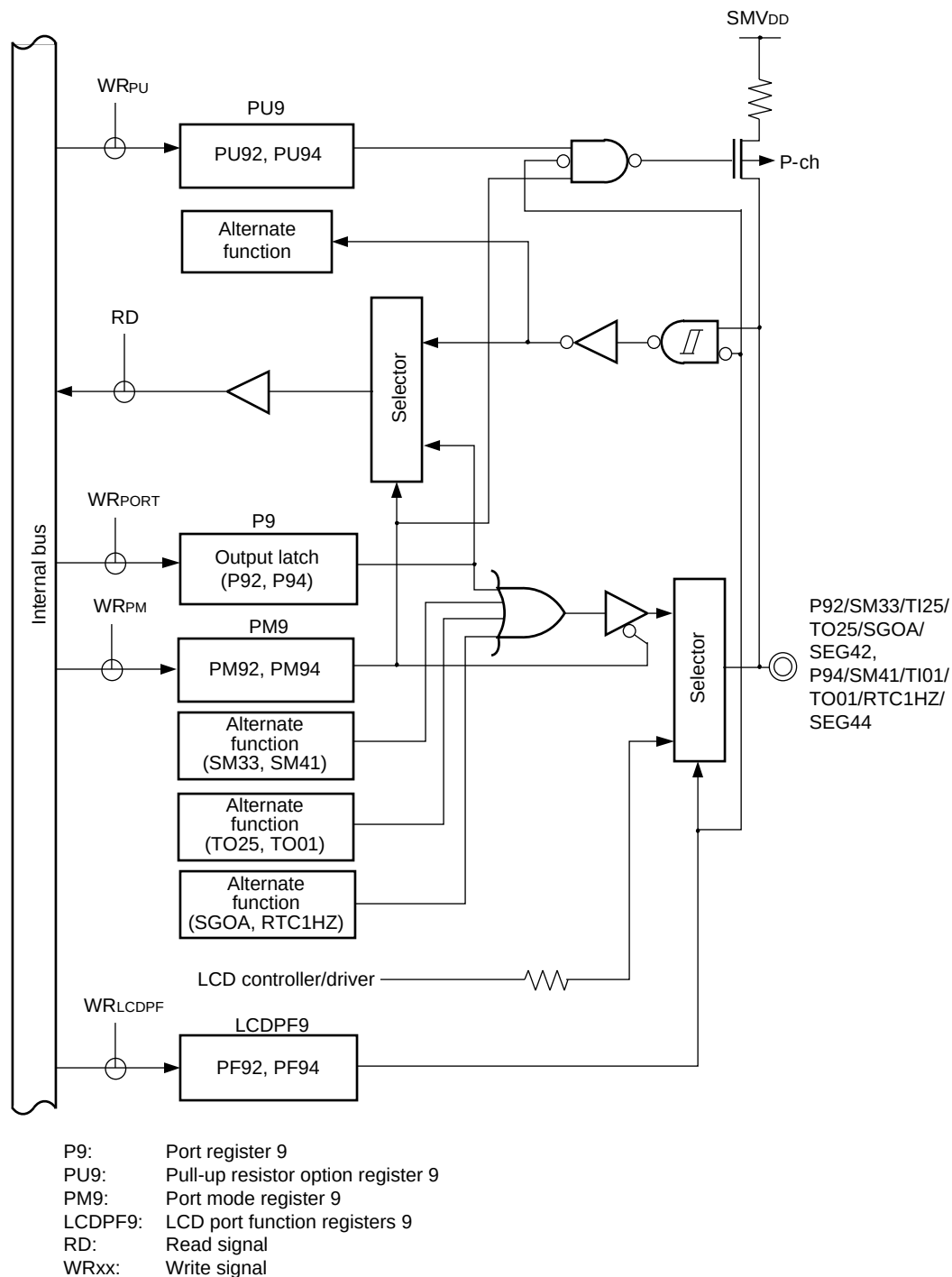
Figure 4-39. Block Diagram of P92, P94
