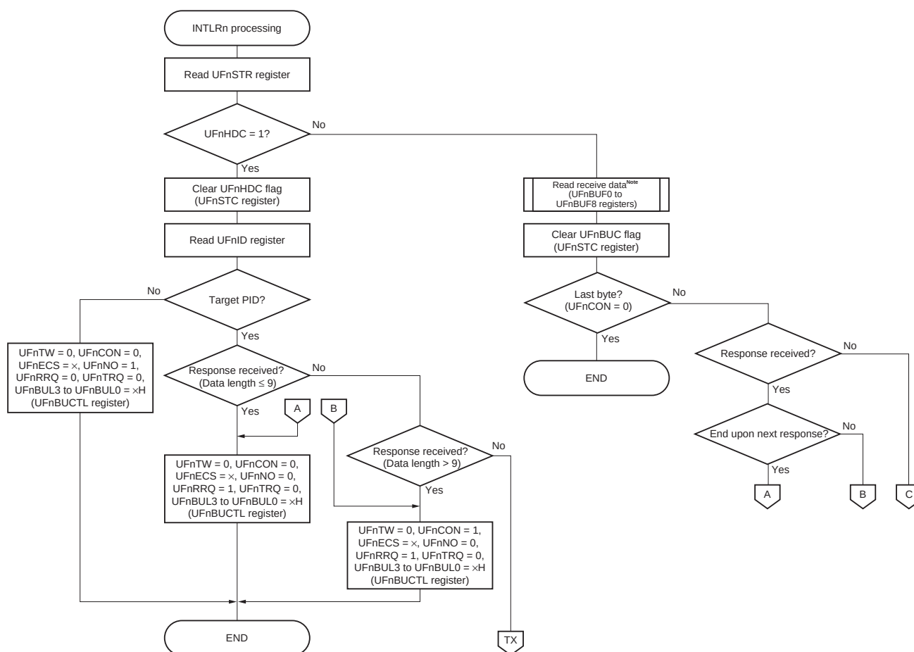
Figure 13-64. Multi-Byte Transmission/Reception Processing Flow Example (1/2)
