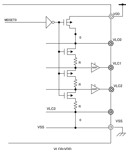
(a) 1/3 bias method and static display mode (MDSET1, MDSET0 = 0, 1) (example of V_{DD} = 5\text{ V} , V_{LC0} = 5\text{ V} )
