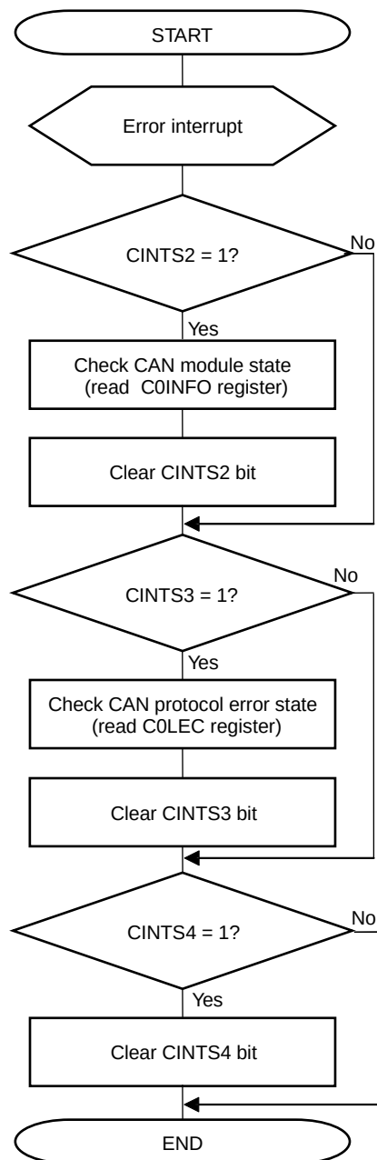
Figure 14-86. Error Handling
