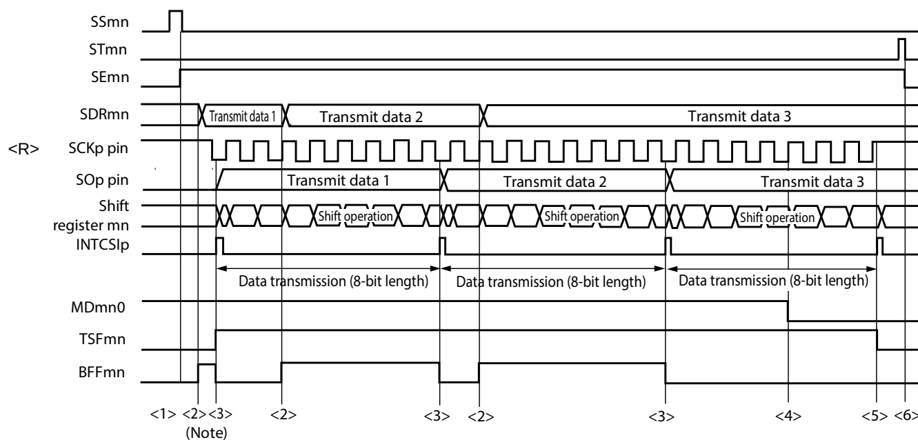
Figure 12-56. Timing Chart of Slave Transmission (in Continuous Transmission Mode)
