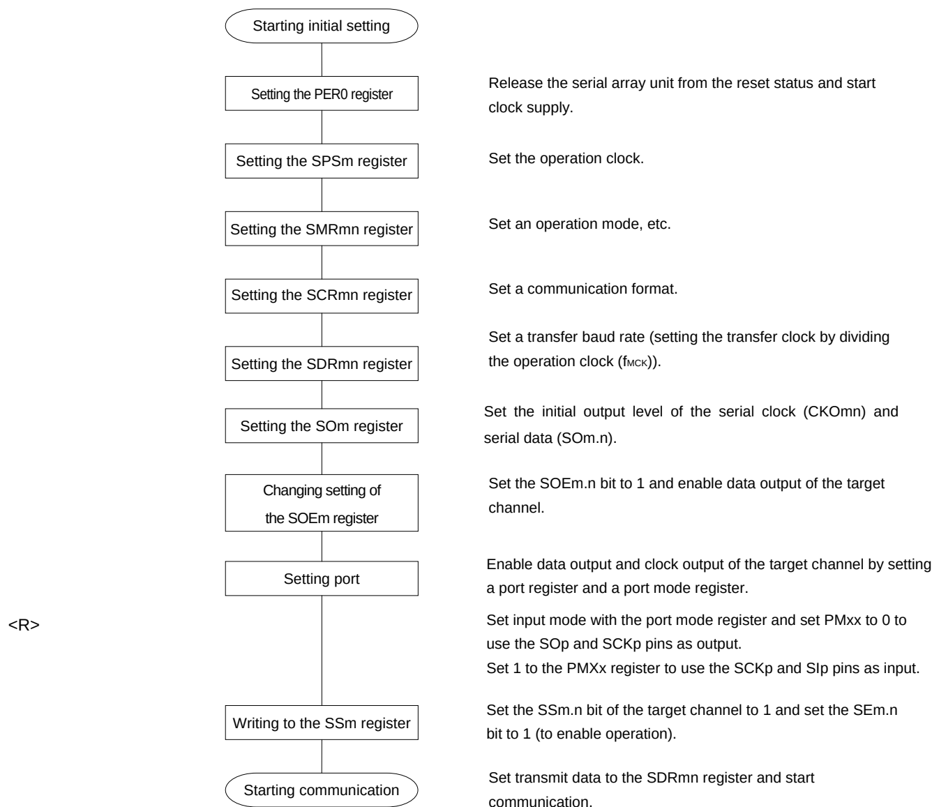
Figure 12-43. Initial Setting Procedure for Master Transmission/Reception
