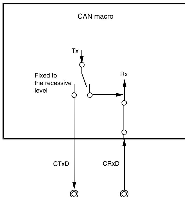
Figure 14-59. CAN Module Terminal Connection in Receive-Only Mode
