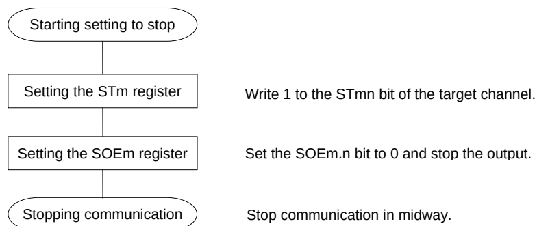
Figure 12-75. Procedure for Stopping UART Transmission
