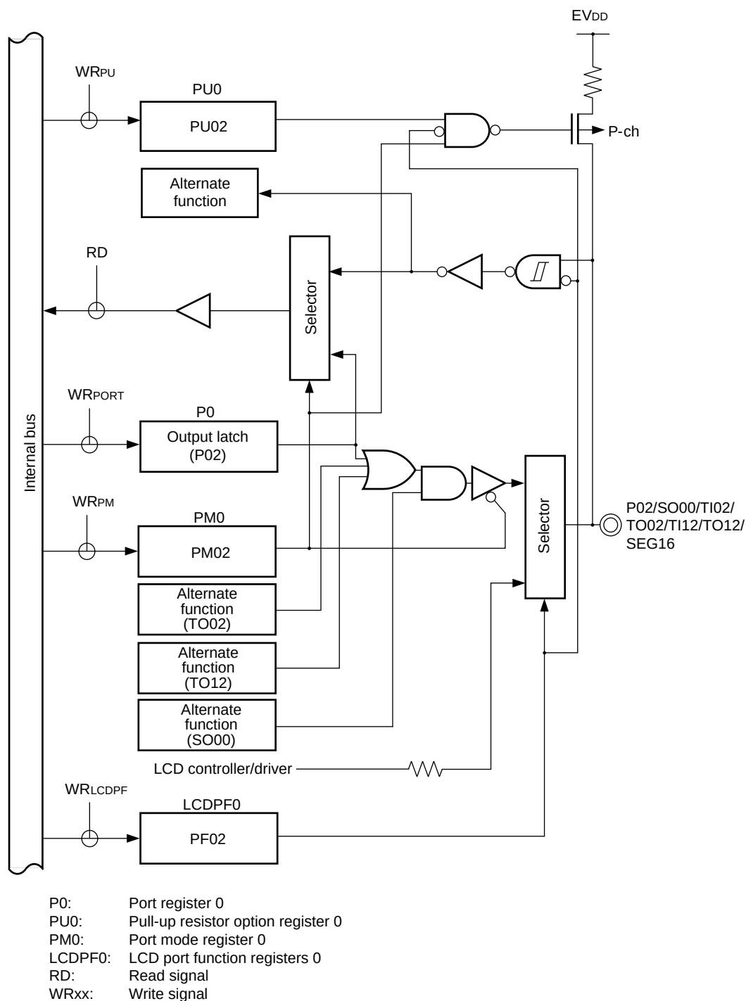
Figure 4-3. Block Diagram of P02
