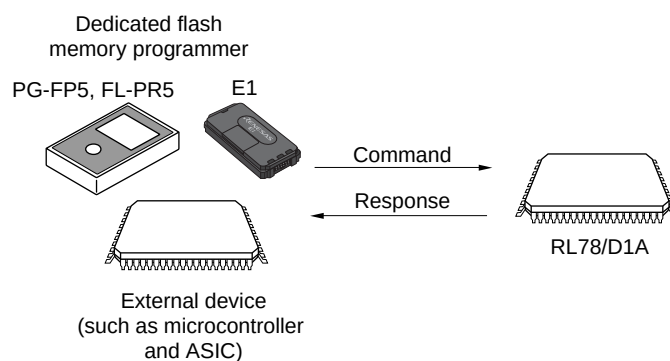
Figure 29-9. Communication Commands
