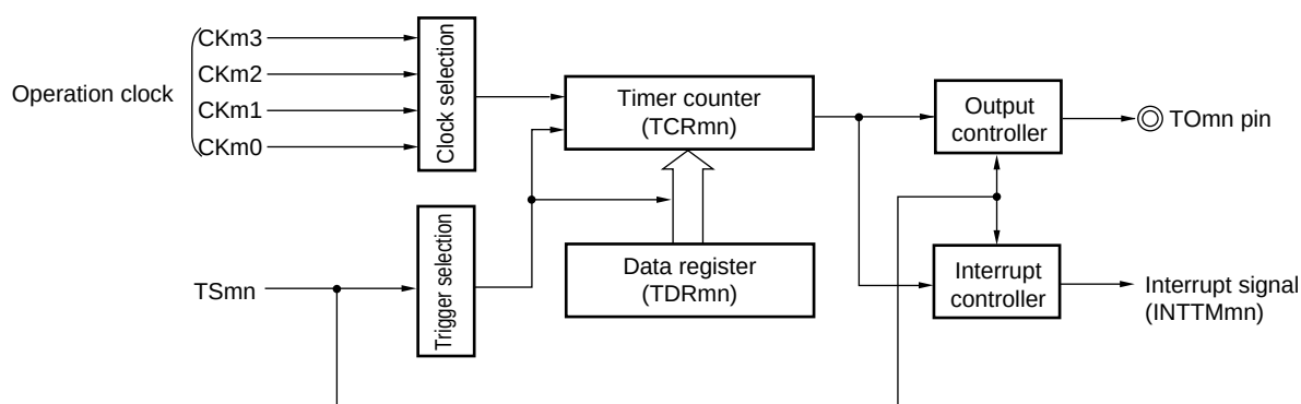
Figure 6-51. Block Diagram of Operation as Interval Timer/Square Wave Output
