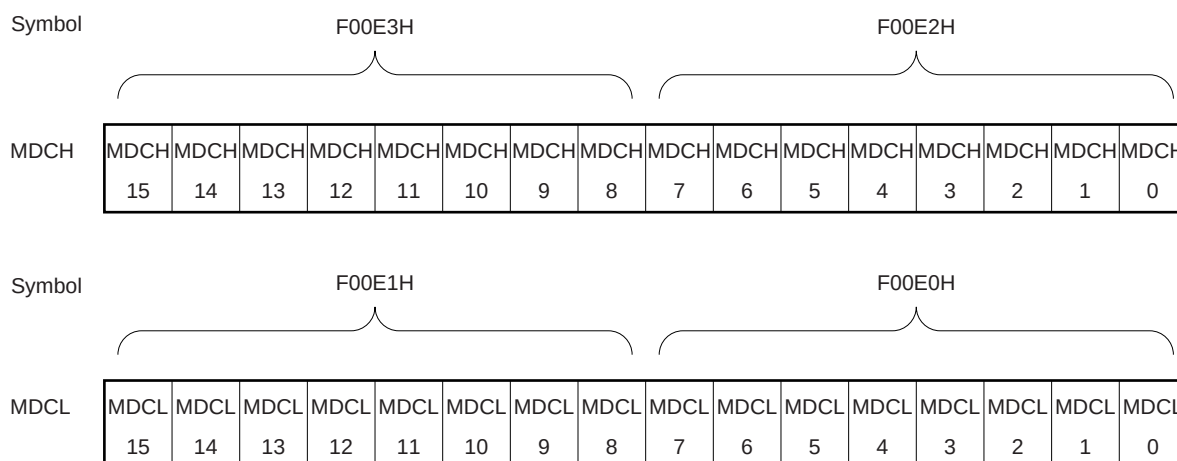
Figure 19-4. Format of Multiplication/Division Data Register C (MDCH, MDCL)
