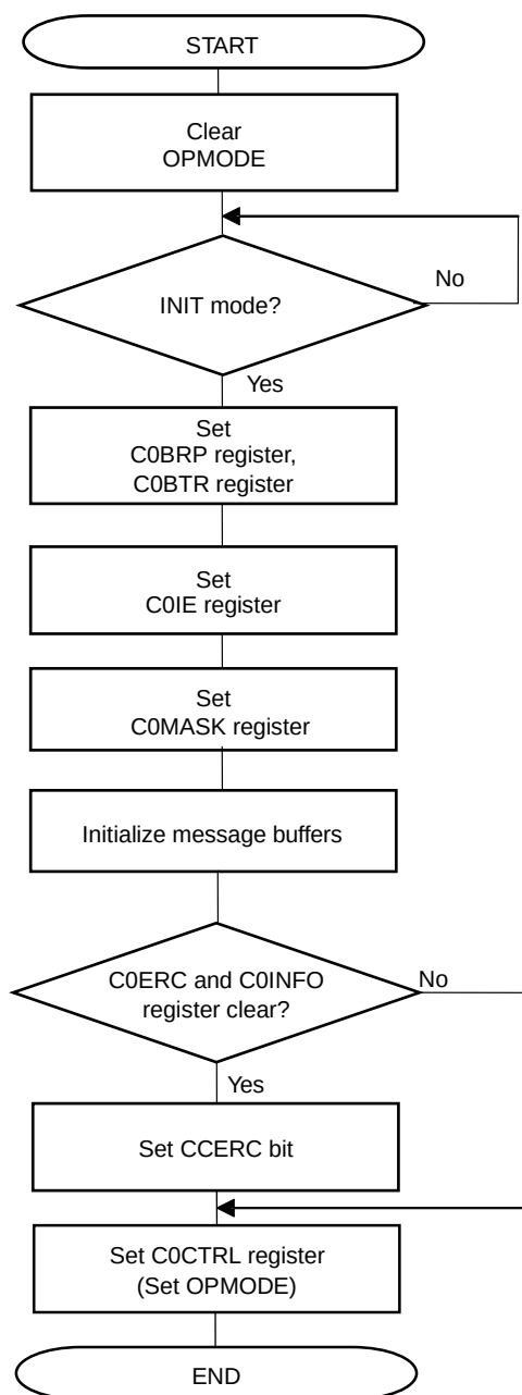
Figure 14-64. Re-initialization
