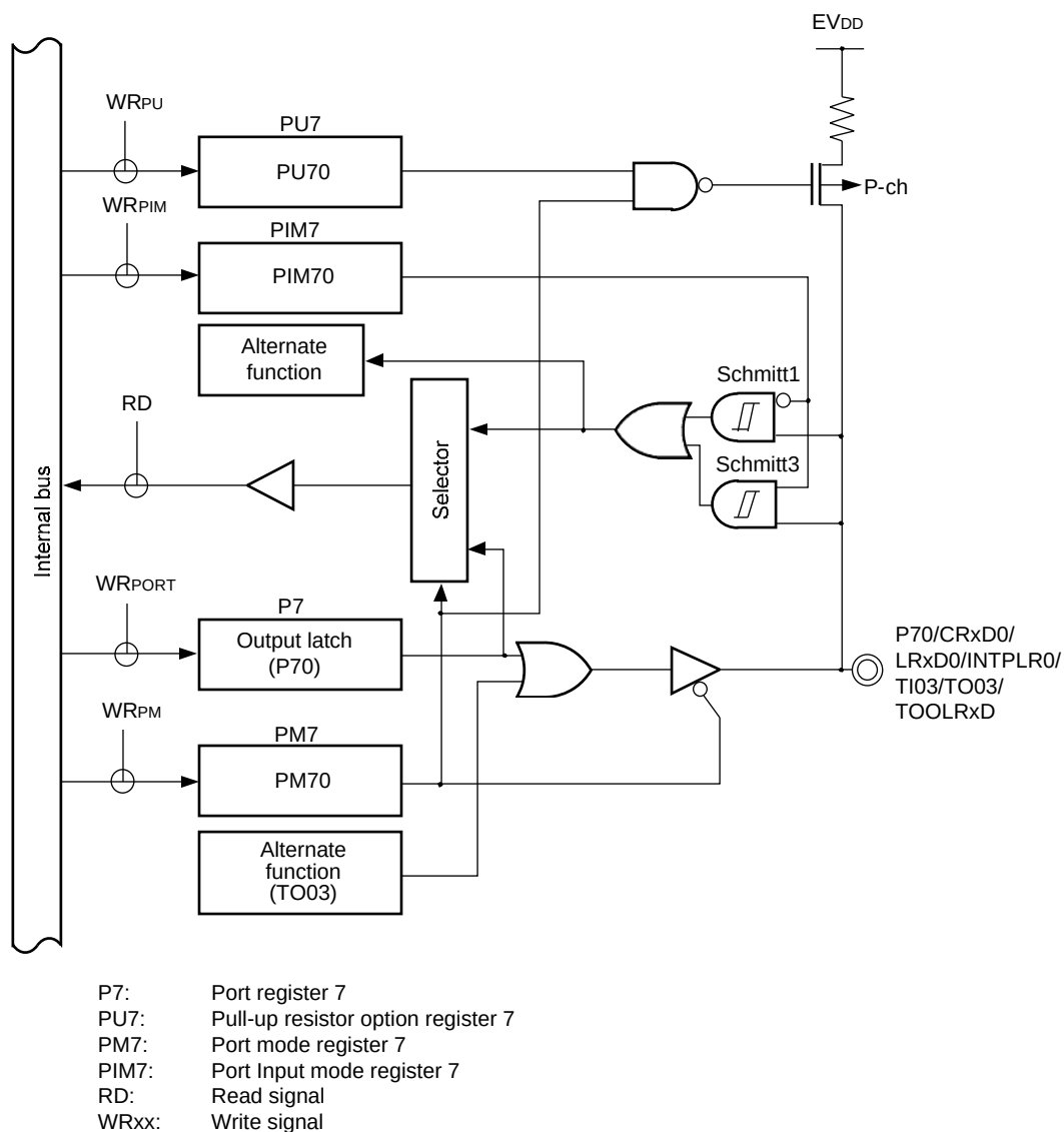
Figure 4-31. Block Diagram of P70
