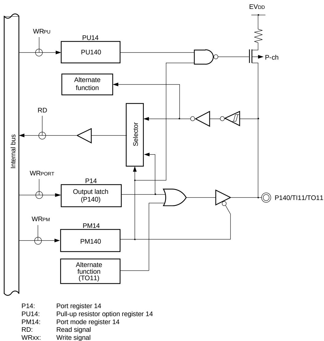
Figure 4-56. Block Diagram of P140
