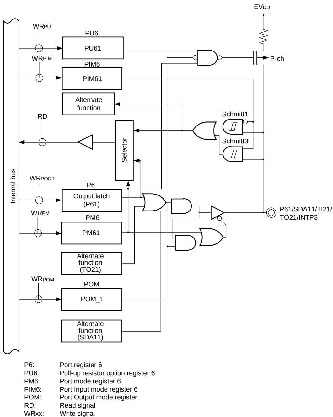
Figure 4-26. Block Diagram of P61
