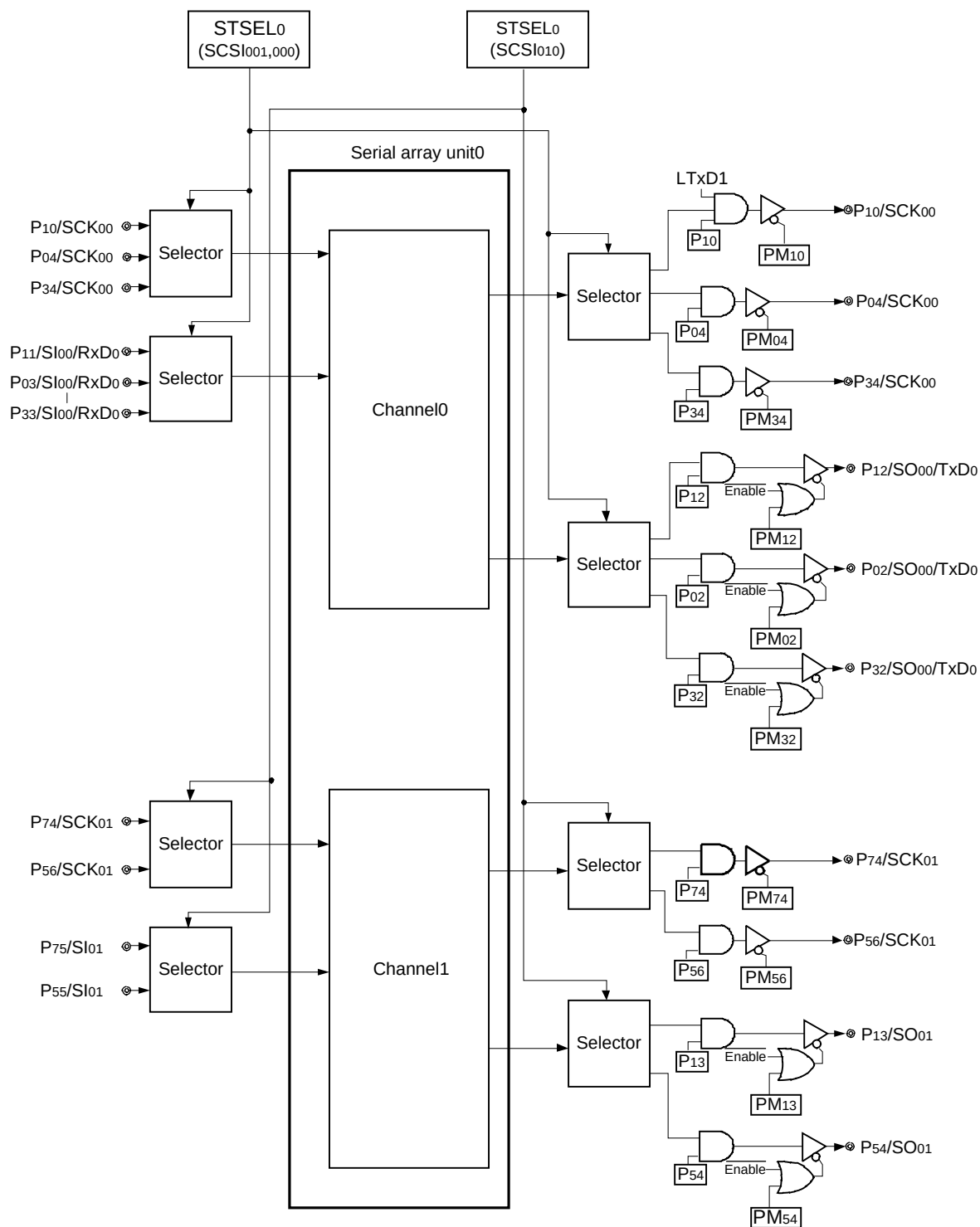
Figure 12-2. Port Configuration Diagram of Serial Array Unit 0
