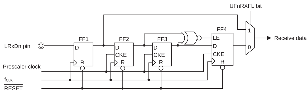
Figure 13-70. Noise Filter Circuit Example
