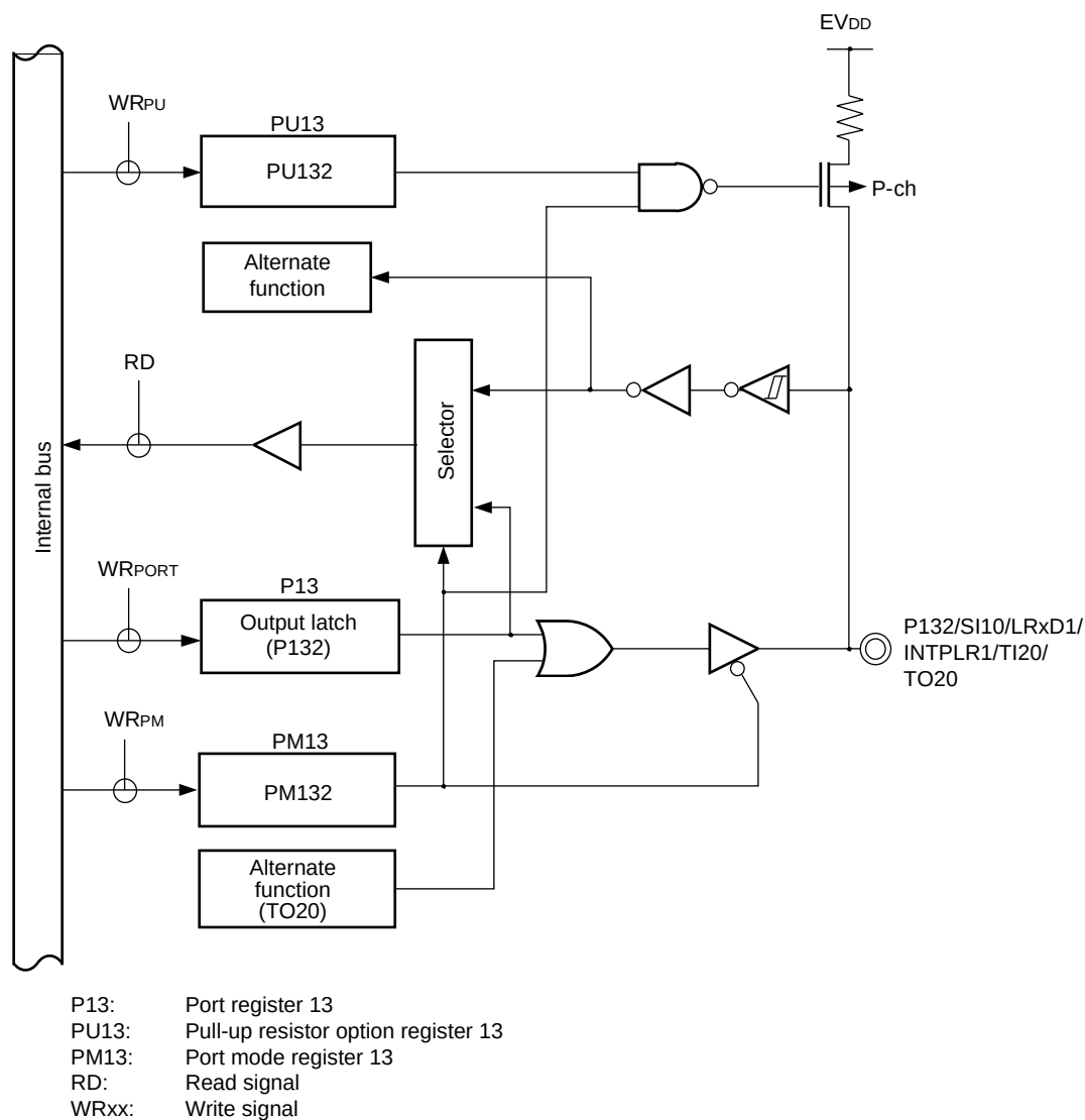
Figure 4-50. Block Diagram of P132
