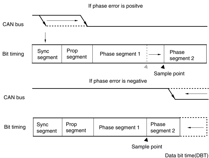
Figure 14-21. Resynchronization
