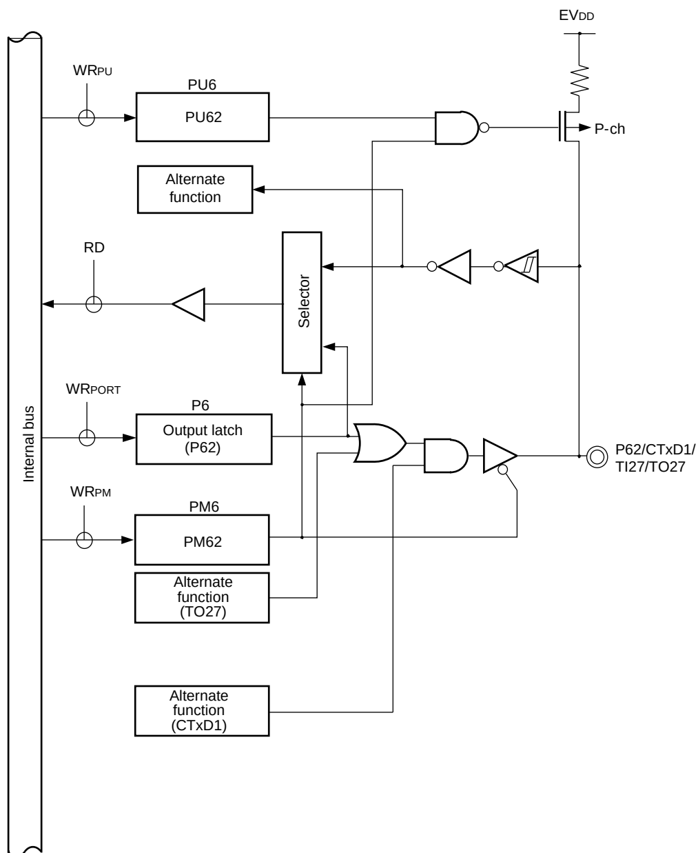
Figure 4-27. Block Diagram of P62
