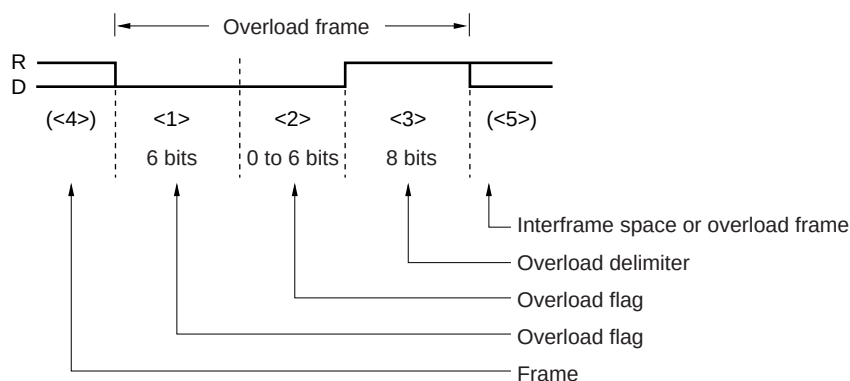
Figure 14-16. Overload Frame
