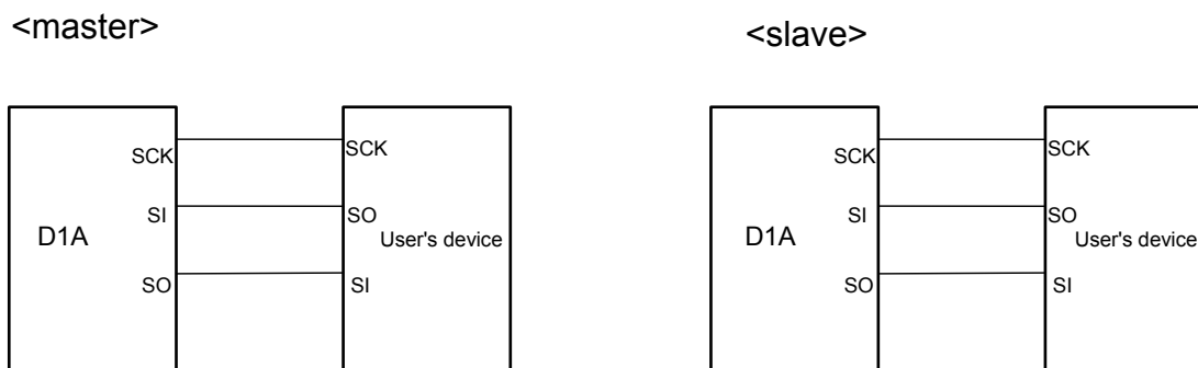
Figure 34-6. CSI mode connection diagram
