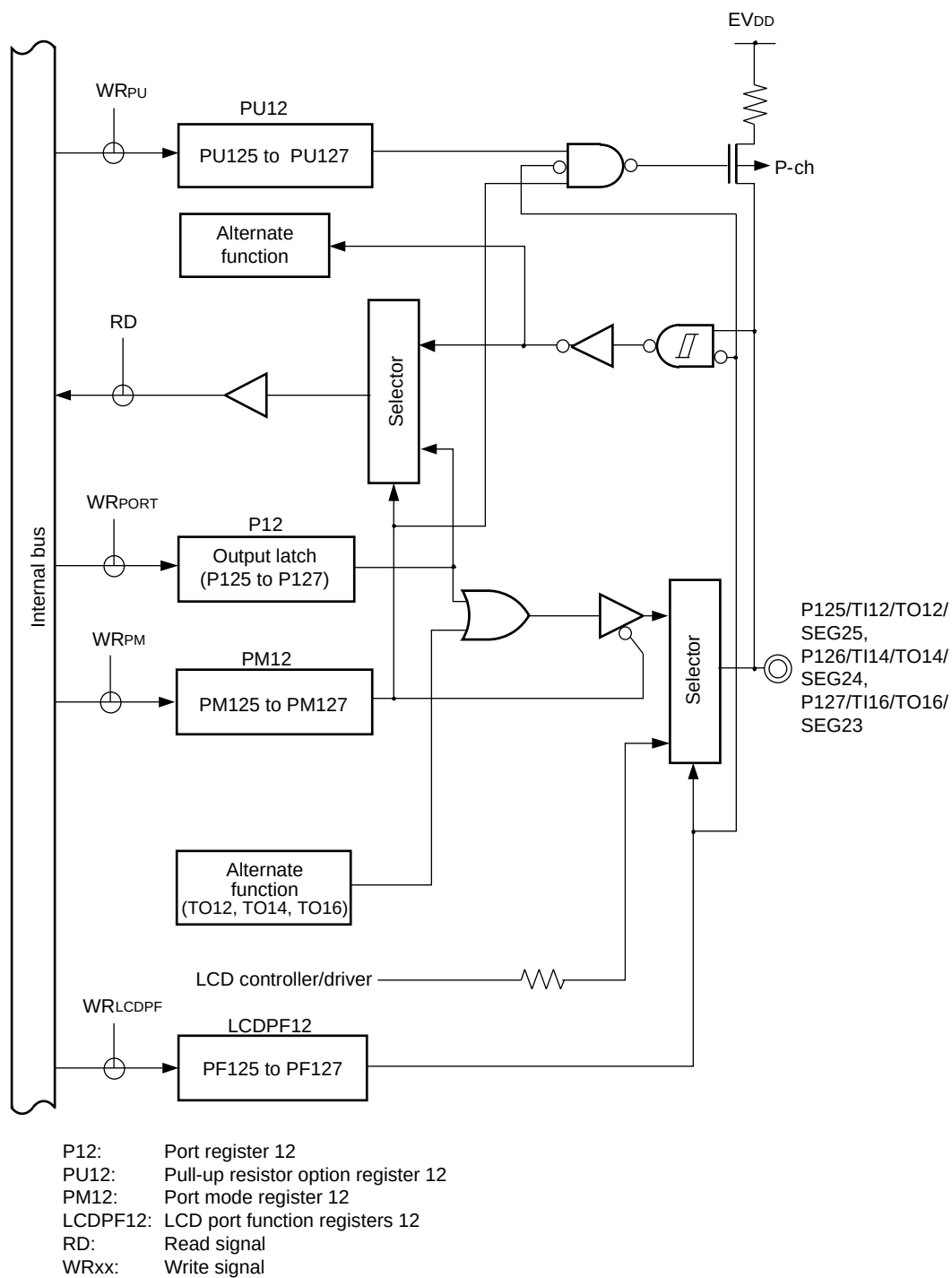
Figure 4-47. Block Diagram of P125 to P127
