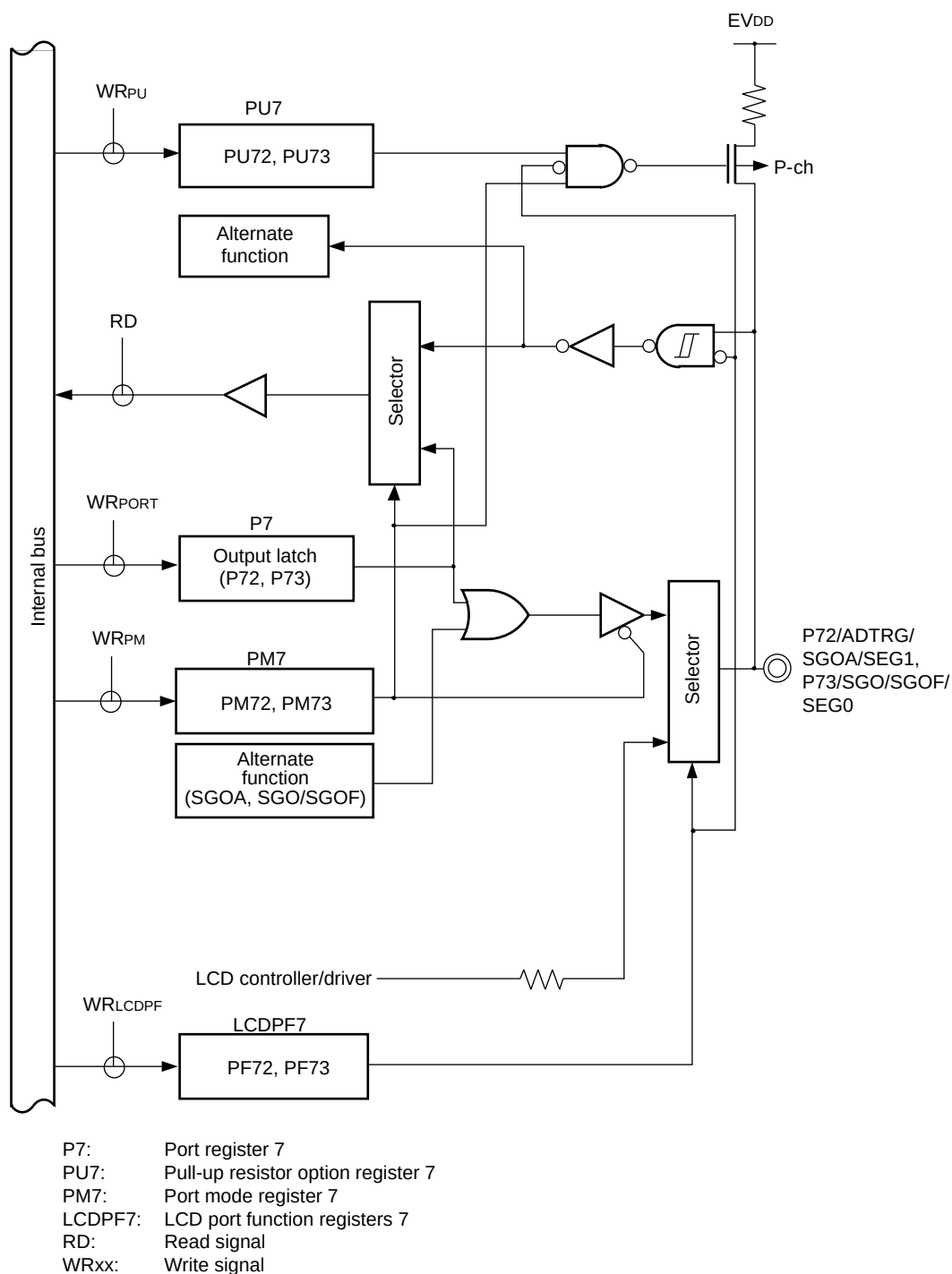
Figure 4-33. Block Diagram of P72, P73
