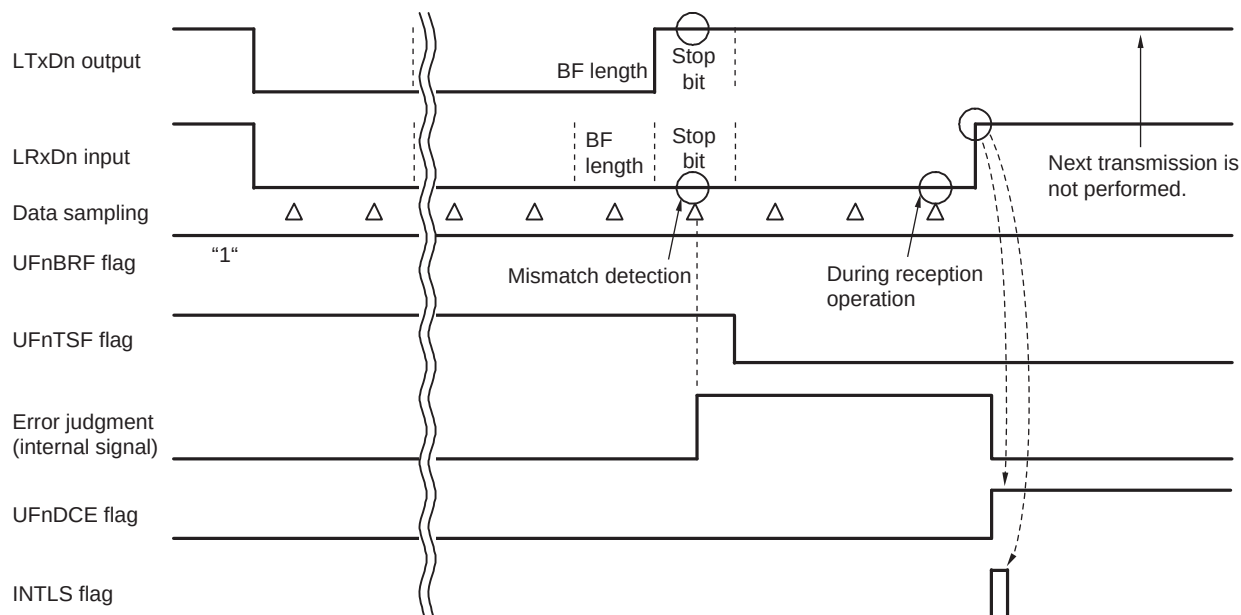
Figure 13-47. Example of Consistency Error Occurrence Timing During BF Transmission When UFnBRF = 1 (If During Reception Operation When Input Data “1” Is Detected After Stop Bit (Previous Bit Is “0”))
