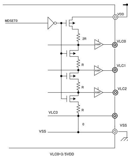
(b) 1/3 bias method and static display mode (MDSET1, MDSET0 = 1, 1) (example of V_{DD} = 5\text{ V} , V_{LC0} = 3\text{ V} )
