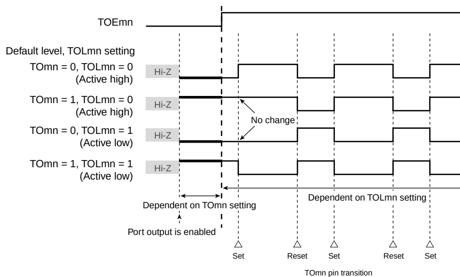
Figure 6-43. TOMmn Pin Output Status at PWM Output (TOMmn = 1)
