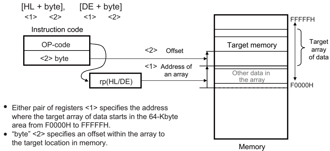
Figure 3-40. Example of [HL + byte], [DE + byte]
