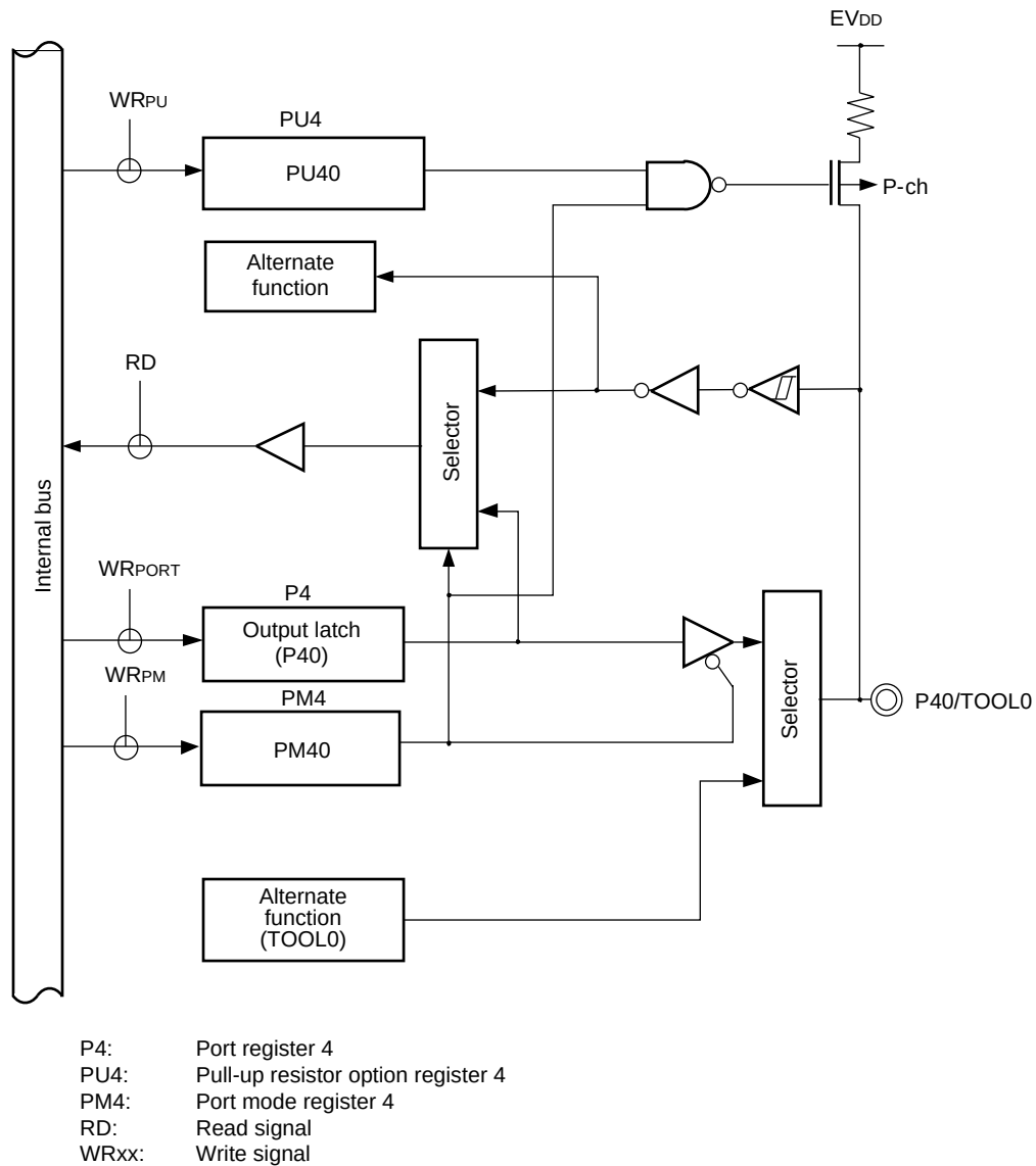
Figure 4-17. Block Diagram of P40
