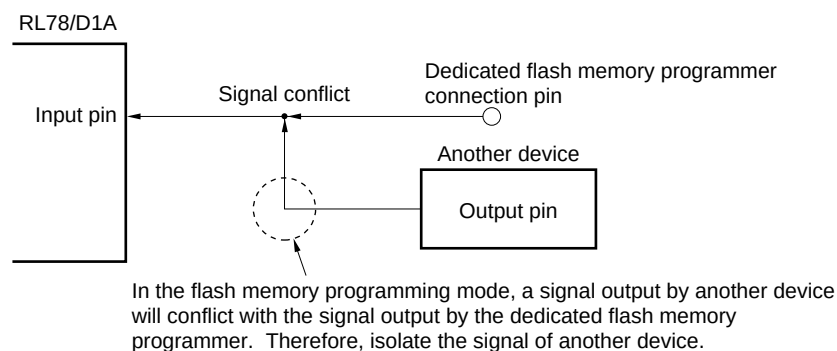
Figure 29-5. Signal Conflict ( \overline{\text{RESET}} Pin)
