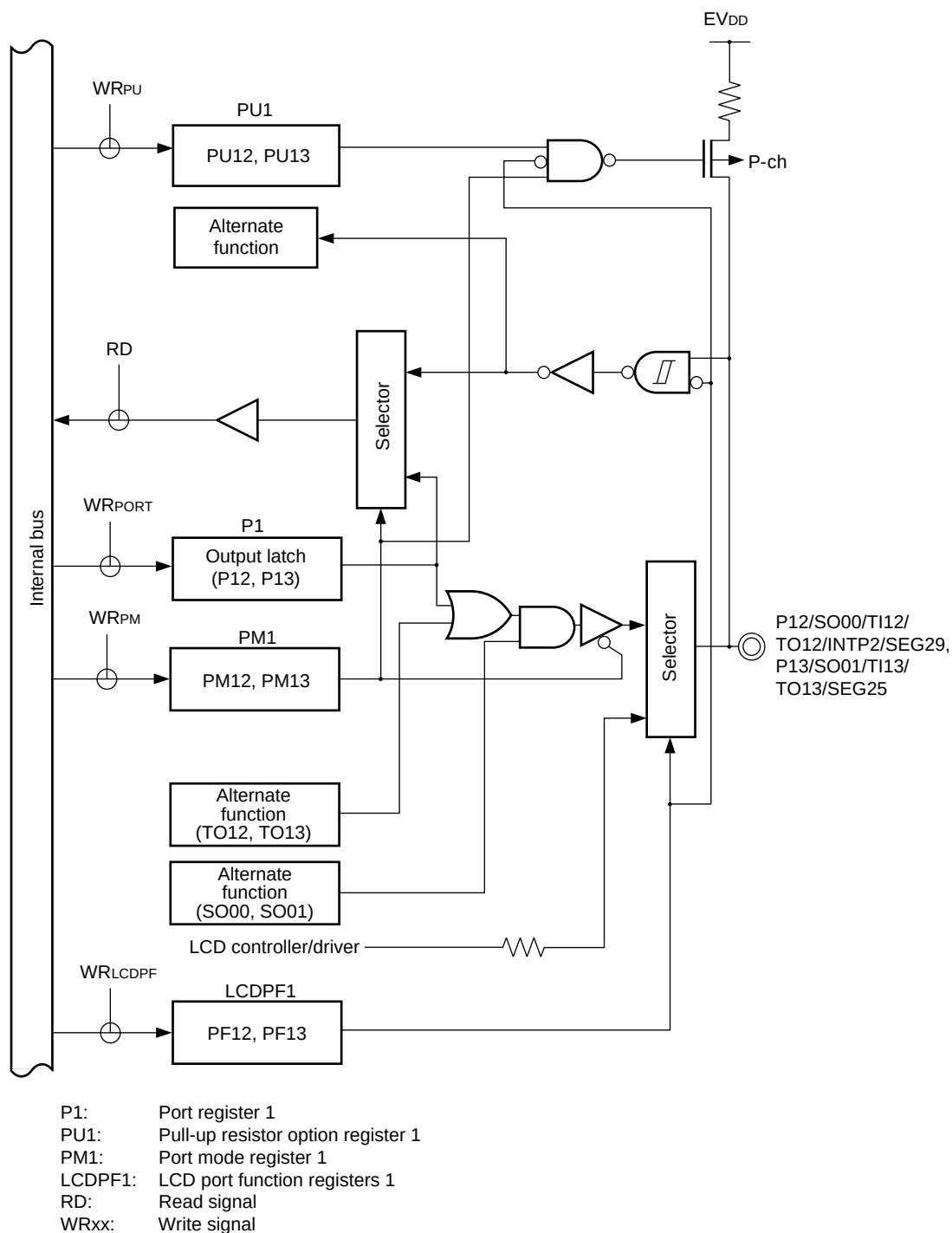
Figure 4-9. Block Diagram of P12, P13
