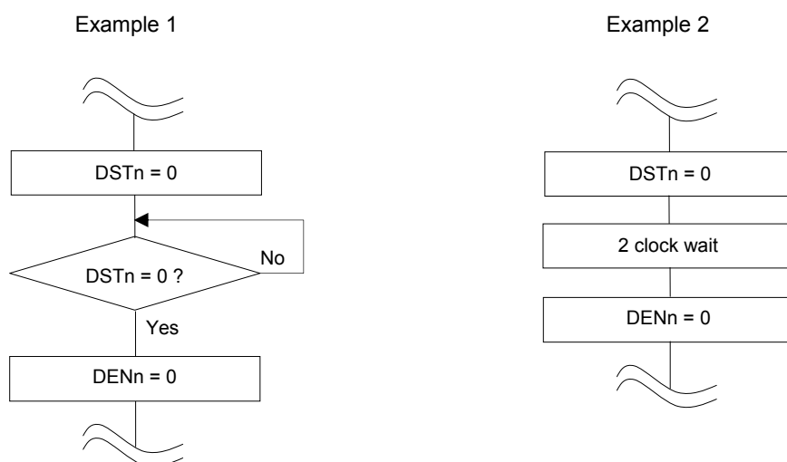
Figure 20-12. Forced Termination of DMA Transfer (1/2)
