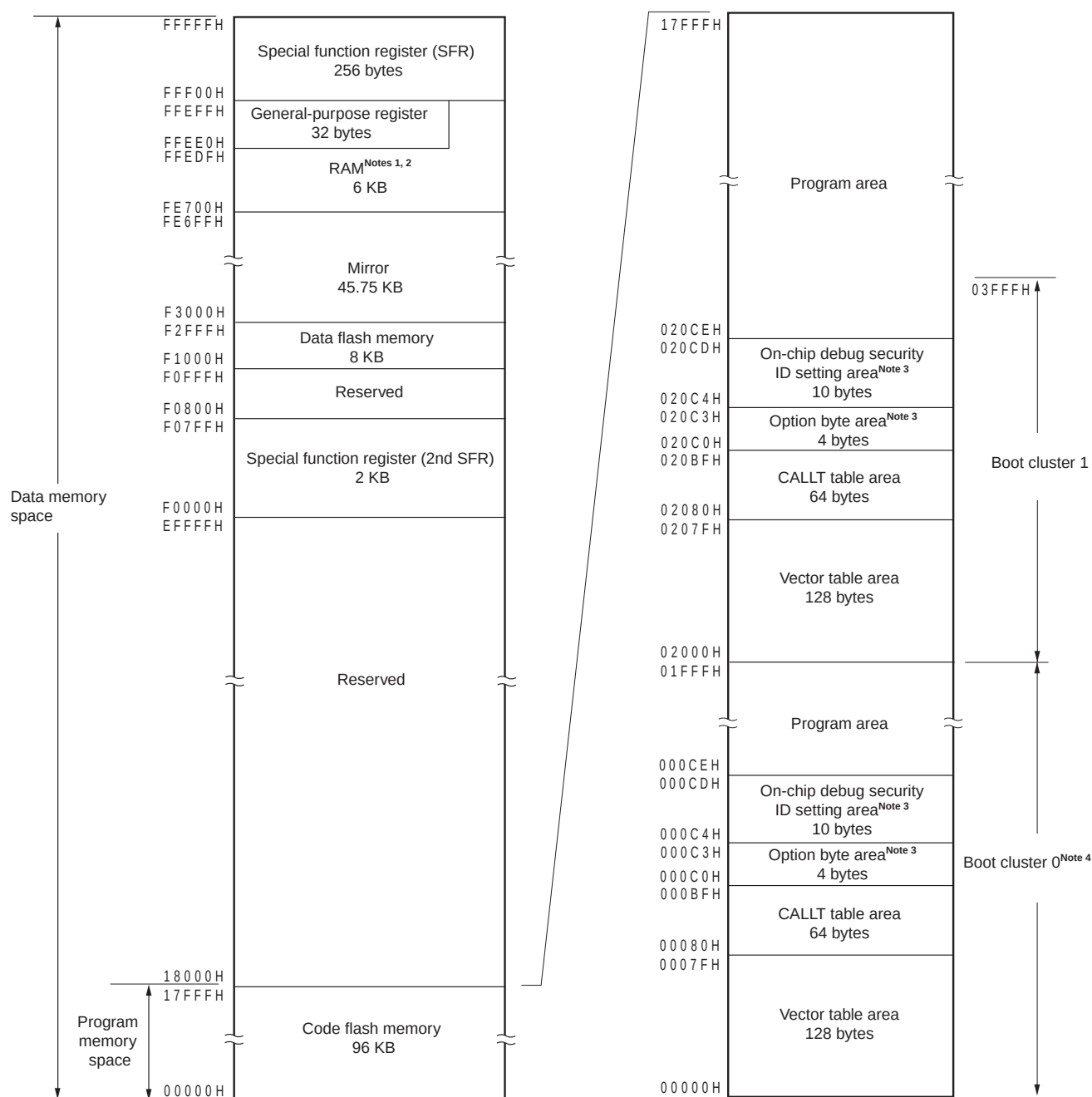
Figure 3-5. Memory Map (R5F10DMFxFB, R5F10DPFB)
