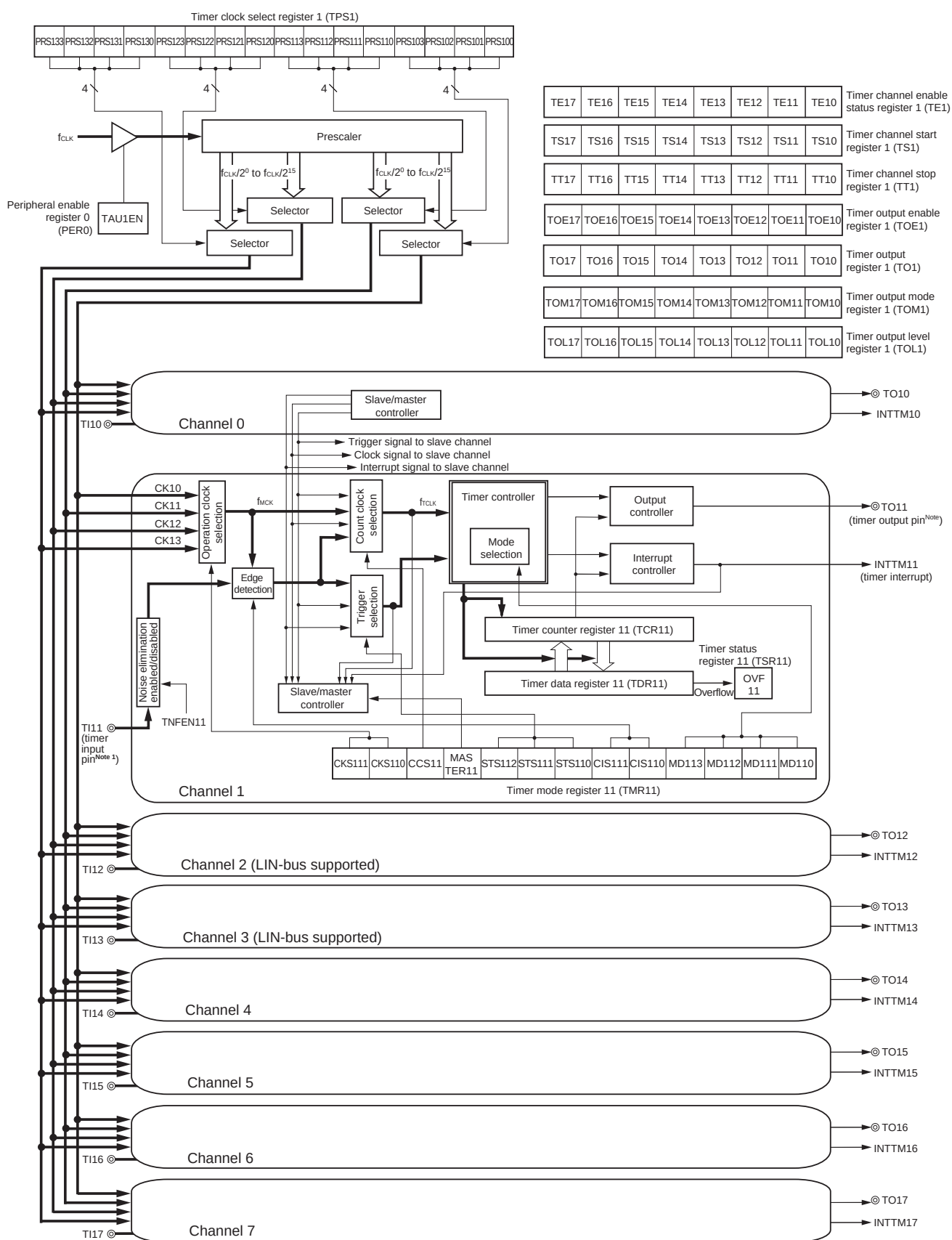
Figure 6-3. Block Diagram of Timer Array Unit 1
