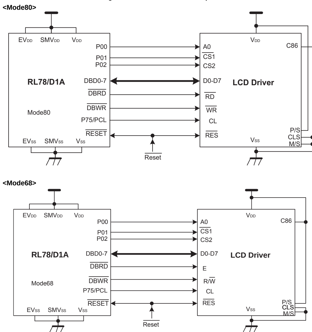
Figure 17-15. Connection example 1
