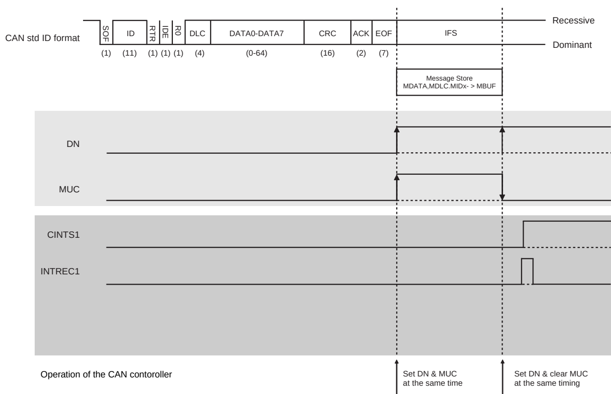
Figure 14-55. DN and MUC Bit Setting Period (for Standard ID Format)
