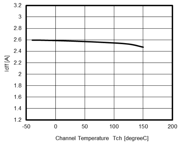
Double frequency flashing threshold VS. Channel TEMPERATURE
