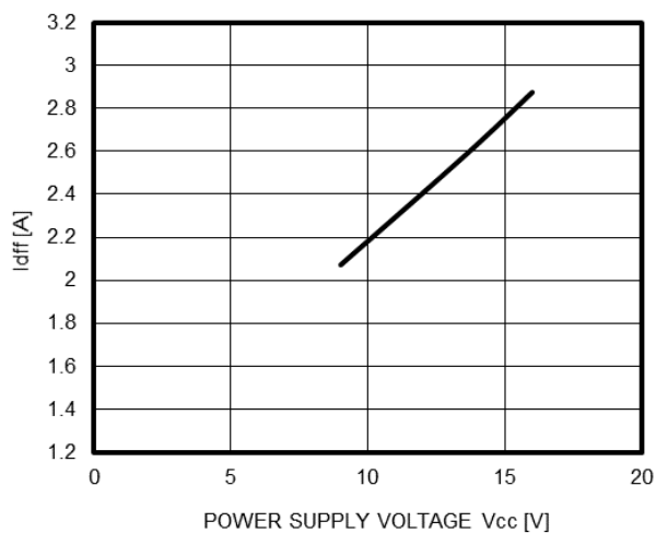
Double frequency flashing threshold VS. POWER SUPPLY VOLTAGE
