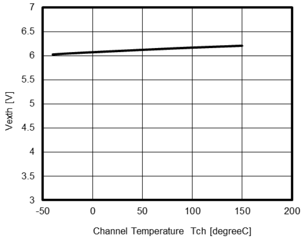
Internal clock high level between EXT and OUT VS. Channel TEMPERATURE
