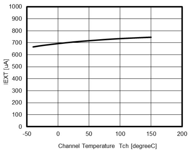
Supply current via EXT pin VS. Channel TEMPERATURE
