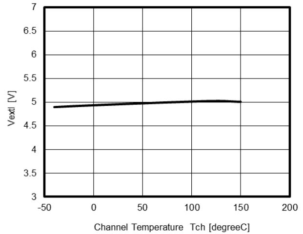
Internal clock low level between EXT and OUT VS. Channel TEMPERATURE
