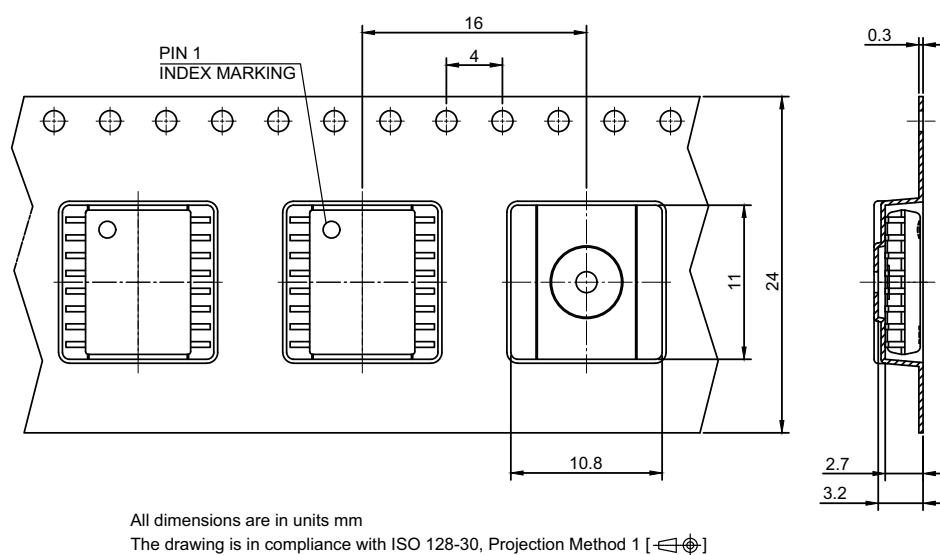
Figure 20 PG-DSO-16-30 packaging
