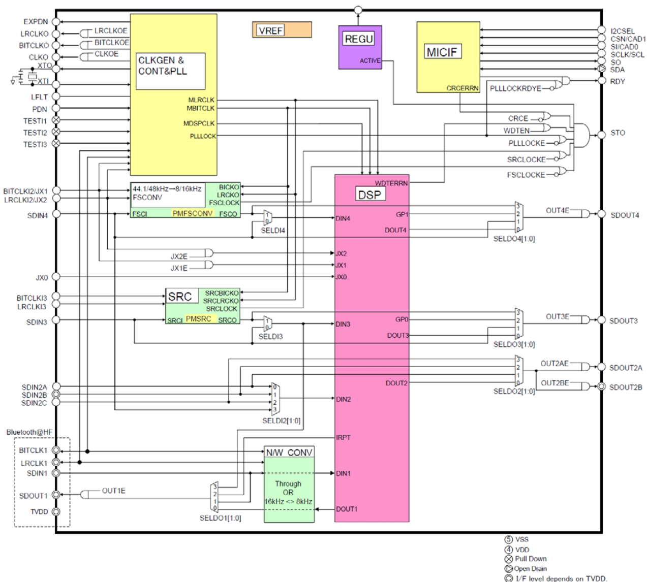
Figure 1. Block Diagram
