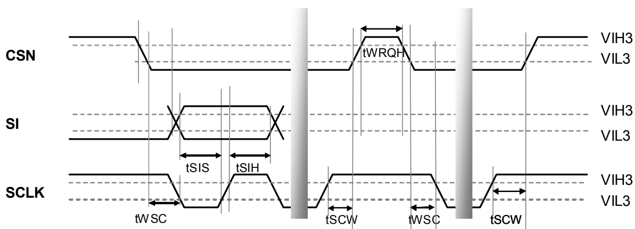
Figure 10. Microprocessor → AK7736A
