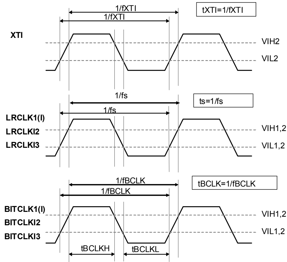
Figure 3. System Clock
