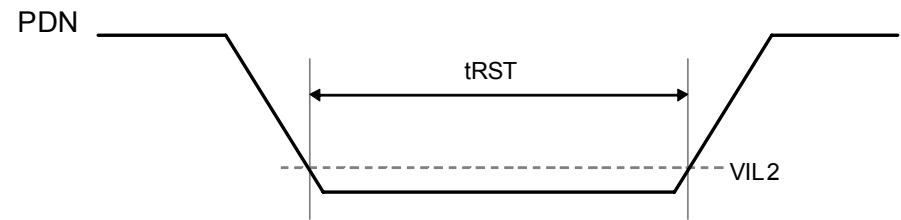
Figure 4. Power-down
