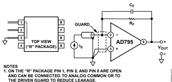
Figure 34. Guarding Scheme—Inverter
