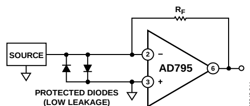
Figure 44. Input Voltage Clamp with Diodes
