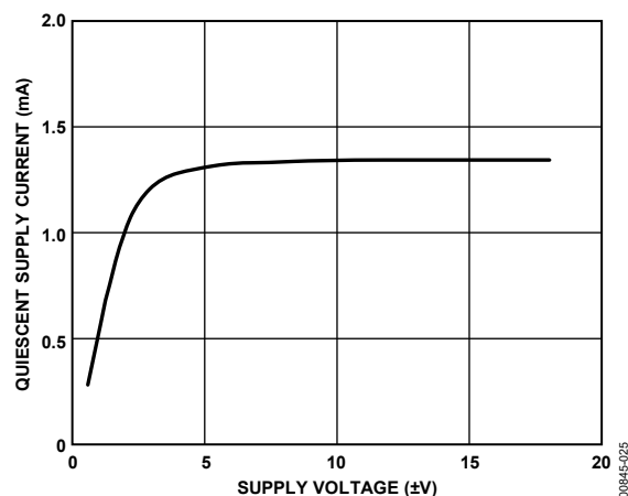
Figure 25. Quiescent Supply Current vs. Supply Voltage
