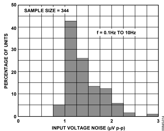
Figure 14. Typical Distribution of Input Voltage Noise
