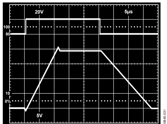
Figure 31. Unity Gain Follower Large Signal Pulse Response
