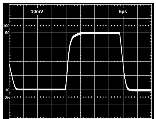
Figure 40. Inverter Pulse Response with 1 M \Omega Source and Feedback Resistance, 1 pF Feedback Capacitance
