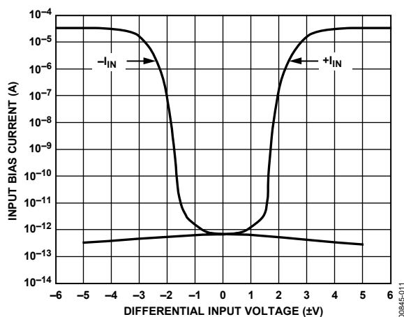
Figure 11. Input Bias Current vs. Differential Input Voltage
