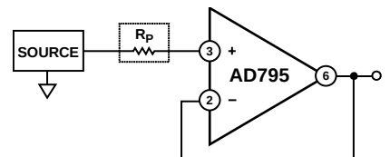
Figure 43. Follower with Input Current Limit
