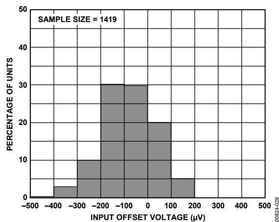
Figure 26. Typical Distribution of Input Offset Voltage
