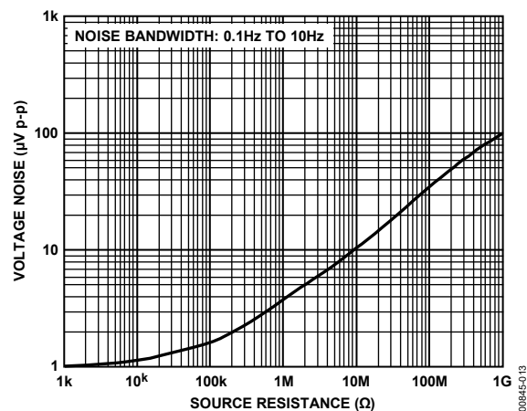
Figure 13. Input Voltage Noise vs. Source Resistance
