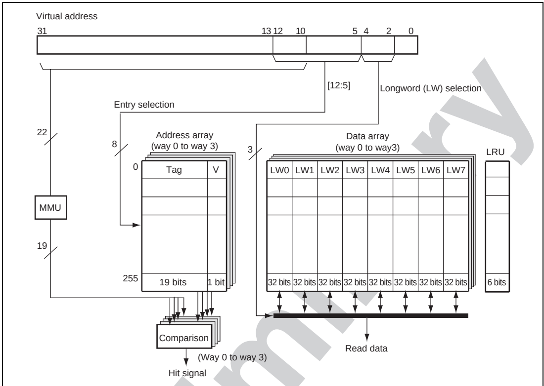
Figure 4.2 Configuration of Instruction Cache (IC)
