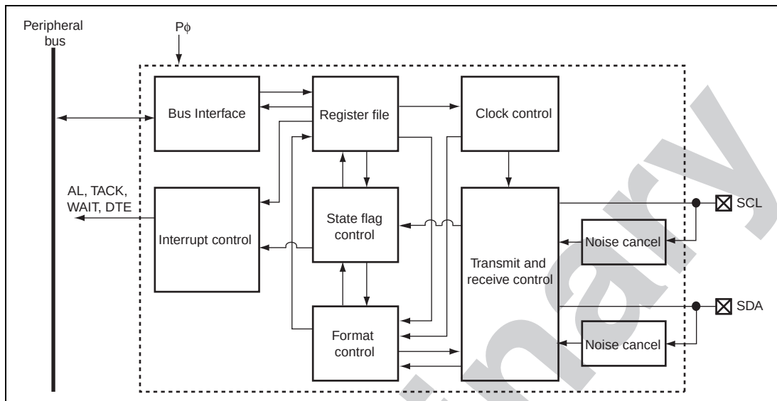
Figure 21.1 Block Diagram of I 2 C Bus Interface
