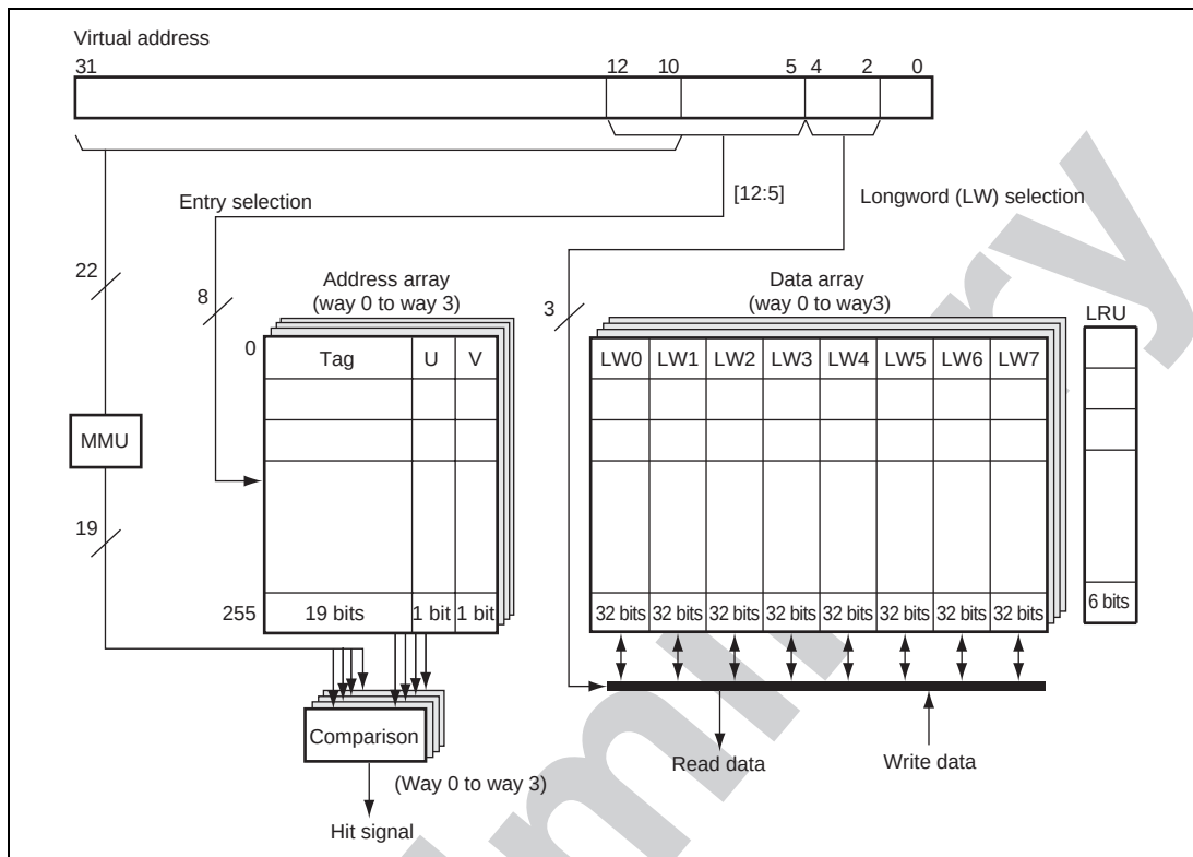
Figure 4.1 Configuration of Operand Cache (OC)
