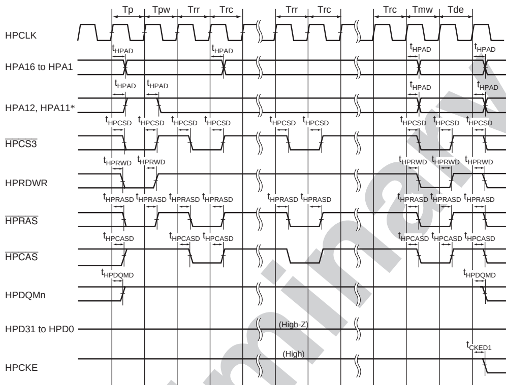
Figure 38.40 Power-On Sequence of SDRAM (Mode Write Timing, TRP = 2 Cycles)
