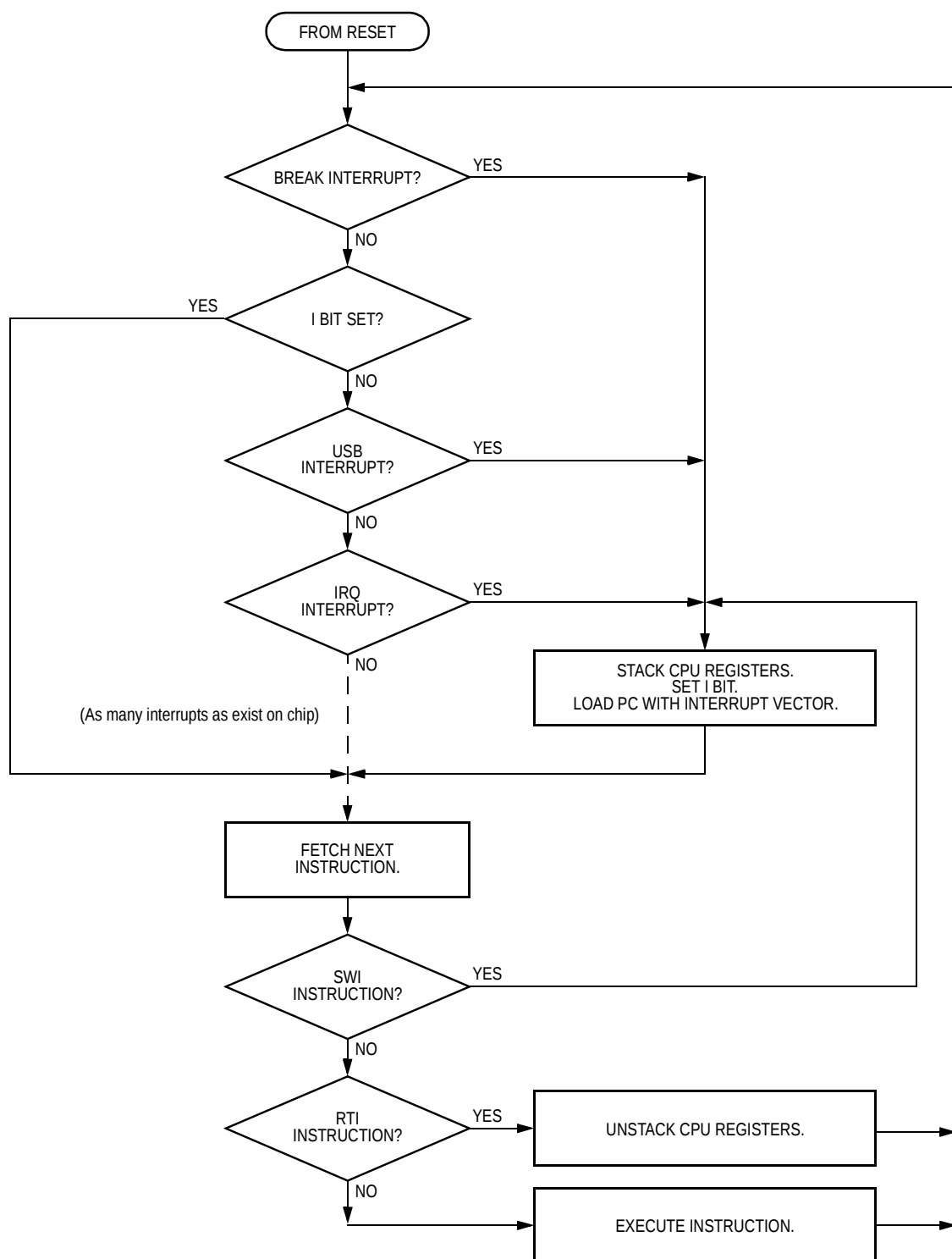
Figure 8-8. Interrupt Processing
