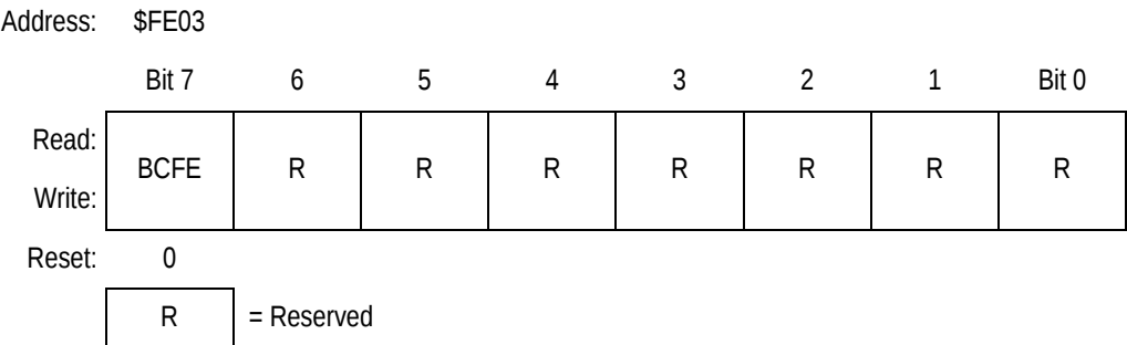
Figure 19-7. SIM Break Flag Control Register (SBFCR)
