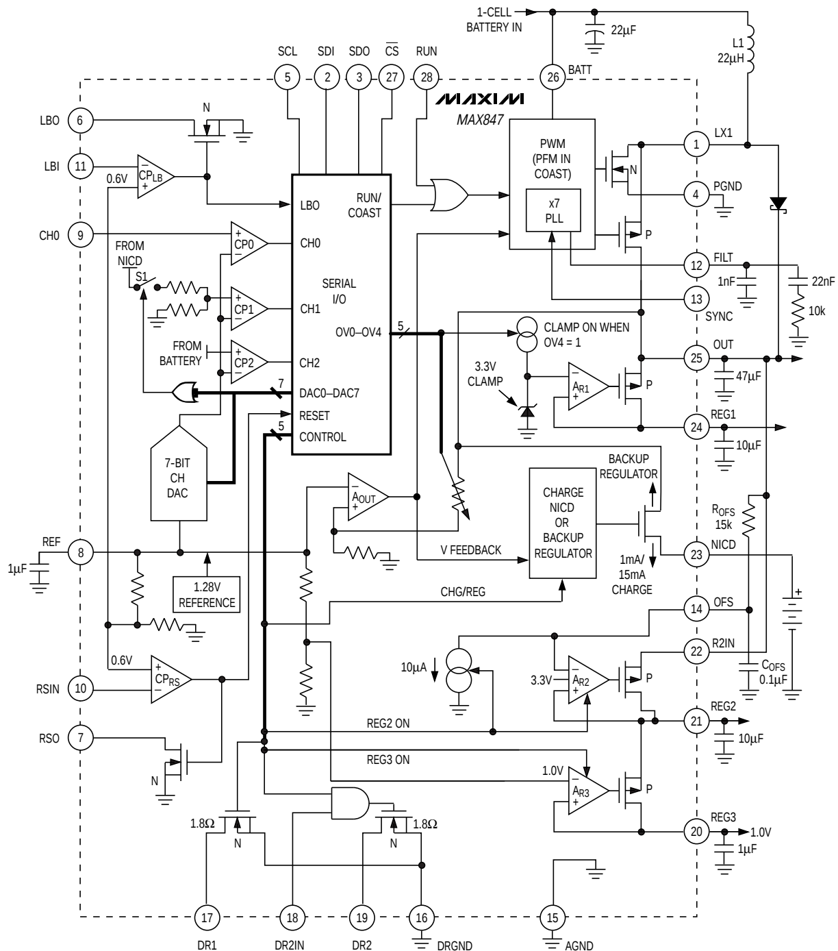
Figure 1. Functional Diagram
