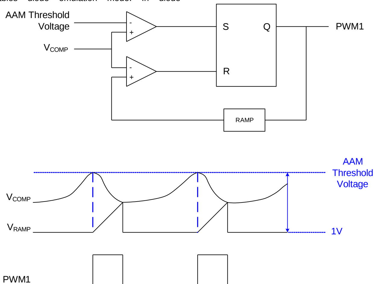
Figure 2: Block Diagram of AAM Operation and Typical Waveforms
