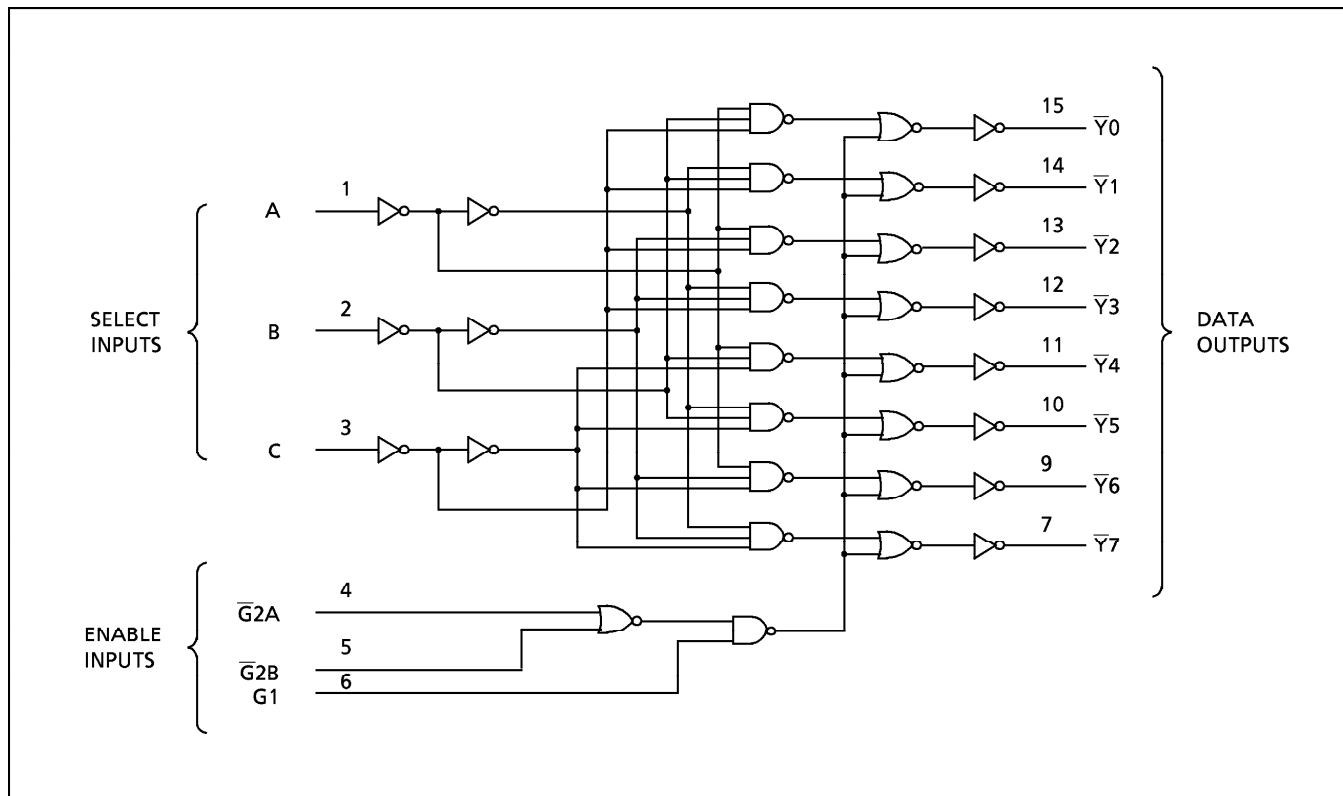
LOGIC DIAGRAM
