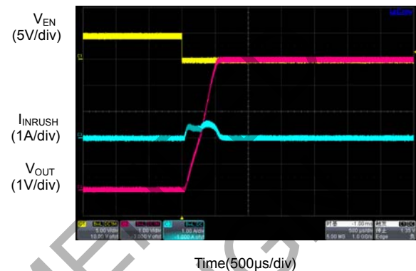
Figure 21. Output Turn ON and Rise Time ( C_{IN}=1.0\mu F, C_{OUT}=47\mu F, \text{No Load} )
