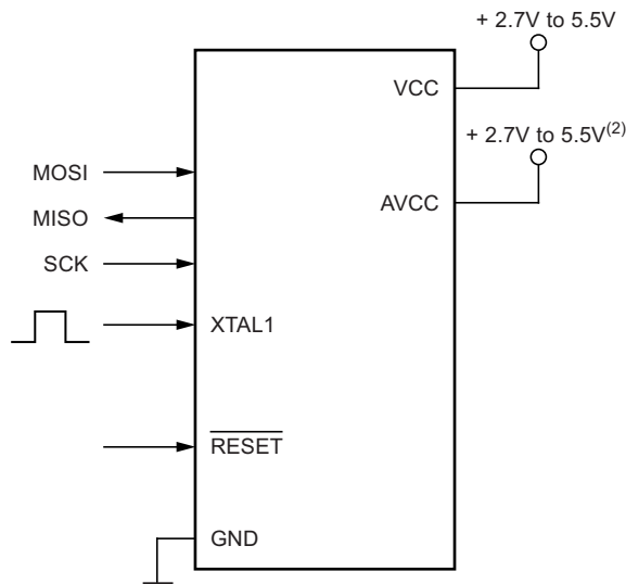
Figure 24-10. Serial Programming and Verify (1)
