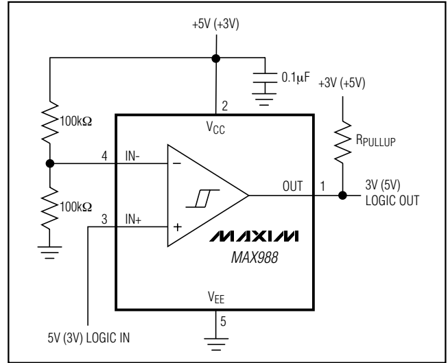
Figure 4. Logic-Level Translator
