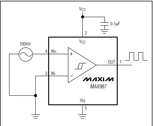
Figure 3. Zero-Crossing Detector
