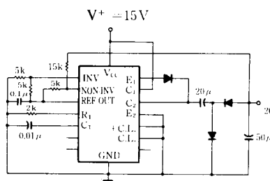
Fig. 1 Capacitor-Diode Output Circuit
