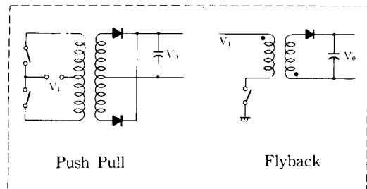
Transformer-Coupled Outputs
