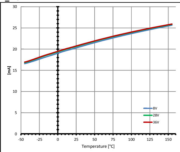
Sense Signal Maximum Current in Fault Condition
