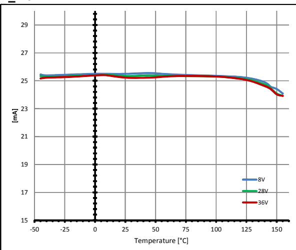
Open Load Detection ON State Threshold
