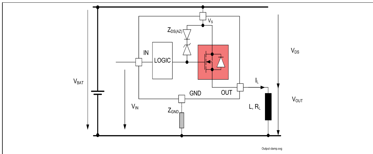
Figure 10 Output Clamp
