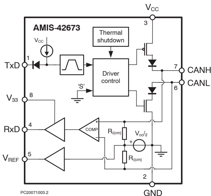
Figure 1. Block Diagram
