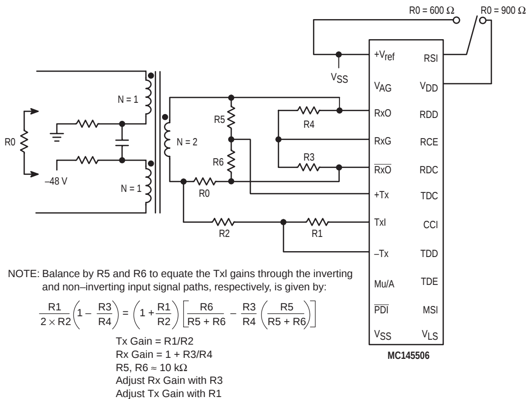
(a) Universal Transformer Hybrid Using MC145506
